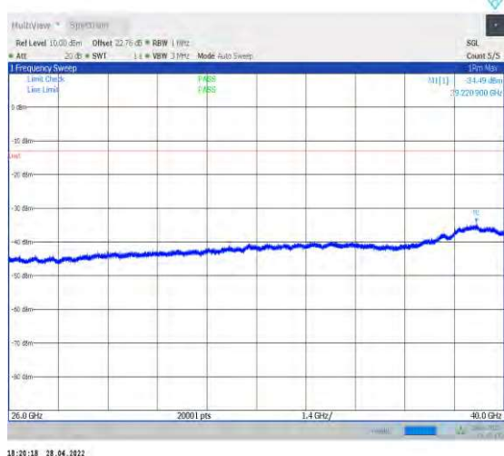
1-N77-3700-3980--30-100-L-1-DFT-QPSK-Edge_1R B_Left-1@0-26000-40000-Ant1--34.49--13-PASS
