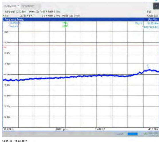
1-N77-3700-3980--30-100-L-1-DFT-QPSK-Edge_1R B_Left-1@0-26000-40000-Ant2--34.85--13-PASS
