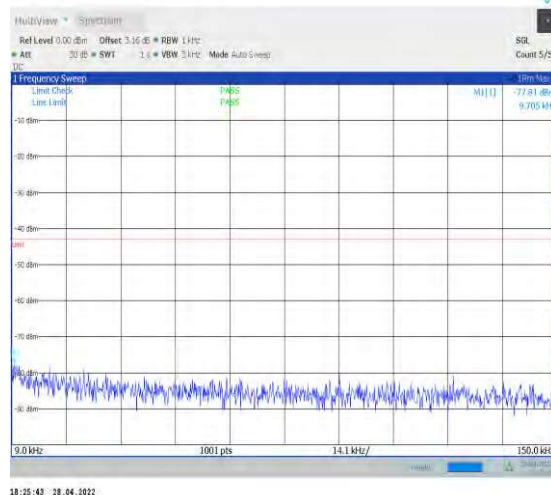
1-N77-3700-3980--30-100-M-1-DFT-QPSK-Edge_1R B_Left-1@0-0.009-0.15-Ant2--77.81--43-PASS
