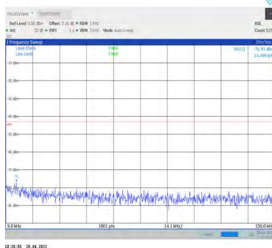
1-N77-3700-3980--30-100-M-1-DFT-QPSK-Edge_1R B_Left-1@0-0.009-0.15-Ant1--76.91--43-PASS
