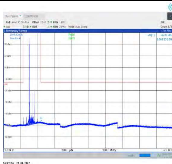
1-N77-3450-3550--30-100-M-1-DFT-QPSK-Edge_1R B_Left-1@0-3000-6000-Ant2--46.92--13-PASS
