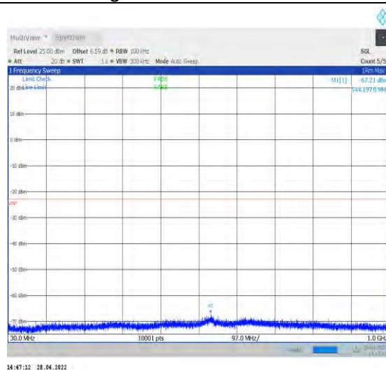
1-N77-3450-3550--30-100-M-1-DFT-QPSK-Edge_1R B_Left-1@0-30-1000-Ant2--67.21--23-PASS
