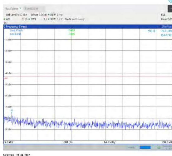
1-N77-3450-3550--30-100-M-1-DFT-QPSK-Edge_1R B_Left-1@0-0.009-0.15-Ant1--76.51--43-PASS
