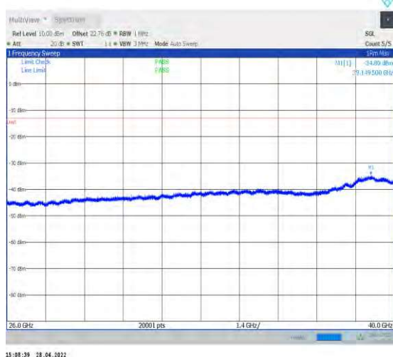
1-N77-3450-3550--30-100-L-1-DFT-QPSK-Edge_1R B_Left-1@0-26000-40000-Ant1--34.80--13-PASS
