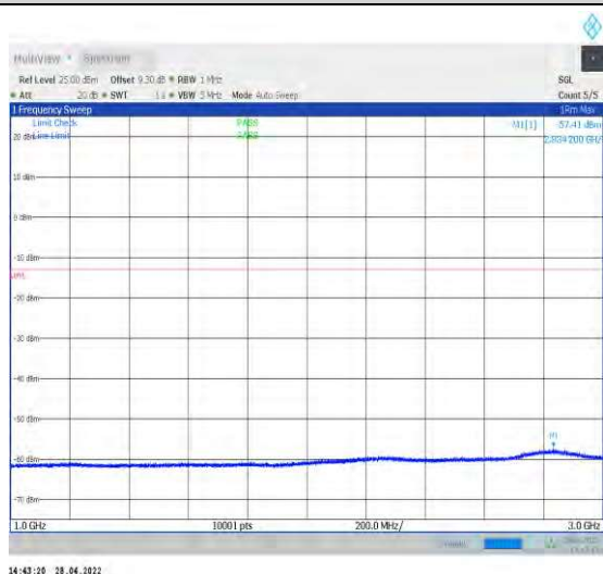
1-N77-3450-3550--30-100-M-1-DFT-QPSK-Edge_1R B_Left-1@0-1000-3000-Ant1--57.41--13-PASS
