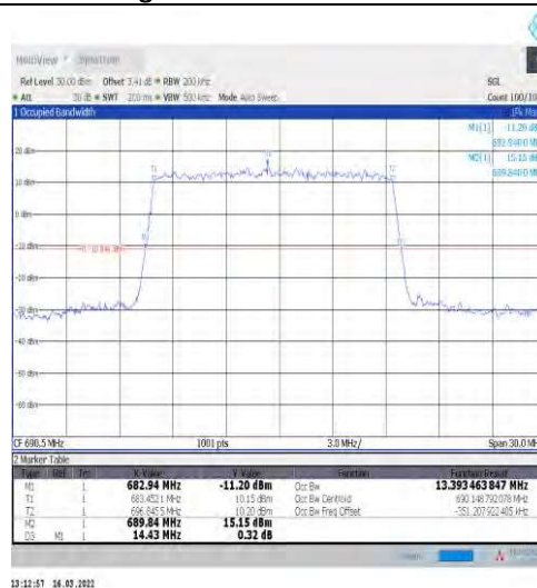
1-N71-15-15-H-2-DFT-PI2BPSK-Outer_Full-75@0-Ant1 -13.393-14.430≤15-PASS
