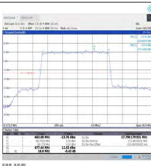
1-N71-15-20-L-4-DFT-64QAM-Outer_Full-100@0-An t1-17.79-18.800-<=20-PASS
