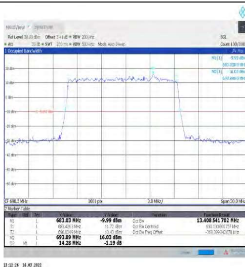
1-N71-15-15-H-1-DFT-QPSK-Outer_Full-75@0-Ant1 -13.409-14.280≤15-PASS
