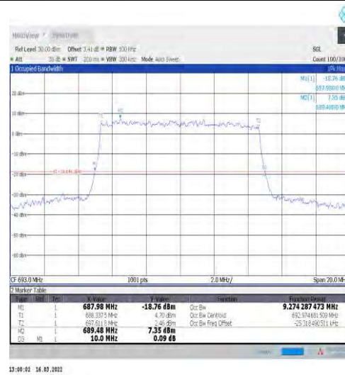
1-N71-15-10-H-9-CP-256QAM-Outer_Full-52@0-Ant 1-9.274-10.000≤10-PASS
