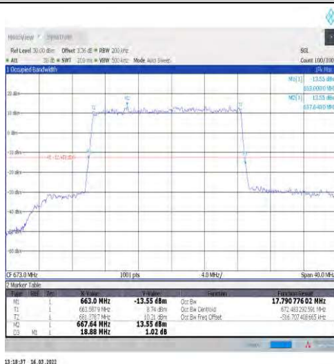
1-N71-15-20-L-2-DFT-PI2BPSK-Outer_Full-100@0- Ant1-17.791-18.880≤20-PASS
