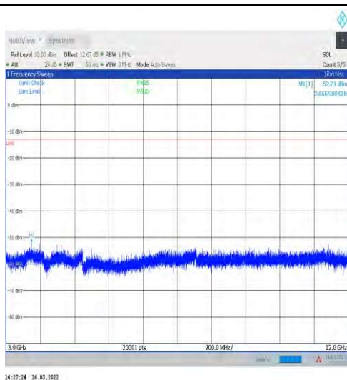
1-N71-15-20-L-1-DFT-PI2BPSK-Inner_1RB_Left-1@ 1-3000-12000-Ant1--52.21--13-PASS
