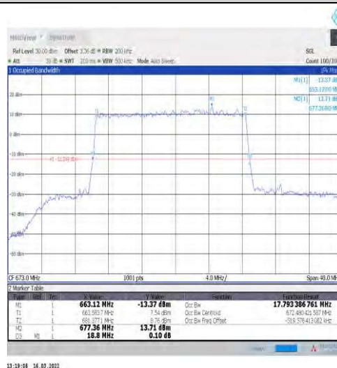
1-N71-15-20-L-3-DFT-16QAM-Outer_Full-100@0-An t1-17.793-18.800≤20-PASS
