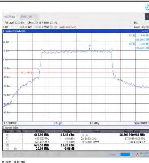
1-N71-15-20-L-6-CP-QPSK-Outer_Full-106@0-Ant1 -18.805-20.040-<=20-PASS
