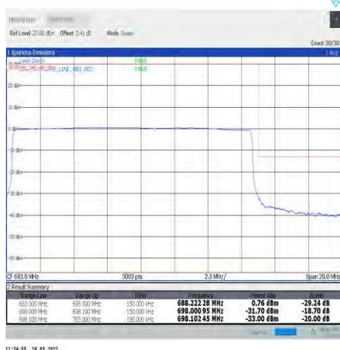
1-N71-15-15-H-6-CP-QPSK-Outer_Full-79@0-Ant1-PASS-see graph
