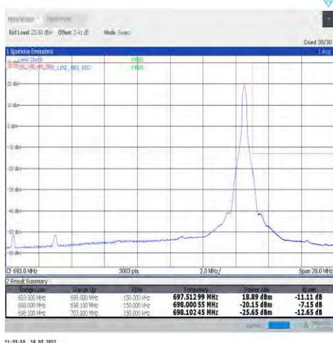
1-N71-15-15-H-5-CP-QPSK-Edge_1RB_Right-1@78-Ant1-PASS-see graph
