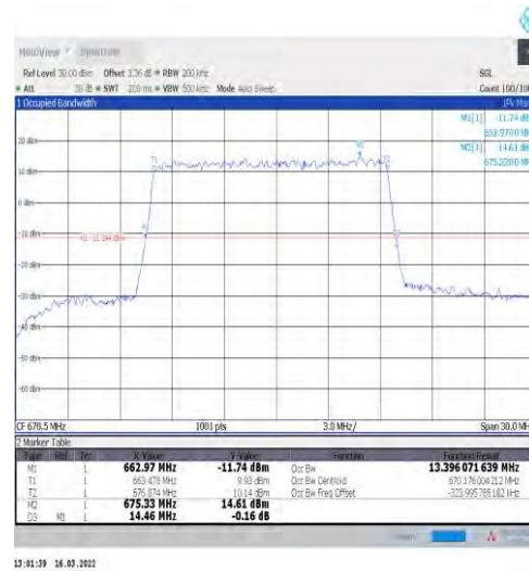
1-N71-15-15-L-2-DFT-PI2BPSK-Outer_Full-75@0-Ant1- 13.396-14.460≤15-PASS
