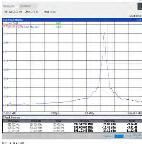
1-N71-15-15-H-2-DFT-PI2BPSK-Edge_1RB_Right-1@78-Ant1-PASS-see graph
