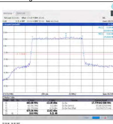
1-N71-15-20-L-1-DFT-QPSK-Outer_Full-100@0-Ant 1-17.78-18.800≤20-PASS
