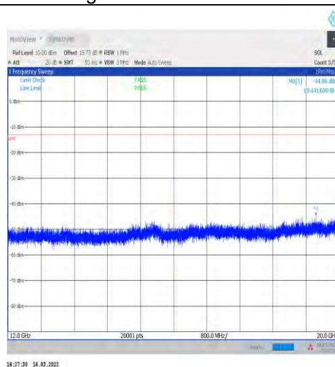
1-N71-15-20-L-1-DFT-PI2BPSK-Inner_1RB_Left-1@ 1-12000-20000-Ant1--44.86--13-PASS
