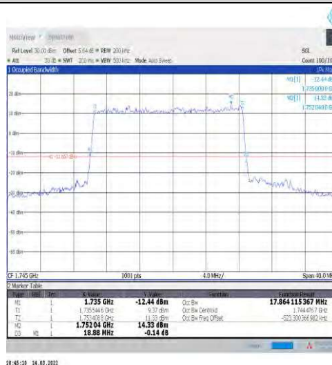
1-N66-15-20-M-2-DFT-PI2BPSK-Outer_Full-100@0-Ant Ant1-17.864-18.880-≤20-PASS
