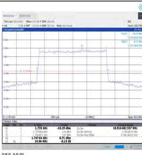
1-N66-15-20-M-9-CP-256QAM-Outer_Full-106@0-Ant 1-18.917-19.960-≤20-PASS
