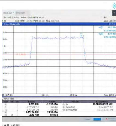
1-N66-15-20-M-1-DFT-QPSK-Outer_Full-100@0-Ant 1-17.88-18.920-≤20-PASS
