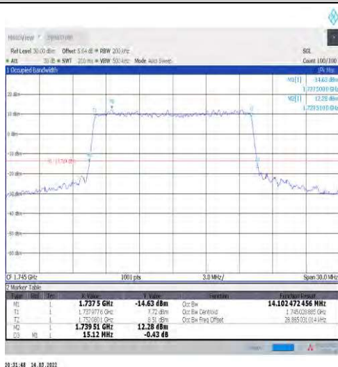
1-N66-15-15-M-8-CP-64QAM-Outer_Full-79@0-Ant1-14.102-15.120-≤15-PASS
