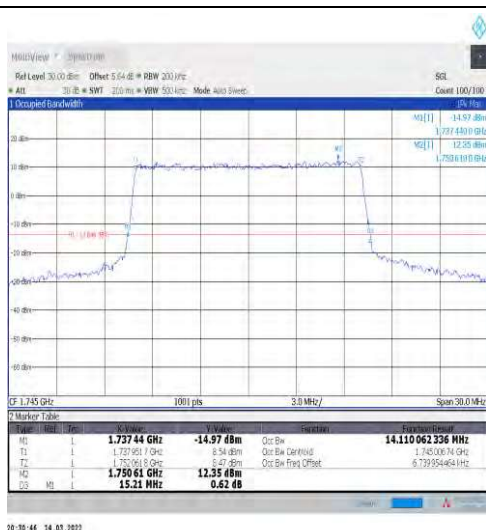
1-N66-15-15-M-6-CP-QPSK-Outer_Full-79@0-Ant1-14.11-15.210-≤15-PASS
