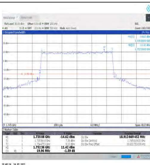
1-N66-15-20-M-7-CP-16QAM-Outer_Full-106@0-Ant 1-18.914-19.960-≤20-PASS
