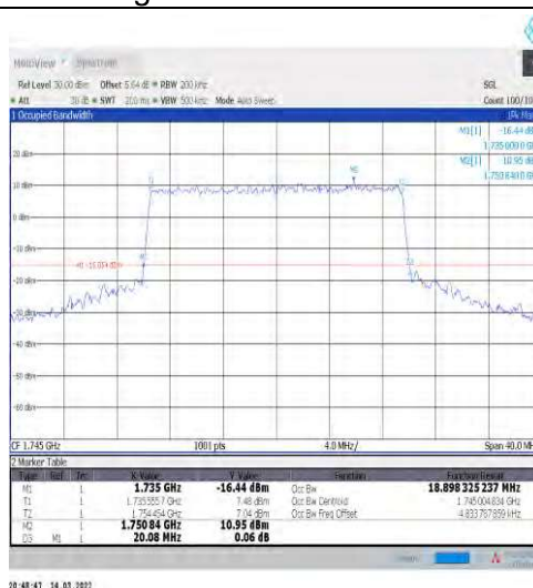
1-N66-15-20-M-8-CP-64QAM-Outer_Full-106@0-Ant 1-18.898-20.080-≤20-PASS
