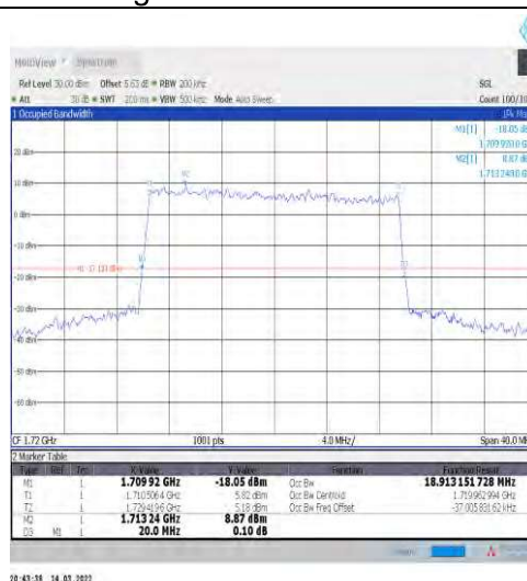
1-N66-15-20-L-9-CP-256QAM-Outer_Full-106@0-Ant t1-18.913-20.000-≤20-PASS
