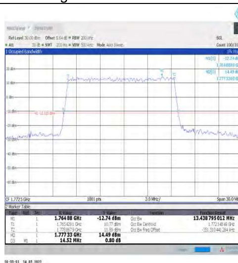
1-N66-15-15-H-2-DFT-PI2BPSK-Outer_Full-75@0-Ant1 -13.439-14.520≤15-PASS
