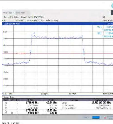
1-N66-15-20-H-1-DFT-QPSK-Outer_Full-100@0-Ant 1-17.912-19.040-≤20-PASS
