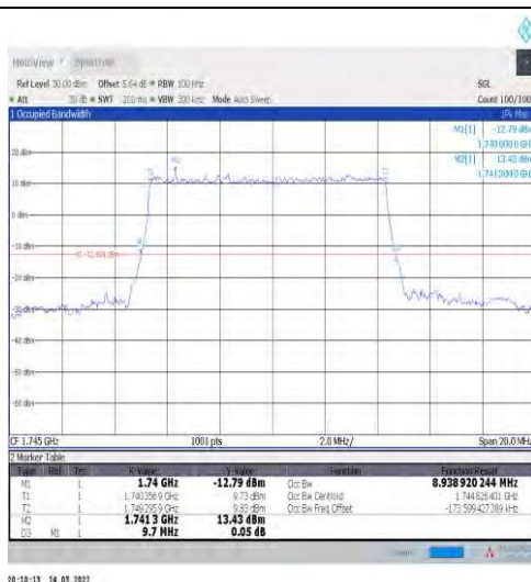
1-N66-15-10-M-1-DFT-QPSK-Outer_Full-50@0-Ant1 -8.939-9.700-≤10-PASS
