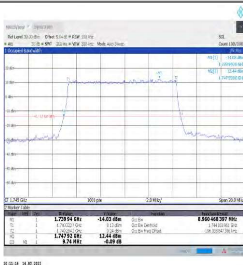
1-N66-15-10-M-3-DFT-16QAM-Outer_Full-50@0-Ant1 1-8.96-9.740-≤10-PASS
