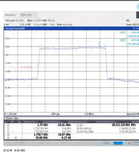
1-N66-15-30-M-5-DFT-256QAM-Outer_Full-160@0-Ant1-28.511-29.880-≤30-PASS
