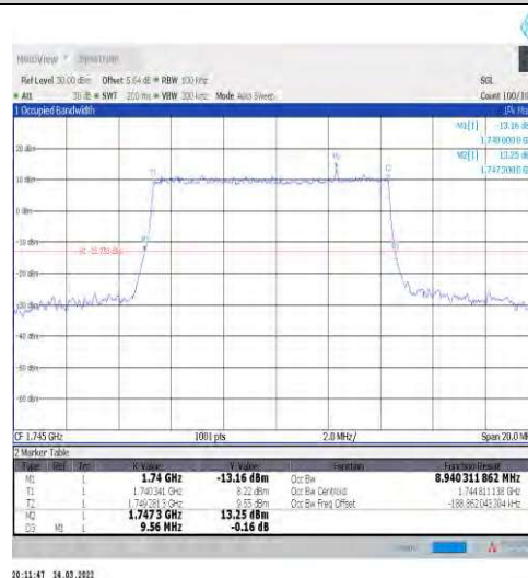
1-N66-15-10-M-4-DFT-64QAM-Outer_Full-50@0-Ant1 1-8.94-9.560-≤10-PASS
