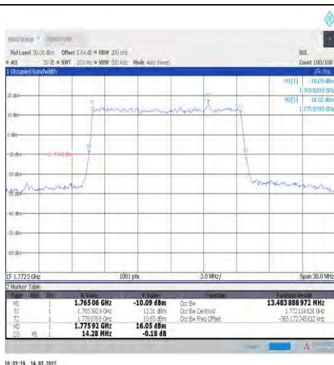
1-N66-15-15-H-1-DFT-QPSK-Outer_Full-75@0-Ant1 -13.484-14.280≤15-PASS
