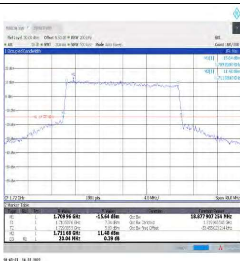
1-N66-15-20-L-8-CP-64QAM-Outer_Full-106@0-Ant 1-18.878-20.040-≤20-PASS
