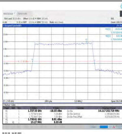
1-N66-15-15-M-9-CP-256QAM-Outer_Full-79@0-Ant1-14.117-15.270-≤15-PASS
