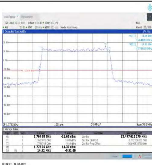
1-N66-15-15-H-3-DFT-16QAM-Outer_Full-75@0-Ant1 1-13.478-14.520≤15-PASS
