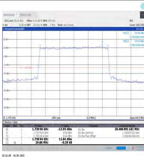
1-N66-15-30-M-6-CP-QPSK-Outer_Full-160@0-Ant1-28.487-29.880-≤30-PASS
