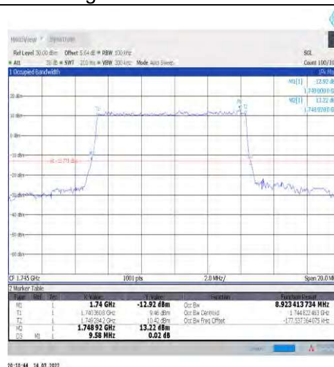
1-N66-15-10-M-2-DFT-PI2BPSK-Outer_Full-50@0-Ant1 -8.923-9.580-≤10-PASS
