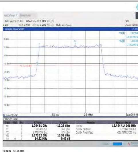
1-N66-15-15-H-4-DFT-64QAM-Outer_Full-75@0-Ant1 1-13.454-14.520≤15-PASS
