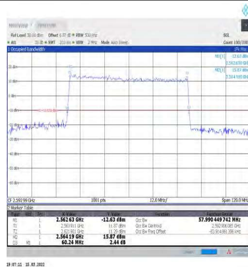
1-N41-30-60-M-3-DFT-16QAM-Outer_Full-162@0-Ant1-57.99-60.240-≤60-PASS
