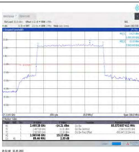
1-N41-30-90-L-4-DFT-64QAM-Outer_Full-240@0-An t1-85.574-89.460-≤90-PASS
