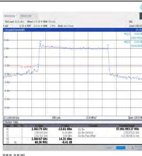
1-N41-30-60-M-7-CP-16QAM-Outer_Full-162@0-A nt1-57.902-60.360-≤60-PASS
