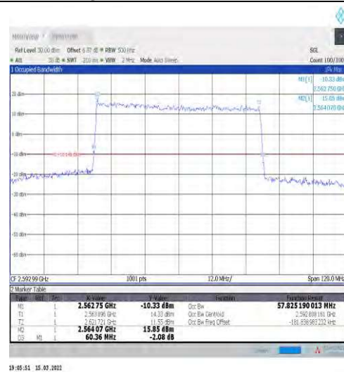
1-N41-30-60-M-1-DFT-QPSK-Outer_Full-162@0-Ant 1-57.825-60.360-≤60-PASS
