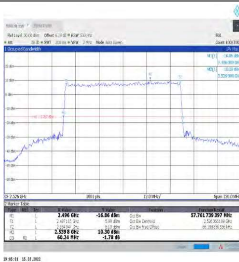
1-N41-30-60-L-9-CP-256QAM-Outer_Full-162@0-An t1-57.762-60.240-≤60-PASS
