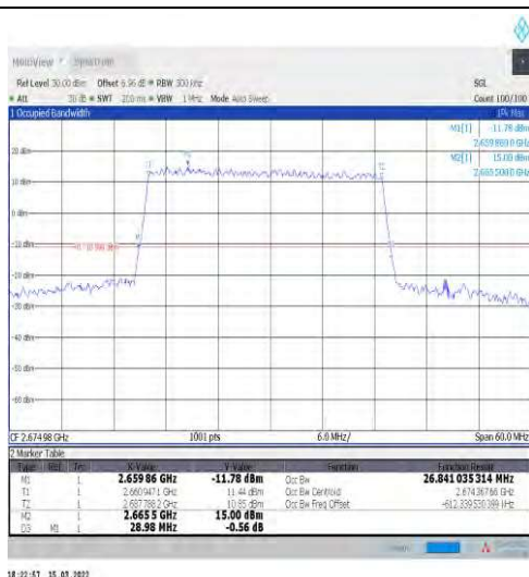
1-N41-30-30-H-4-DFT-64QAM-Outer_Full-75@0-Ant 1-26.841-28.980-≤30-PASS
