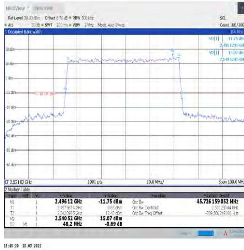
1-N41-30-50-L-4-DFT-64QAM-Outer_Full-128@0-An t1-45.726-48.200-≤50-PASS
