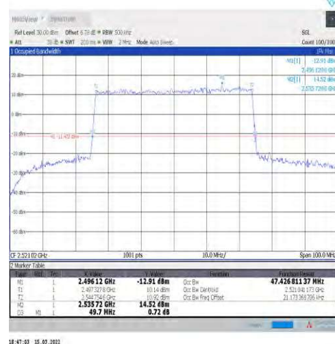
1-N41-30-50-L-7-CP-16QAM-Outer_Full-133@0-Ant 1-47.427-49.700-≤50-PASS
