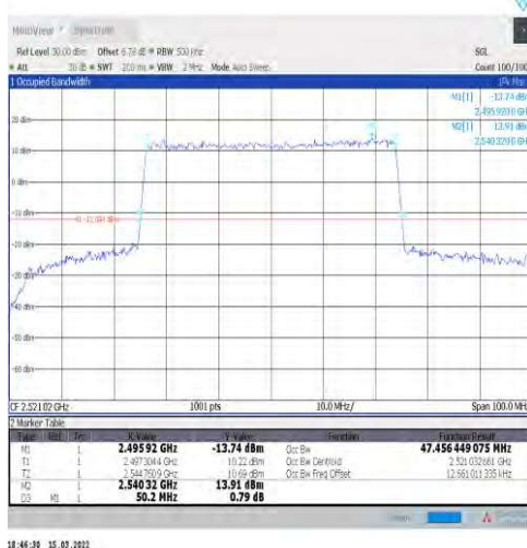
1-N41-30-50-L-6-CP-QPSK-Outer_Full-133@0-Ant1- 47.456-50.200-≤50-PASS
