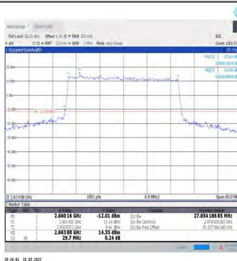
1-N41-30-30-H-7-CP-16QAM-Outer_Full-78@0-Ant1 -27.854-29.700-≤30-PASS
