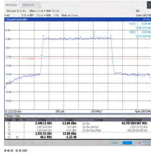
1-N41-30-50-L-5-DFT-256QAM-Outer_Full-128@0-A nt1-45.708-48.100-≤50-PASS
