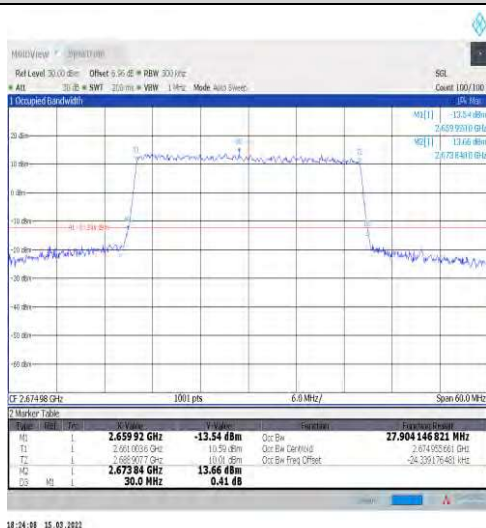
1-N41-30-30-H-6-CP-QPSK-Outer_Full-78@0-Ant1- 27.904-30.000-≤30-PASS
