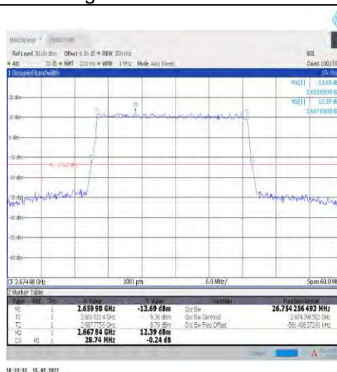
1-N41-30-30-H-5-DFT-256QAM-Outer_Full-75@0-A nt1-26.754-28.740-≤30-PASS
