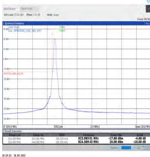
1-N5-15-20-L-4-CP-QPSK-Edge_1RB_Left-1@0-Ant1-seegraph-PASS-see graph
