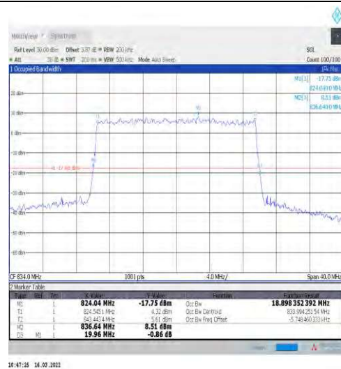
1-N5-15-20-L-9-CP-256QAM-Outer_Full-106@0-Ant 1-18.898-19.960-≤20-PASS
