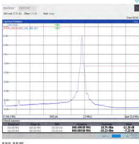
1-N5-15-15-H-5-CP-QPSK-Edge_1RB_Right-1@78-Ant1-seegraph-PASS-see graph
