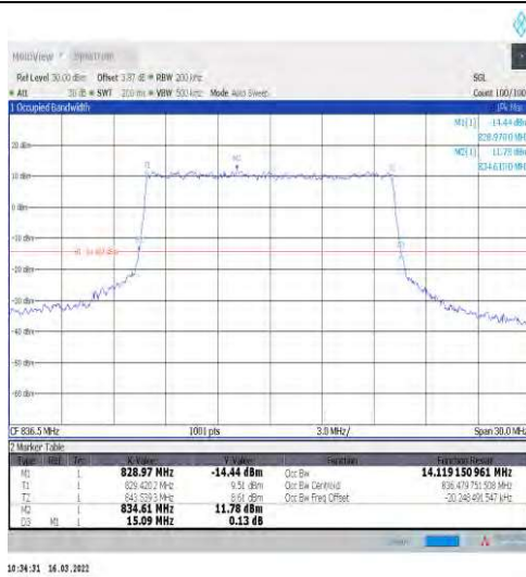
1-N5-15-15-M-6-CP-QPSK-Outer_Full-79@0-Ant1-1 4.119-15.090≤15-PASS
