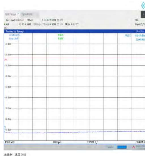
1-N5-15-20-H-1-DFT-PI2BPSK-Inner_1RB_Left-1@ 1-0.15-30-Ant1--90.45--23-PASS
