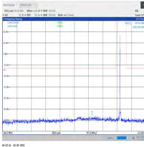
1-N5-15-20-L-1-DFT-PI2BPSK-Inner_1RB_Left-1@1 -30-1000-Ant1--55.66--13-PASS
