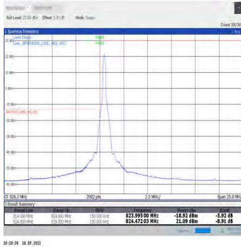
1-N5-15-15-L-1-DFT-PI2BPSK-Edge_1RB_Left-1@0-A nt1-seegraph-PASS-see graph
