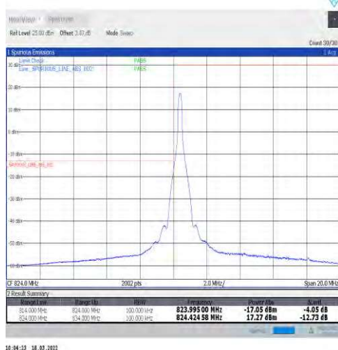
1-N5-15-10-L-4-CP-QPSK-Edge_1RB_Left-1@0-Ant1 seegraph-PASS-see graph
