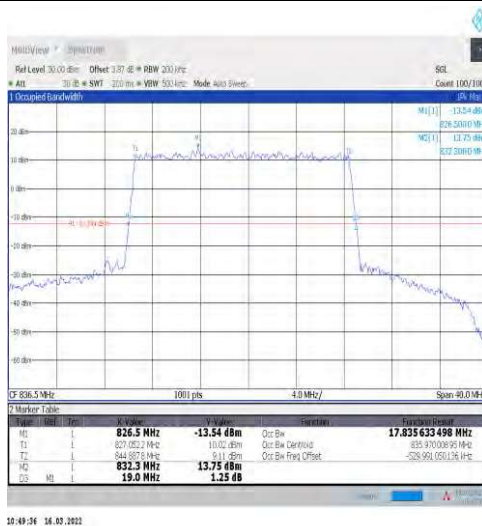
1-N5-15-20-M-1-DFT-QPSK-Outer_Full-100@0-Ant1 -17.836-19.000-≤20-PASS
