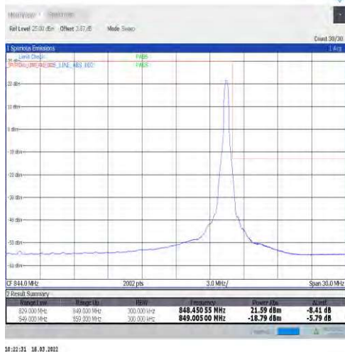
1-N5-15-20-H-2-DFT-PI2BPSK-Edge_1RB_Right-1@105-Ant1-seegraph-PASS-see graph
