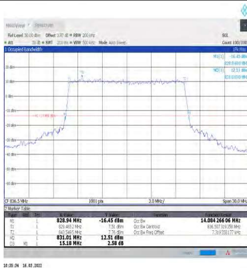
1-N5-15-15-M-8-CP-64QAM-Outer_Full-79@0-Ant1-1 14.084-15.180≤15-PASS
