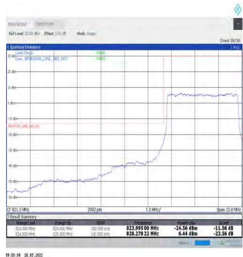
1-N5-15-5-L-3-DFT-PI2BPSK-Outer_Full-25@0-A nt1-seegraph-PASS-see graph
