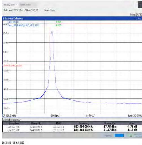
1-N5-15-20-L-1-DFT-PI2BPSK-Edge_1RB_Left-1@0-A nt1-seegraph-PASS-see graph
