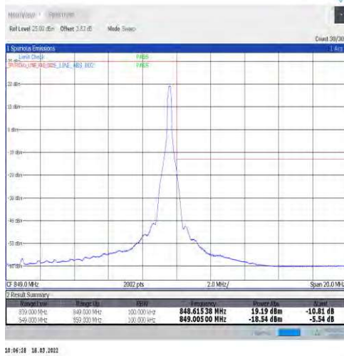
1-N5-15-10-H-2-DFT-PI2BPSK-Edge_1RB_Right-1@5 1-Ant1-seegraph-PASS-see graph
