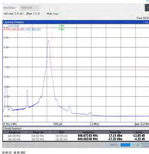
1-N5-15-5-H-5-CP-QPSK-Edge_1RB_Right-1@24-Ant1-seegraph-PASS-see graph
