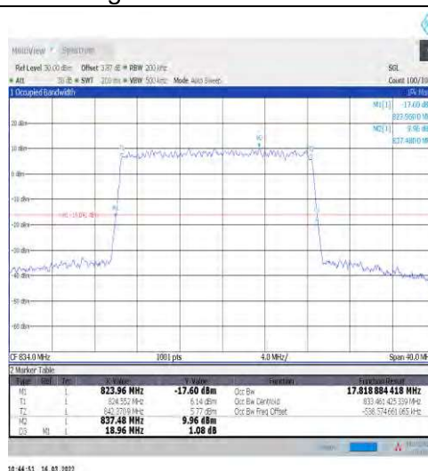
1-N5-15-20-L-5-DFT-256QAM-Outer_Full-100@0-Ant 1-17.819-18.960-≤20-PASS
