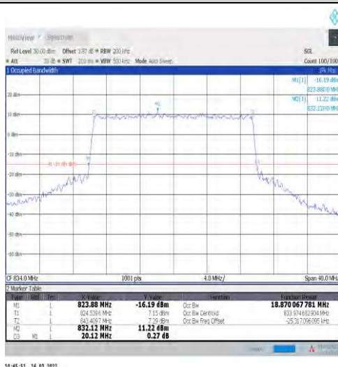
1-N5-15-20-L-6-CP-QPSK-Outer_Full-106@0-Ant1 18.87-20.120-≤20-PASS
