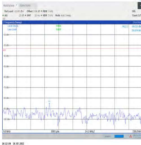
1-N5-15-20-L-1-DFT-PI2BPSK-Inner_1RB_Left-1@1 -0.009-0.15-Ant1--86.53--33-PASS
