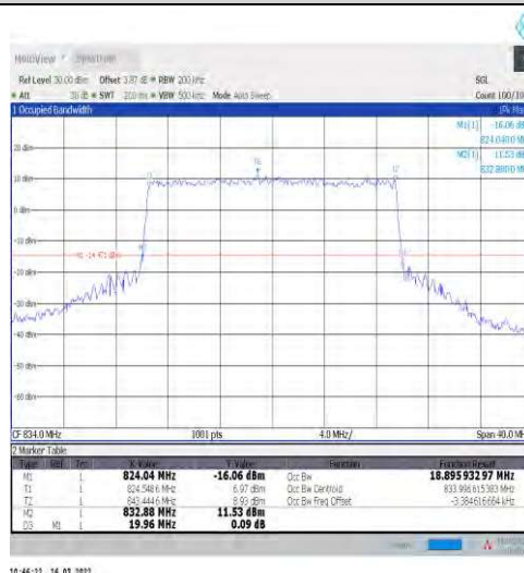
1-N5-15-20-L-7-CP-16QAM-Outer_Full-106@0-Ant1 18.896-19.960-≤20-PASS
