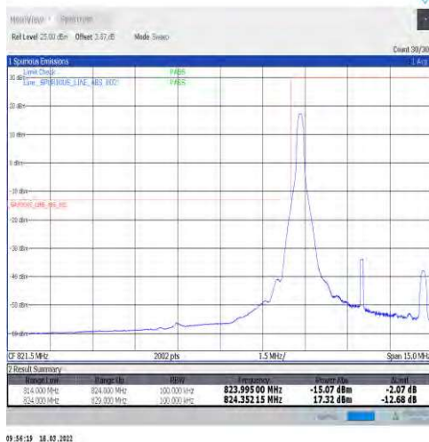
1-N5-15-5-L-4-CP-QPSK-Edge_1RB_Left-1@0-Ant1-s eegraph-PASS-see graph
