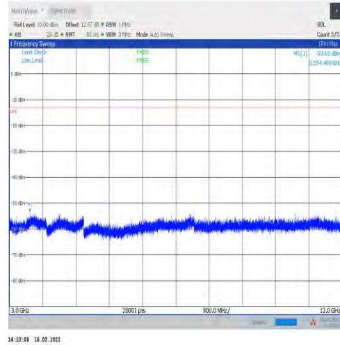
1-N5-15-20-M-1-DFT-PI2BPSK-Inner_1RB_Left-1@ 1-3000-12000-Ant1--53.68--13-PASS
