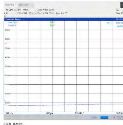
1-N5-15-20-L-1-DFT-PI2BPSK-Inner_1RB_Left-1@1 -0.15-30-Ant1--91.02--23-PASS
