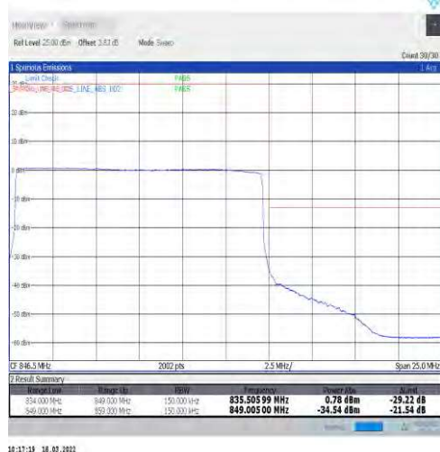
1-N5-15-15-H-6-CP-QPSK-Outer_Full-79@0-Ant1-seegraph-PASS-see graph
