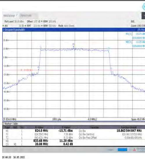
1-N5-15-20-L-8-CP-64QAM-Outer_Full-106@0-Ant1 -18.864-20.080-≤20-PASS
