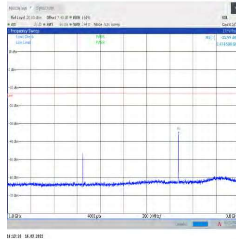
1-N5-15-20-L-1-DFT-PI2BPSK-Inner_1RB_Left-1@1 -1000-3000-Ant1--35.99--13-PASS
