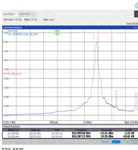
1-N5-15-5-L-1-DFT-PI2BPSK-Edge_1RB_Left-1@0-An t1-seegraph-PASS-see graph
