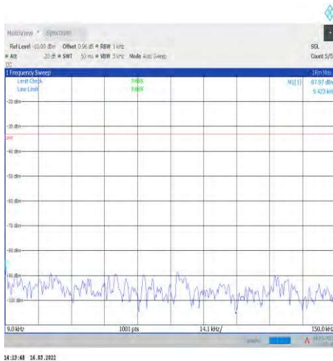
1-N5-15-20-H-1-DFT-PI2BPSK-Inner_1RB_Left-1@ 1-0.009-0.15-Ant1--87.97--33-PASS
