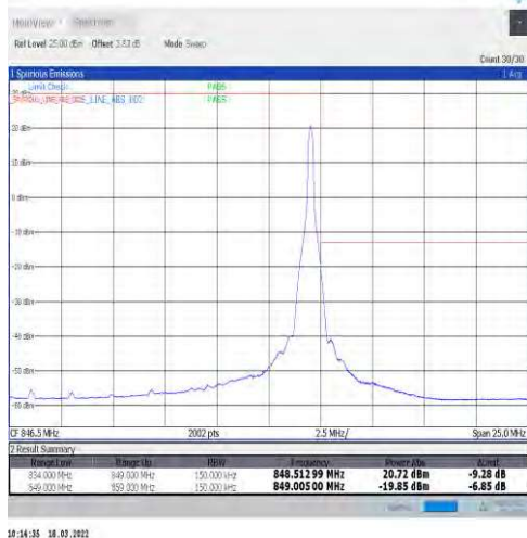
1-N5-15-15-H-2-DFT-PI2BPSK-Edge_1RB_Right-1@7 8-Ant1-seegraph-PASS-see graph
