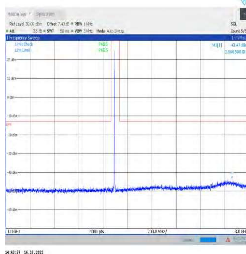
1-N2-15-20-H-1-DFT-PI2BPSK-Inner_1RB_Left-1@1 -1000-3000-Ant1--43.47--13-PASS
