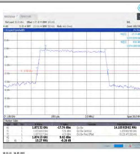
1-N2-15-15-M-9-CP-256QAM-Outer_Full-79@0-Ant1-1 -14.106-15.270≤15-PASS
