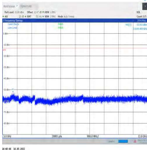
1-N2-15-20-L-1-DFT-PI2BPSK-Inner_1RB_Left-1@1 -3000-12000-Ant1--52.93--13-PASS
