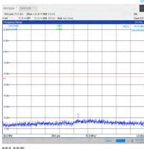
1-N2-15-20-H-1-DFT-PI2BPSK-Inner_1RB_Left-1@ 1-30-1000-Ant1--60.43--23-PASS
