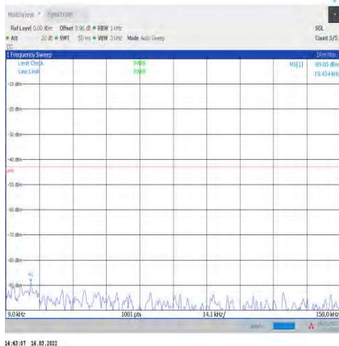
1-N2-15-20-H-1-DFT-PI2BPSK-Inner_1RB_Left-1@ 1-0.009-0.15-Ant1--89.05--43-PASS
