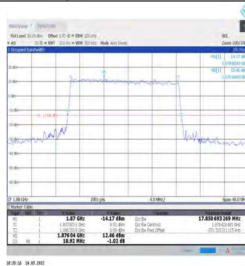
1-N2-15-20-M-4-DFT-64QAM-Outer_Full-100@0-Ant 1-17.851-18.920-≤20-PASS
