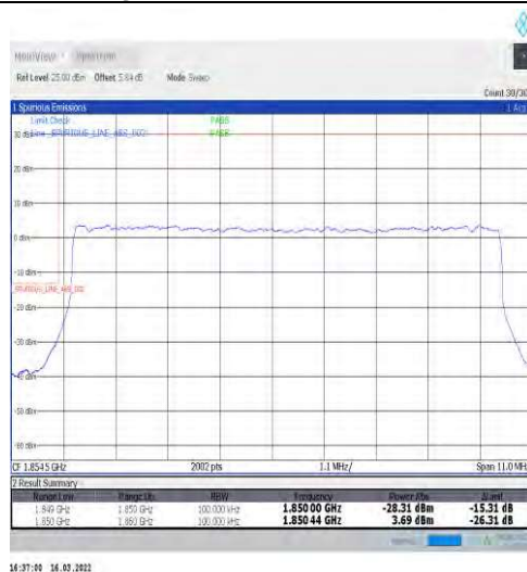
1-N2-15-10-L-3-DFT-PI2BPSK-Outer_Full-50@0-Ant1-seegraph-PASS-see graph
