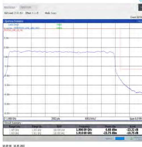
1-N2-15-5-H-3-DFT-PI2BPSK-Outer_Full-25@0-Ant1-seegraph-PASS-see graph
