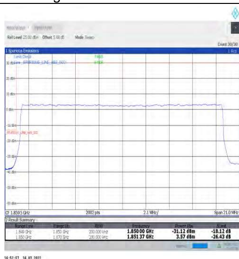
1-N2-15-20-L-3-DFT-PI2BPSK-Outer_Full-100@0-Ant1-seegraph-PASS-see graph
