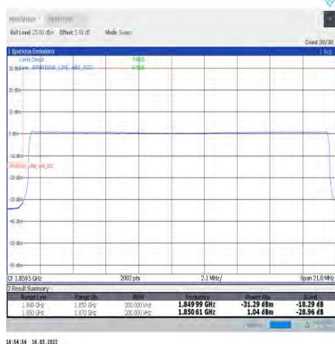
1-N2-15-20-L-6-CP-QPSK-Outer_Full-106@0-Ant1-seegraph-PASS-see graph
