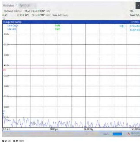
1-N2-15-20-M-1-DFT-PI2BPSK-Inner_1RB_Left-1@1 1-0.009-0.15-Ant1--87.35--43-PASS
