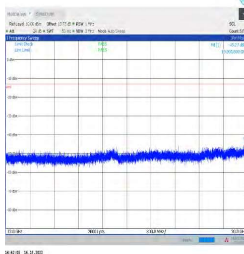
1-N2-15-20-M-1-DFT-PI2BPSK-Inner_1RB_Left-1@1 -12000-20000-Ant1--45.27--13-PASS
