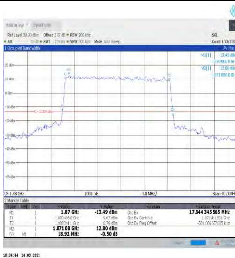
1-N2-15-20-M-3-DFT-16QAM-Outer_Full-100@0-Ant 1-17.844-18.920-≤20-PASS
