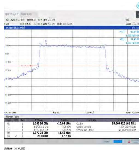
1-N2-15-20-M-6-CP-QPSK-Outer_Full-106@0-Ant1 18.864-20.000-≤20-PASS
