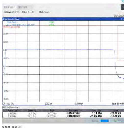
1-N2-15-15-H-6-CP-QPSK-Outer_Full-79@0-Ant1-seegraph-PASS-see graph
