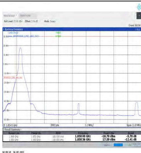
1-N2-15-10-L-4-CP-QPSK-Edge_1RB_Left-1@0-Ant1-seegraph-PASS-see graph
