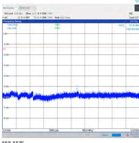
1-N2-15-20-M-1-DFT-PI2BPSK-Inner_1RB_Left-1@ 1-3000-12000-Ant1--52.96--13-PASS
