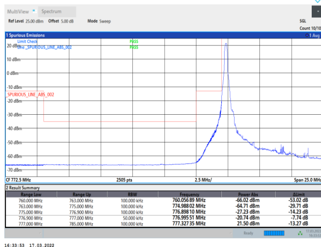
Band13-5MHz-QPSK-23205-25RB#0
