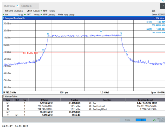
Band13-5MHz-QPSK-23230-25RB#0
