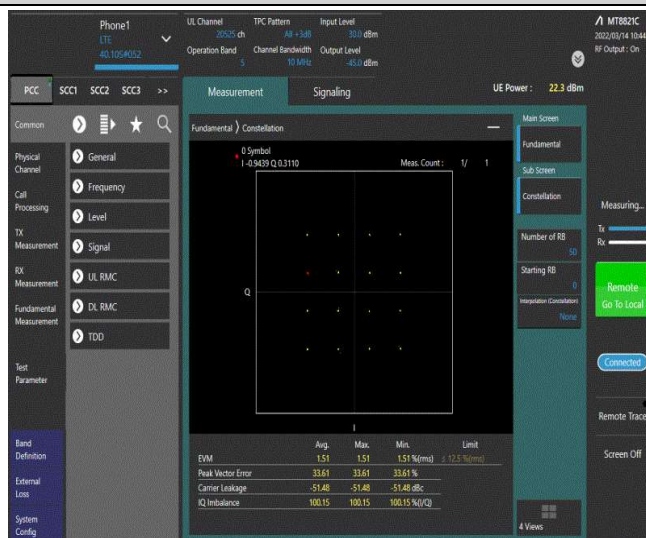
Band5-10MHz-16QAM-20525-50RB#0
