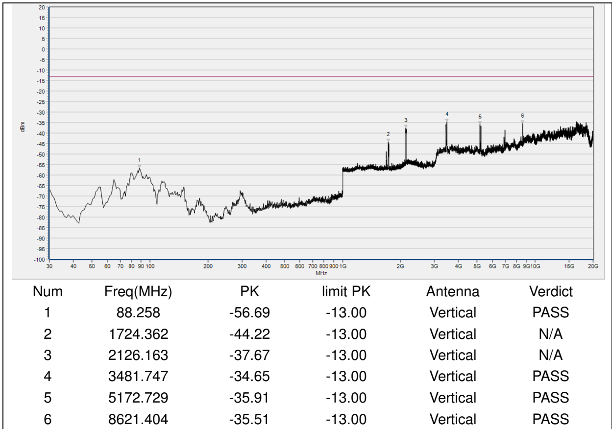
(LTE Band4, 20MHz BW, QPSK, Mid Channel, Vertical)
