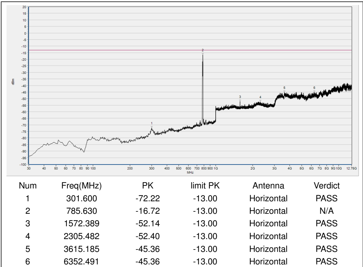
(LTE Band13, 10MHz BW, QPSK, Mid Channel, Horizontal)
