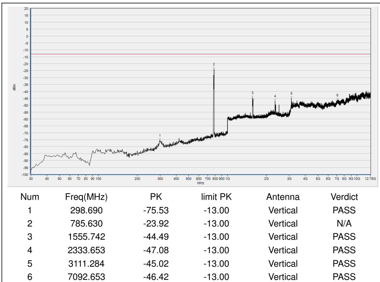
(LTE Band13, 10MHz BW, QPSK, Mid Channel, Vertical)
