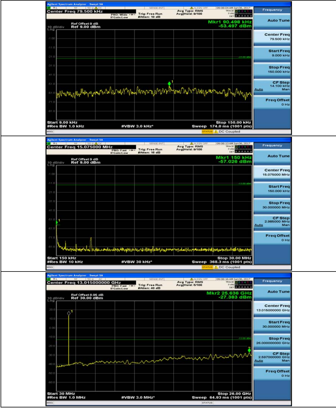
(Channel Bandwidth: 1.4 MHz)_MCH_QPSK_1RB#0
