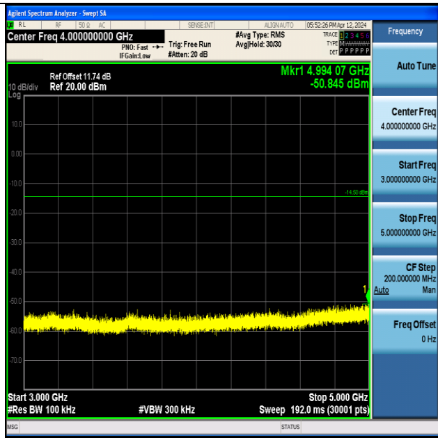
ZIGB-Ant1-2405-3000~5000-PASS
