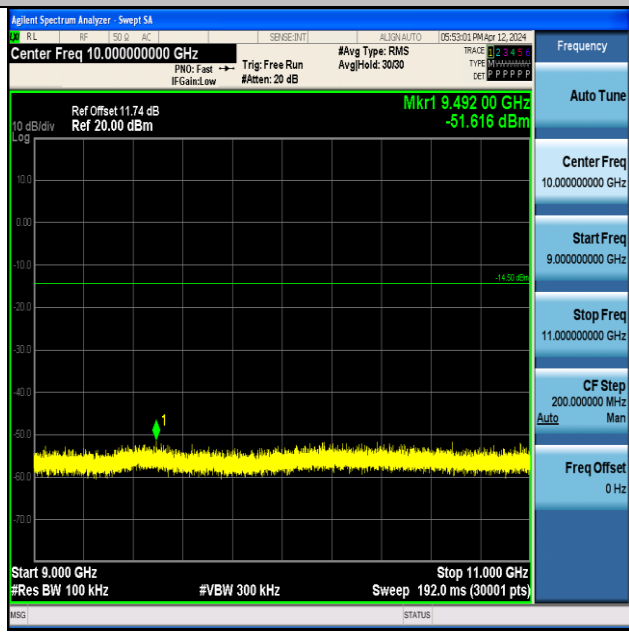
ZIGB-Ant1-2405-9000~11000-PASS
