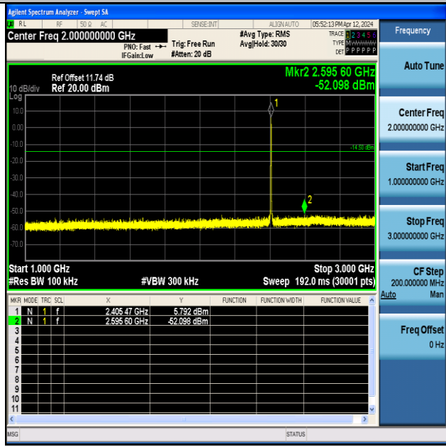
ZIGB-Ant1-2405-1000~3000-PASS
