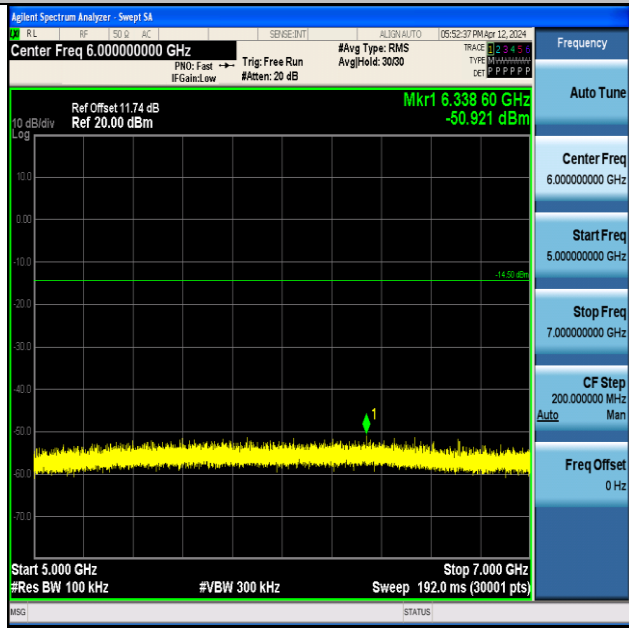
ZIGB-Ant1-2405-5000~7000-PASS
