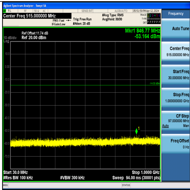
ZIGB-Ant1-2405-30~1000-PASS
