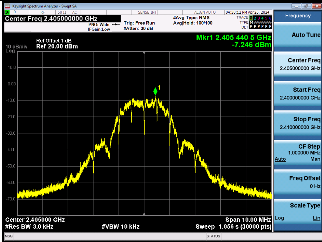
ZIGB-Ant1-2405-PASS
