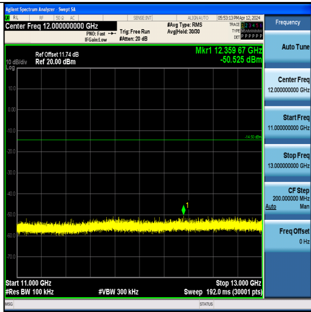
ZIGB-Ant1-2405-11000~13000-PASS
