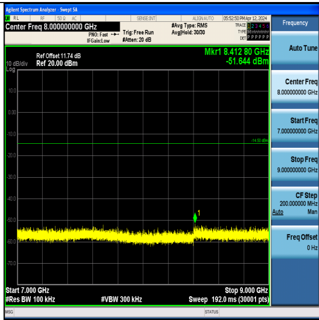
ZIGB-Ant1-2405-7000~9000-PASS
