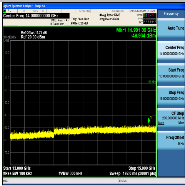
ZIGB-Ant1-2405-13000~15000-PASS
