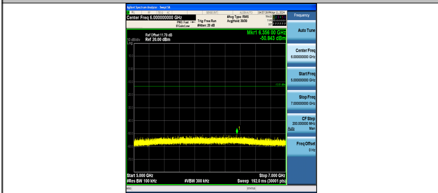
BLE_125K-Ant1-2402-5000~7000-PASS
