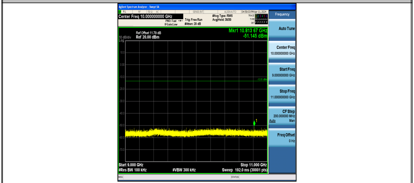
BLE_125K-Ant1-2402-9000~11000-PASS
