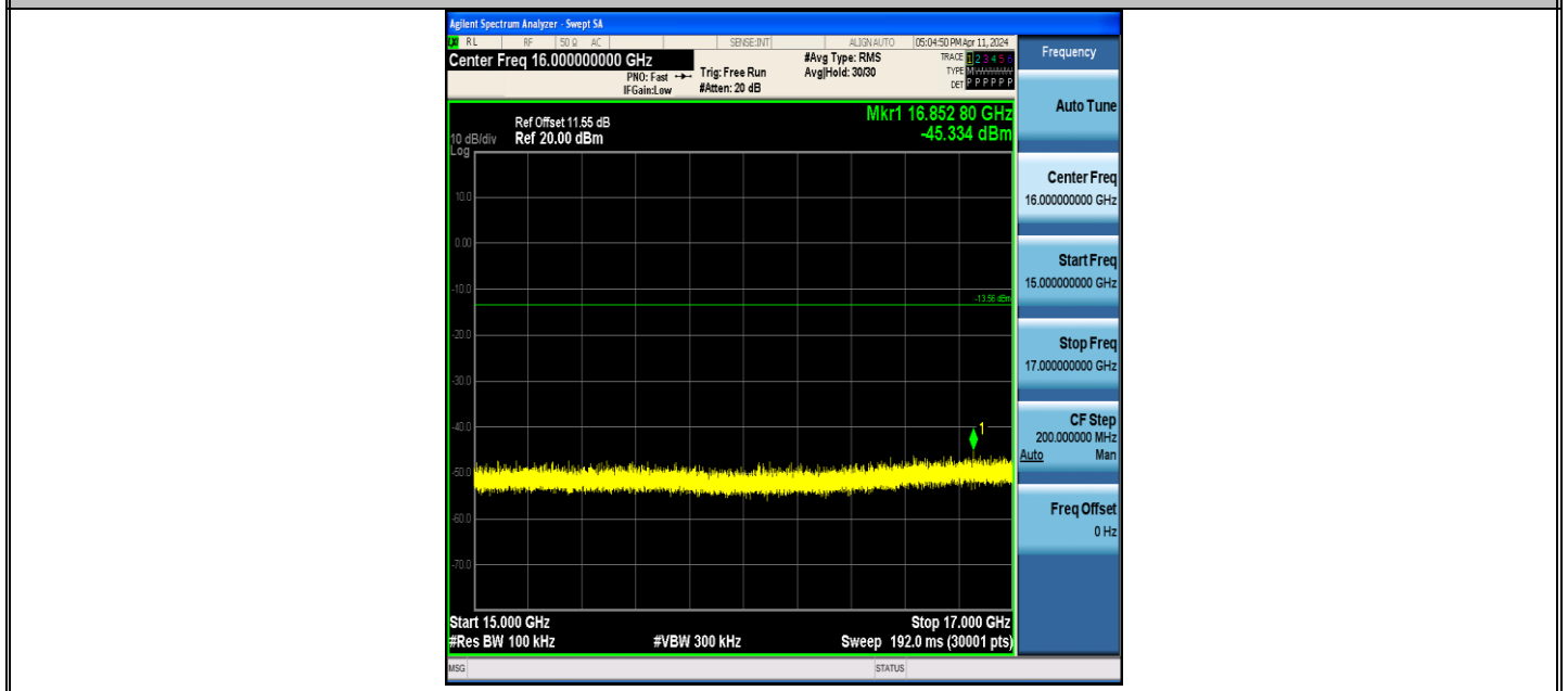
BLE_125K-Ant1-2440-15000~17000-PASS
