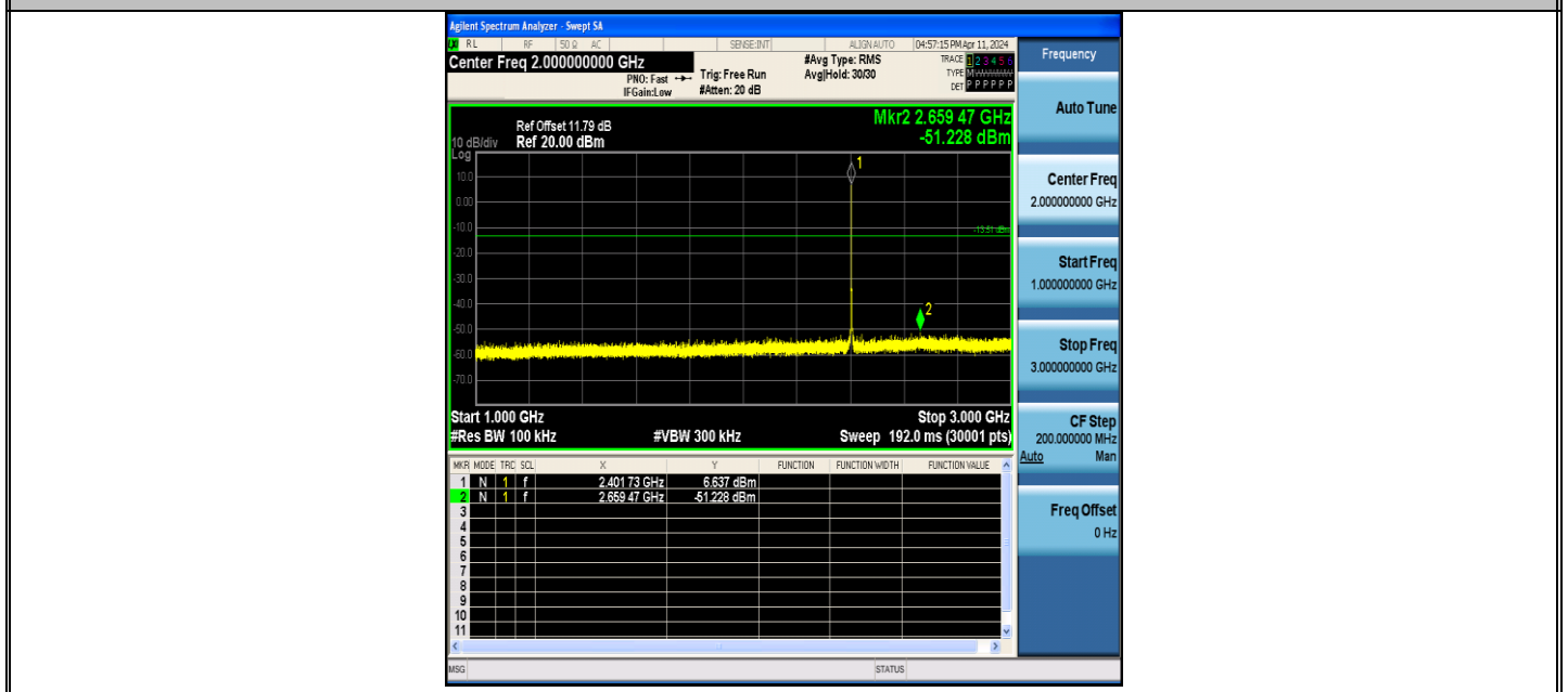
BLE_125K-Ant1-2402-1000~3000-PASS
