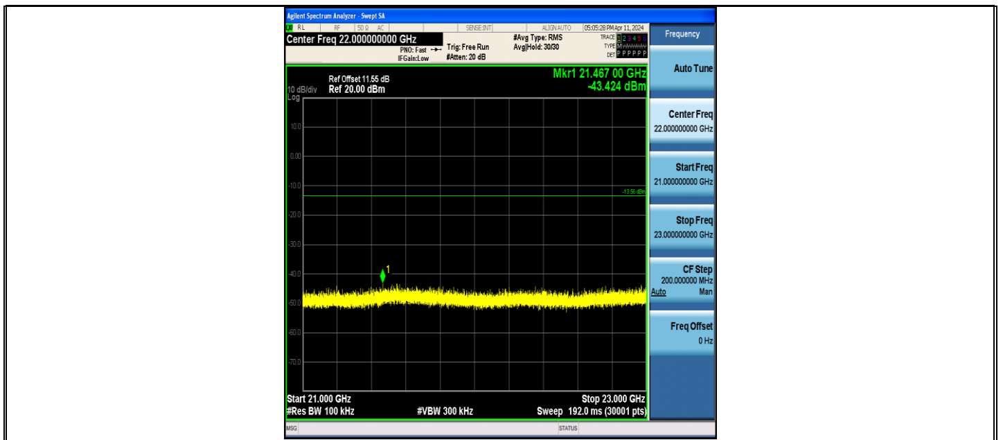
BLE_125K-Ant1-2440-21000~23000-PASS
