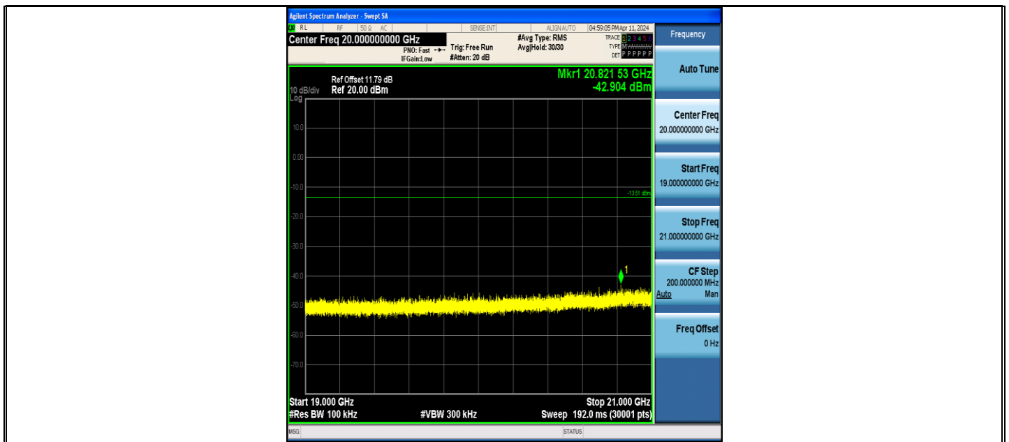
BLE_125K-Ant1-2402-19000~21000-PASS
