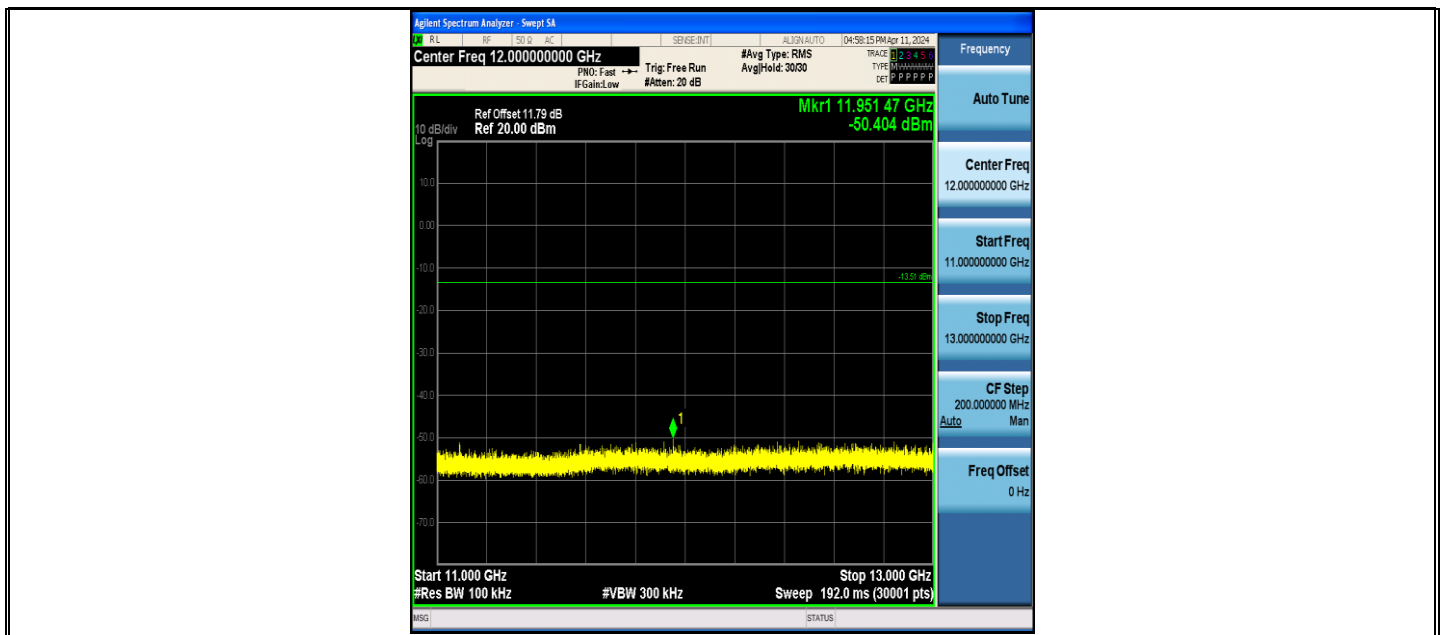
BLE_125K-Ant1-2402-11000~13000-PASS
