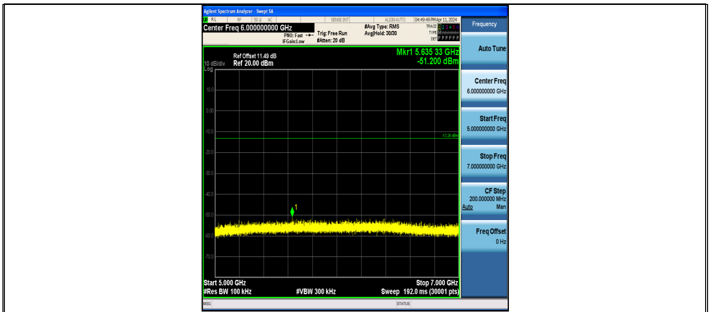
BLE_2M-Ant1-2480-5000~7000-PASS
