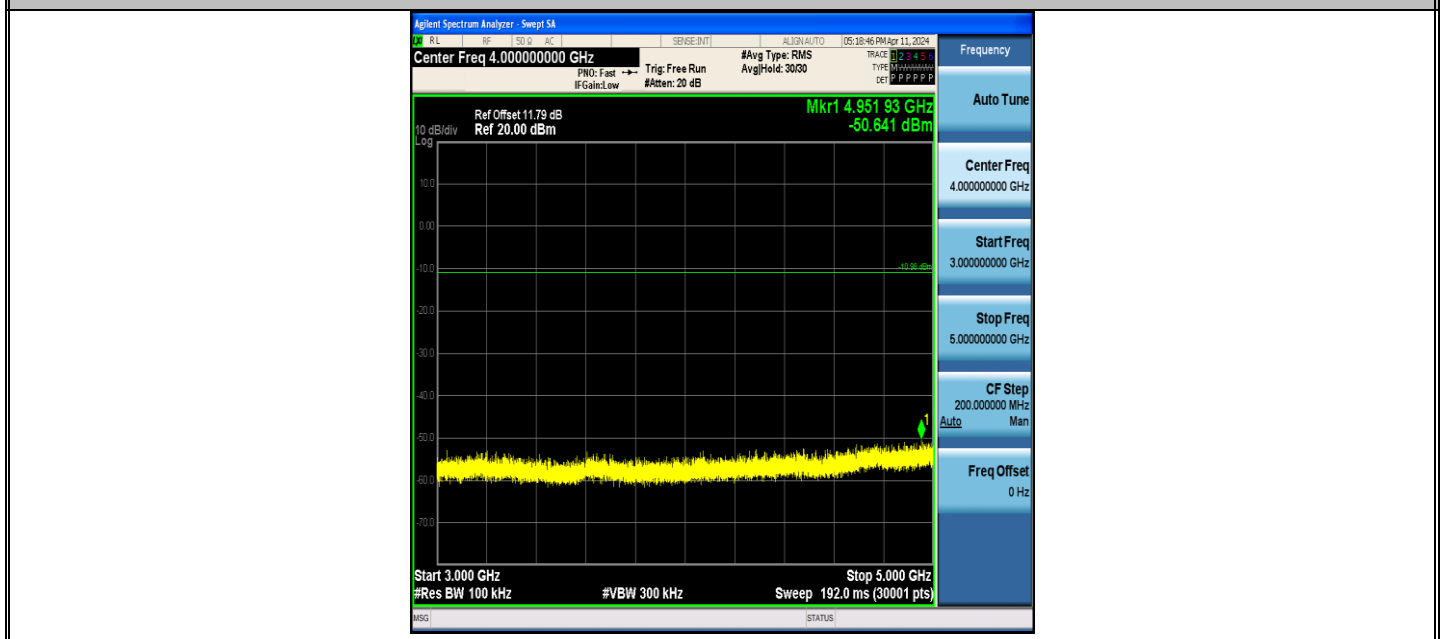
BLE_500K-Ant1-2402-3000~5000-PASS
