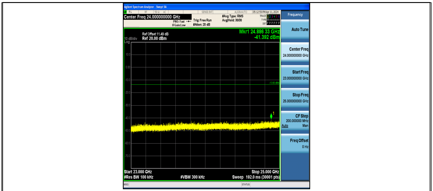
BLE_125K-Ant1-2480-23000~25000-PASS
