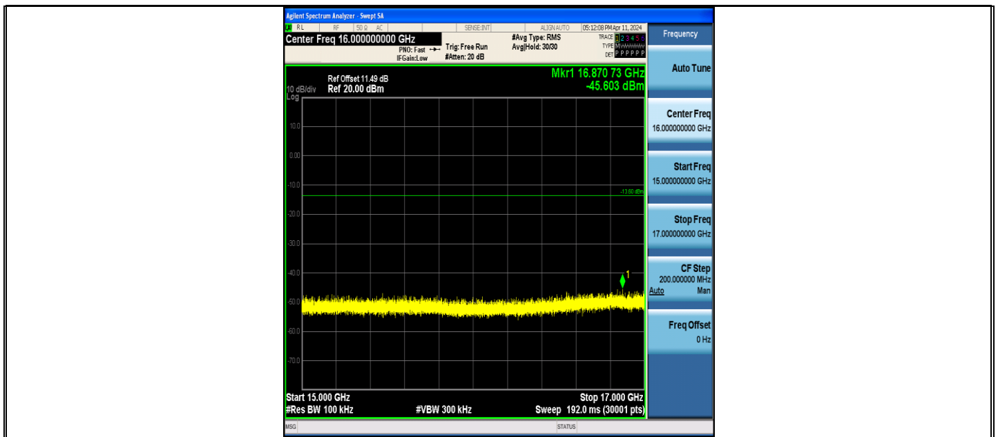
BLE_125K-Ant1-2480-15000~17000-PASS
