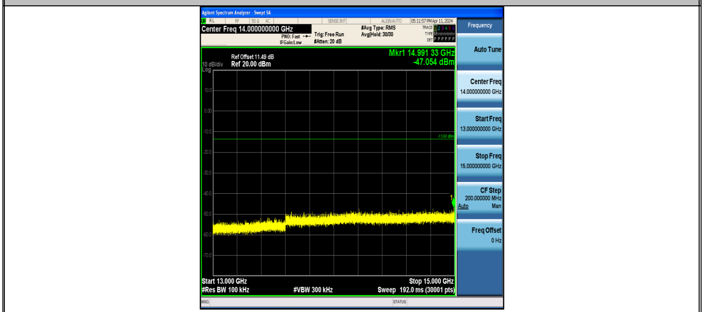
BLE_125K-Ant1-2480-13000~15000-PASS
