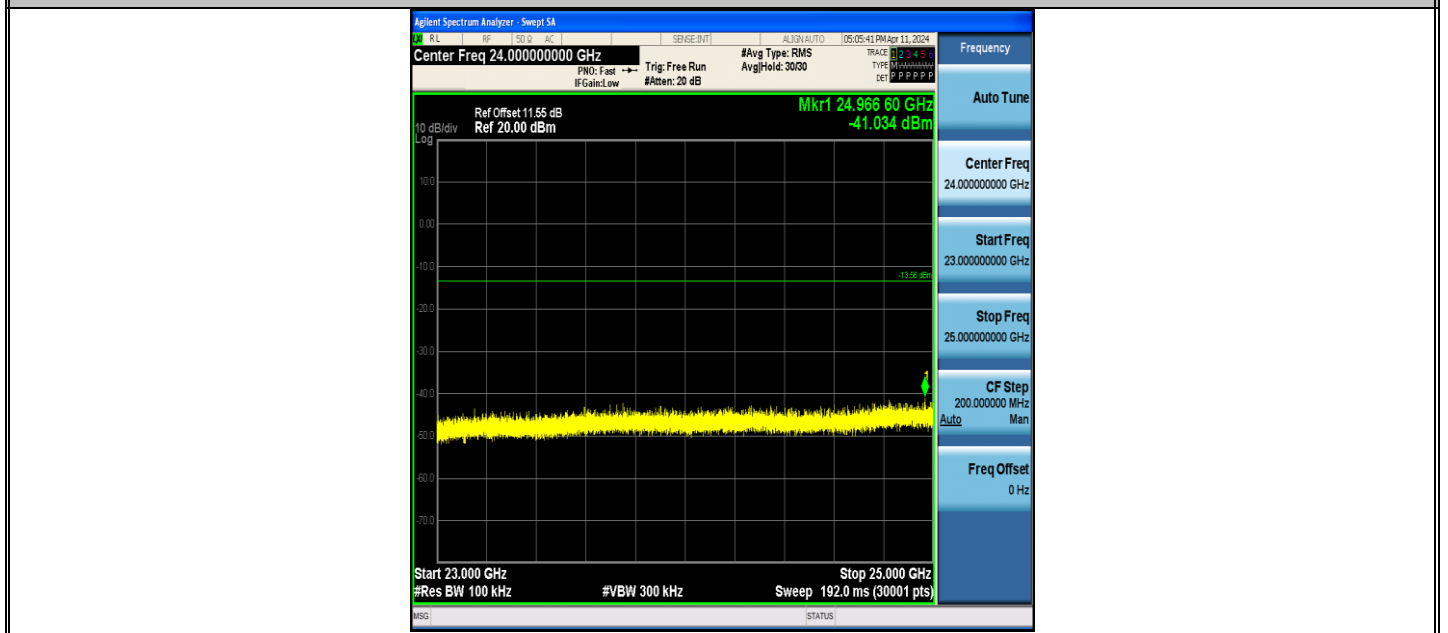
BLE_125K-Ant1-2440-23000~25000-PASS
