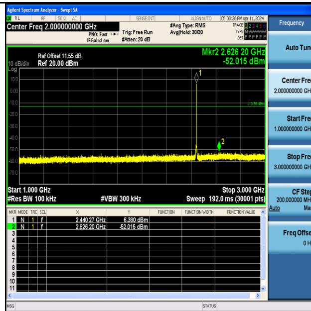
BLE_125K-Ant1-2440-1000~3000-PASS
