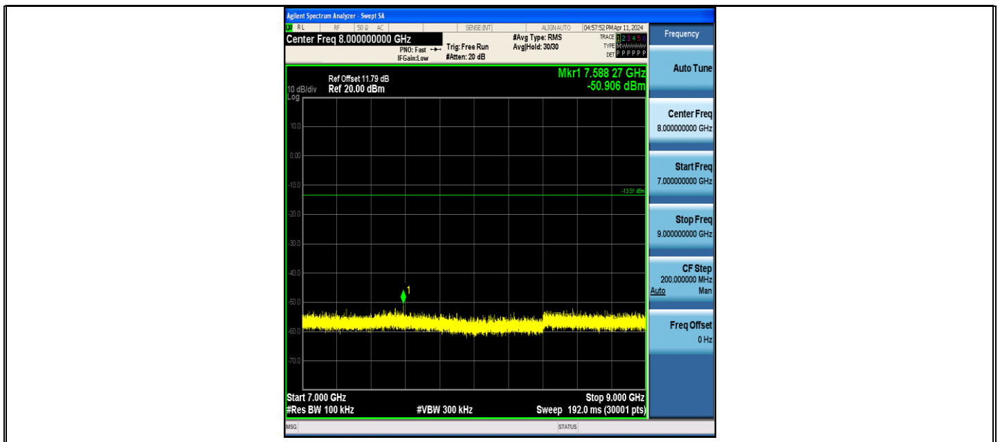
BLE_125K-Ant1-2402-7000~9000-PASS
