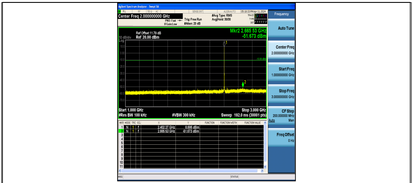
BLE_500K-Ant1-2402-1000~3000-PASS
