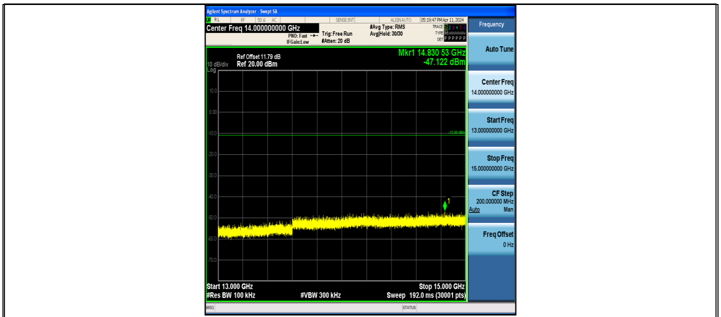
BLE_500K-Ant1-2402-13000~15000-PASS
