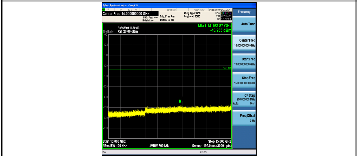
BLE_125K-Ant1-2402-13000~15000-PASS
