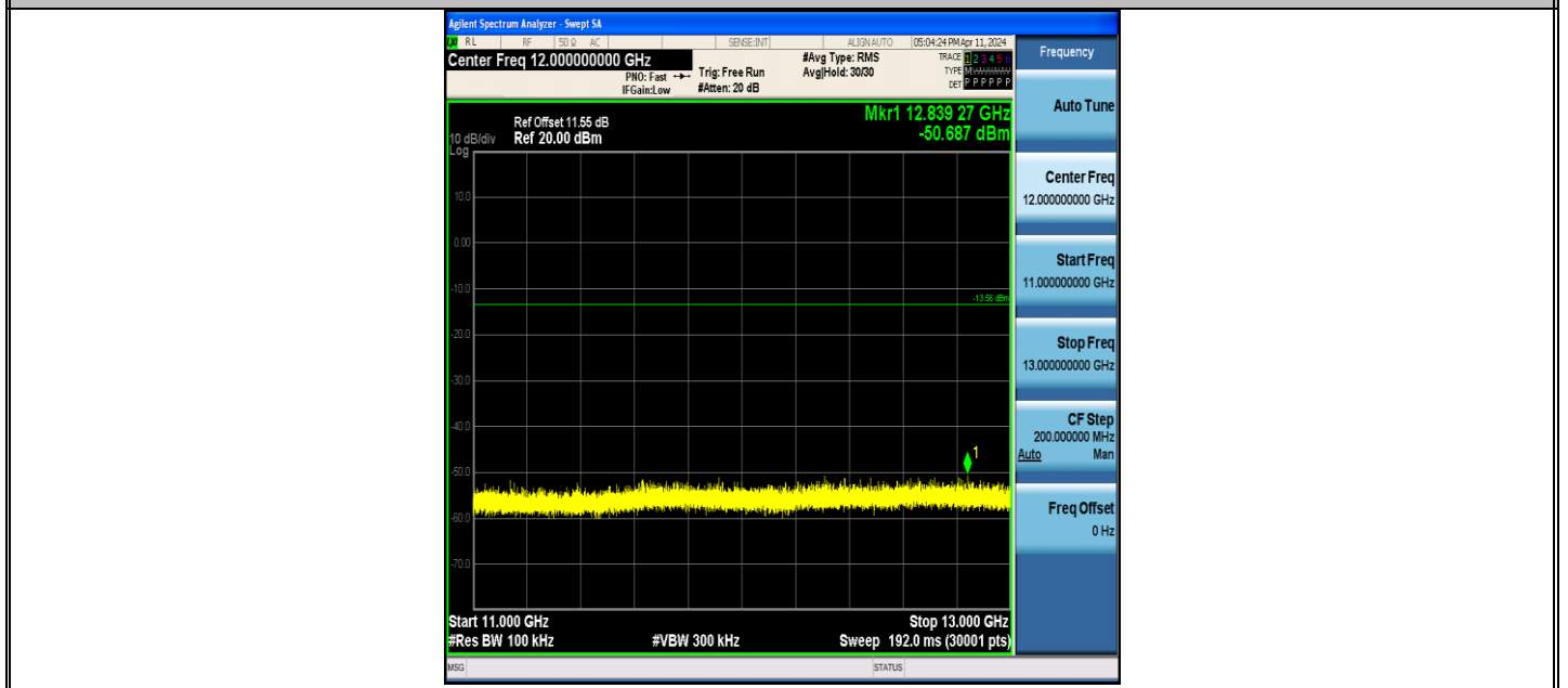
BLE_125K-Ant1-2440-11000~13000-PASS
