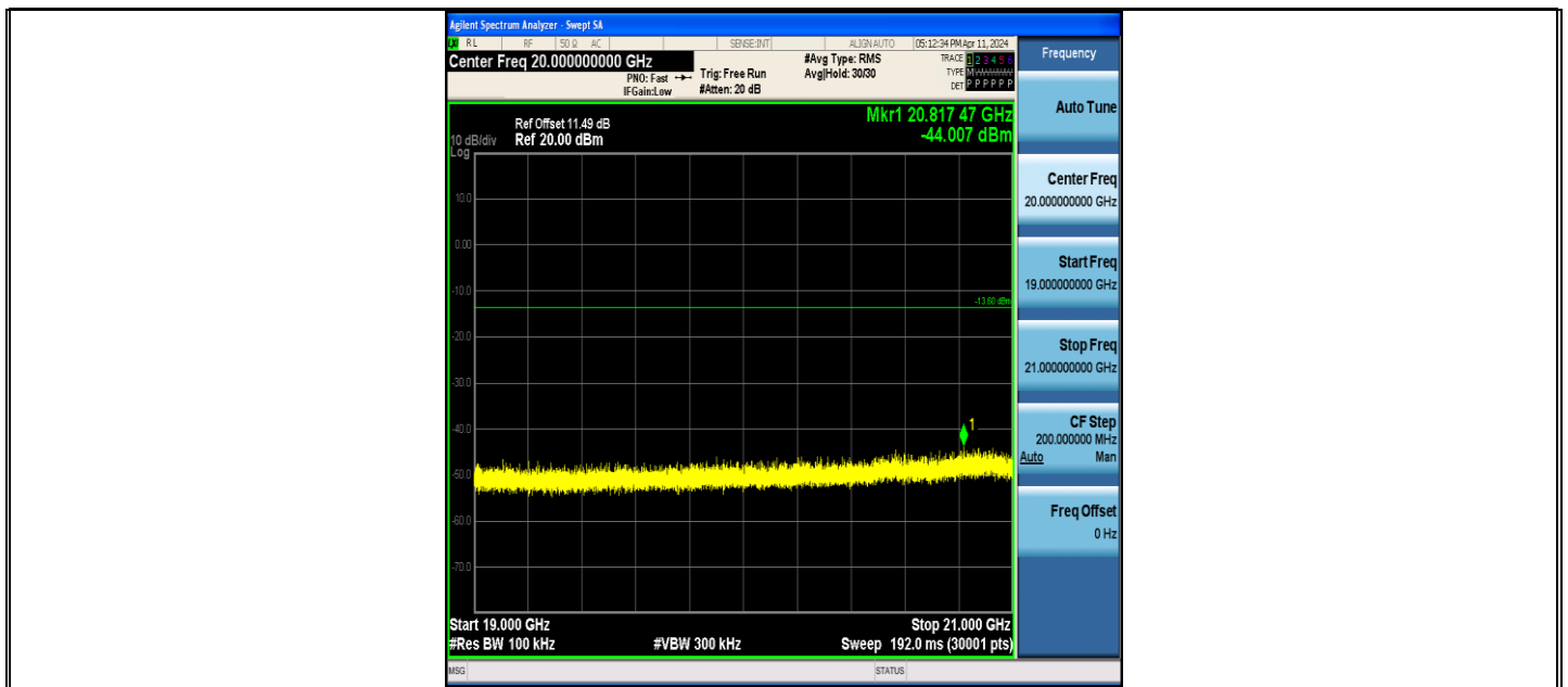
BLE_125K-Ant1-2480-19000~21000-PASS
