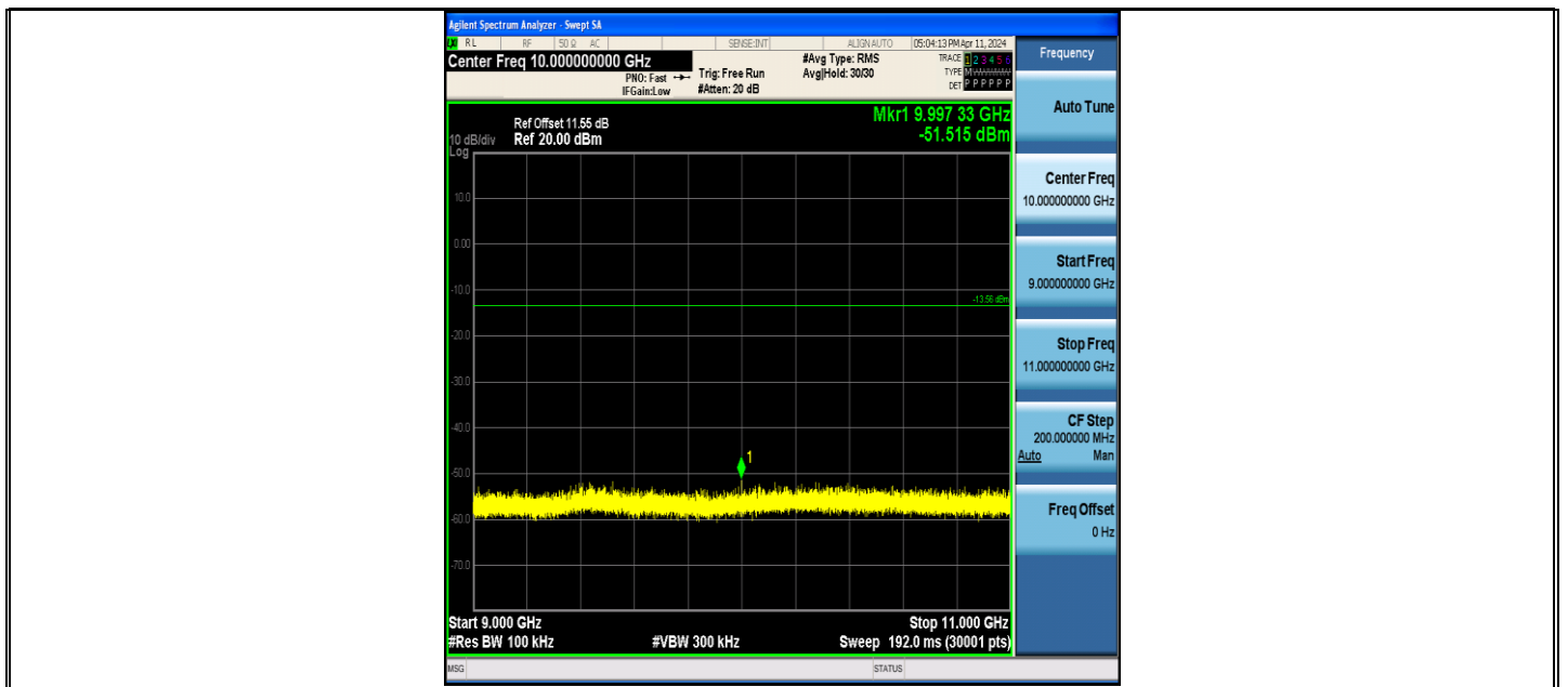
BLE_125K-Ant1-2440-9000~11000-PASS
