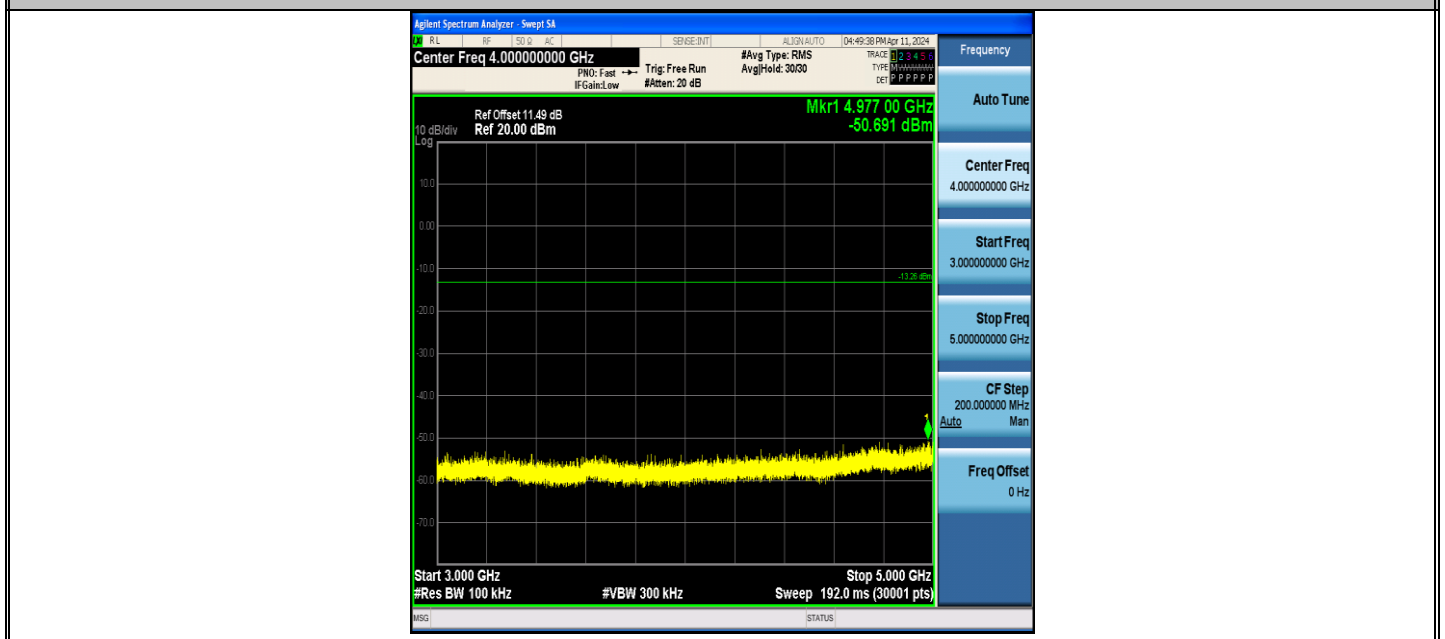
BLE_2M-Ant1-2480-3000~5000-PASS
