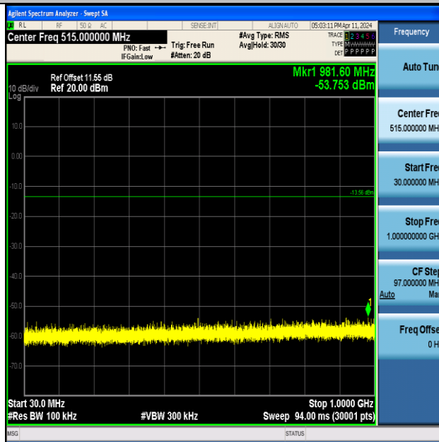
BLE_125K-Ant1-2440-30~1000-PASS
