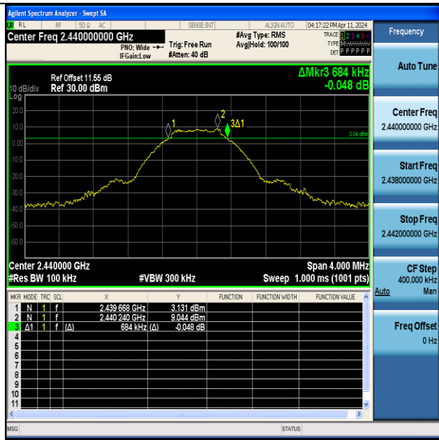
BLE_1M-Ant1-2440-PASS
