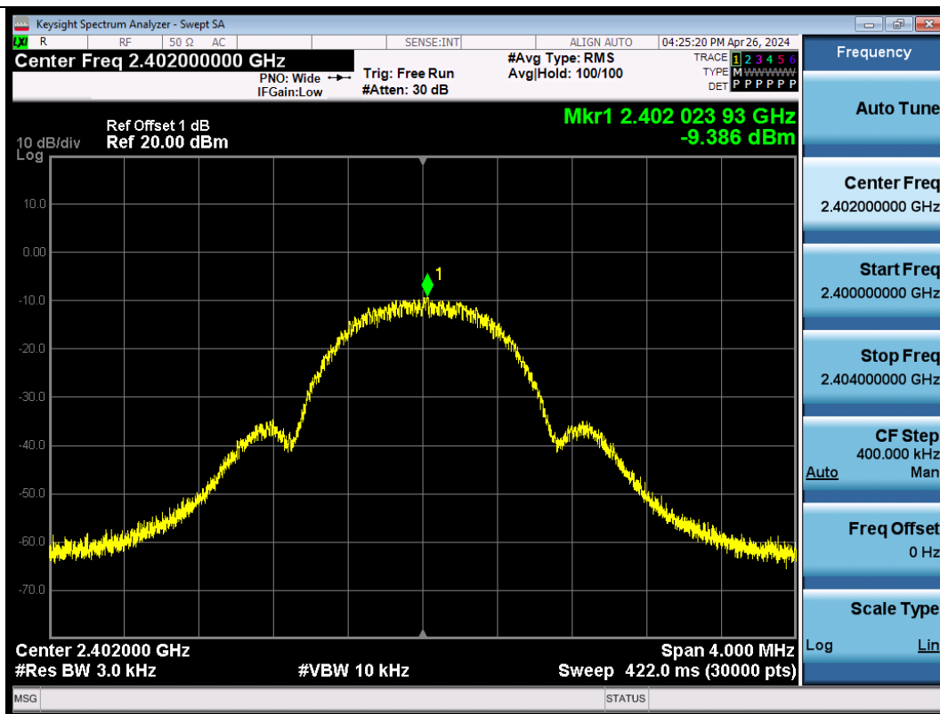
BLE_500K-Ant1-2402-PASS
