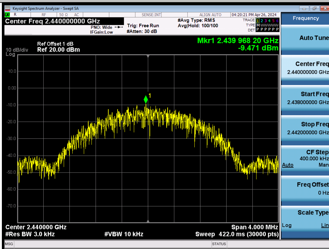
BLE_2M-Ant1-2440-PASS
