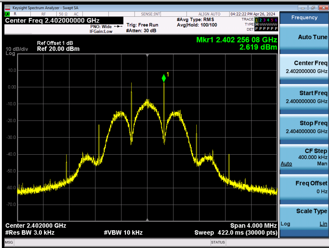
BLE_125K-Ant1-2402-PASS
