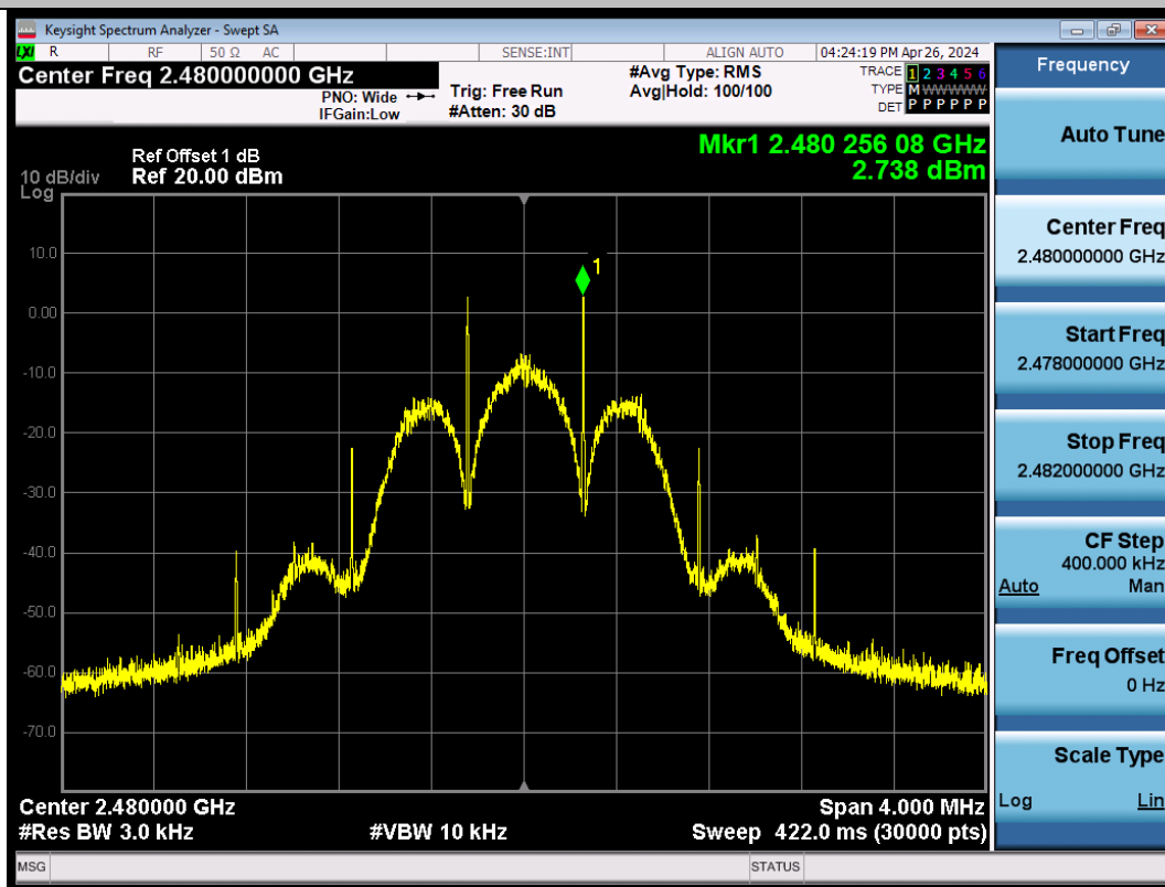
BLE_125K-Ant1-2480-PASS
