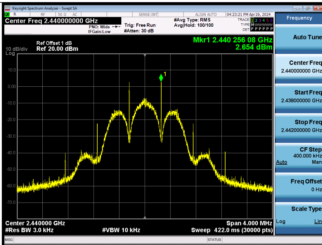
BLE_125K-Ant1-2440-PASS
