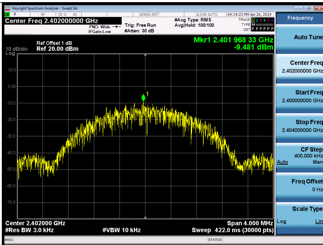
BLE_2M-Ant1-2402-PASS
