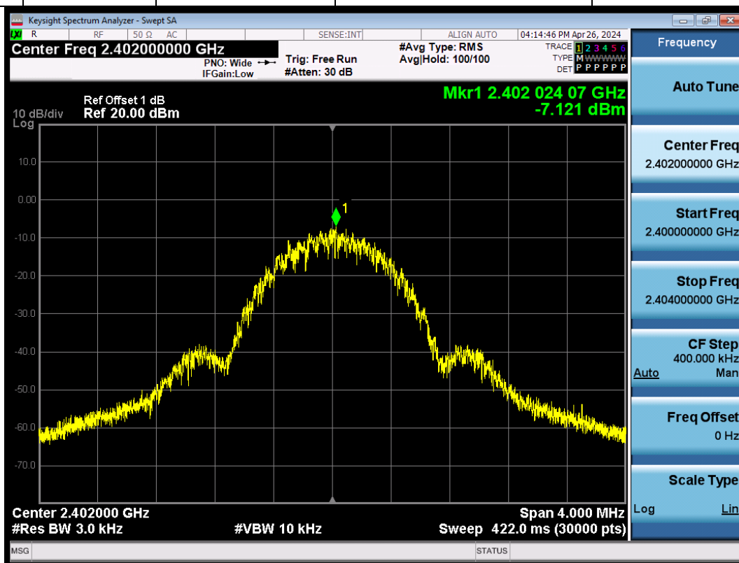
BLE_1M-Ant1-2402-PASS
