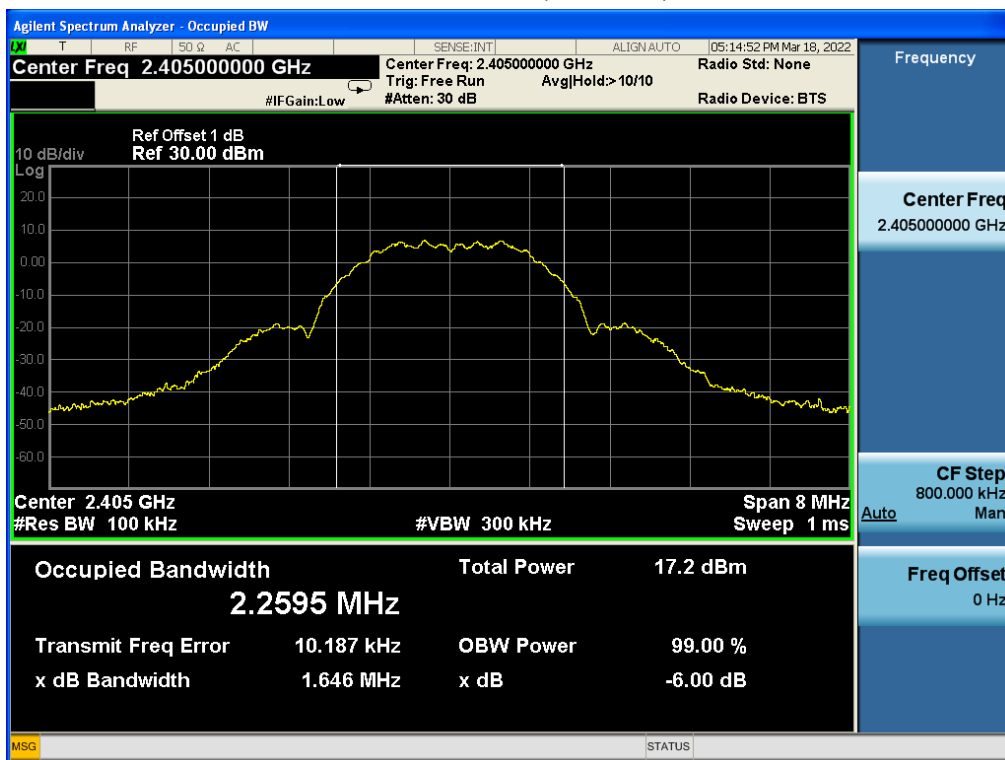
6dB Occupied Bandwidth Mode 1 / CH11 (2405MHz)
