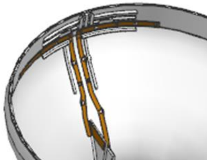
Dipole antenna
