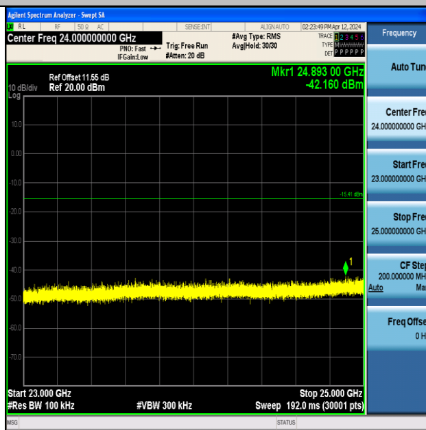
BLE_125K-Ant1-2440-23000~25000-PASS
