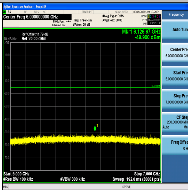
BLE_125K-Ant1-2402-5000~7000-PASS
