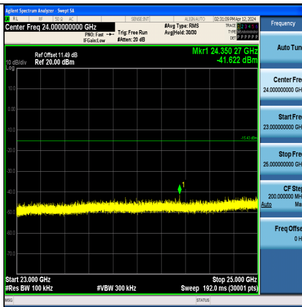
BLE_125K-Ant1-2480-23000~25000-PASS
