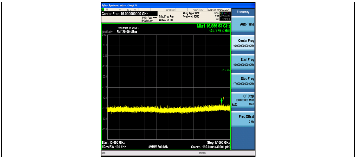
BLE_125K-Ant1-2402-15000~17000-PASS
