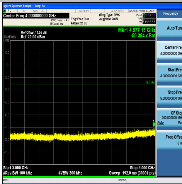
BLE_125K-Ant1-2440-3000~5000-PASS
