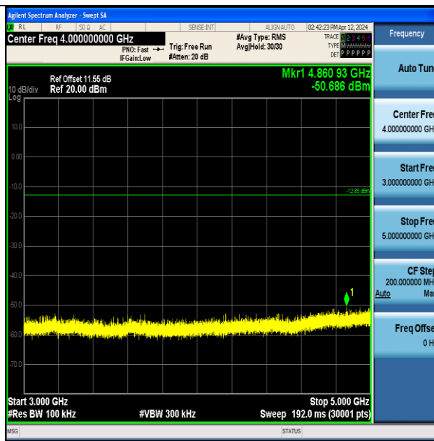
BLE_500K-Ant1-2440-3000~5000-PASS
