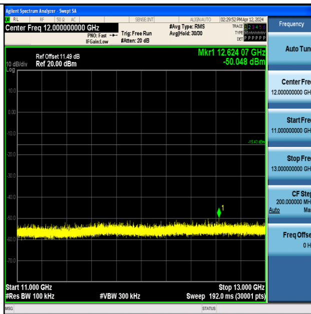
BLE_125K-Ant1-2480-11000~13000-PASS
