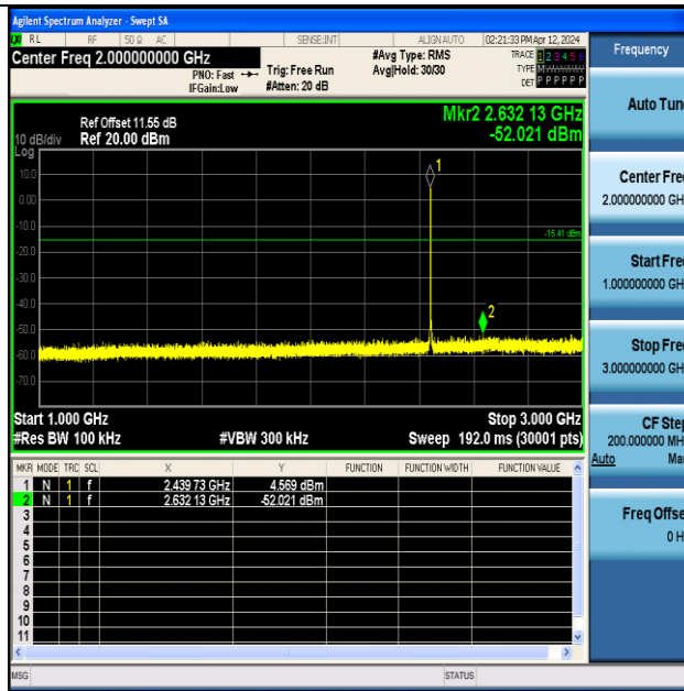
BLE_125K-Ant1-2440-1000~3000-PASS
