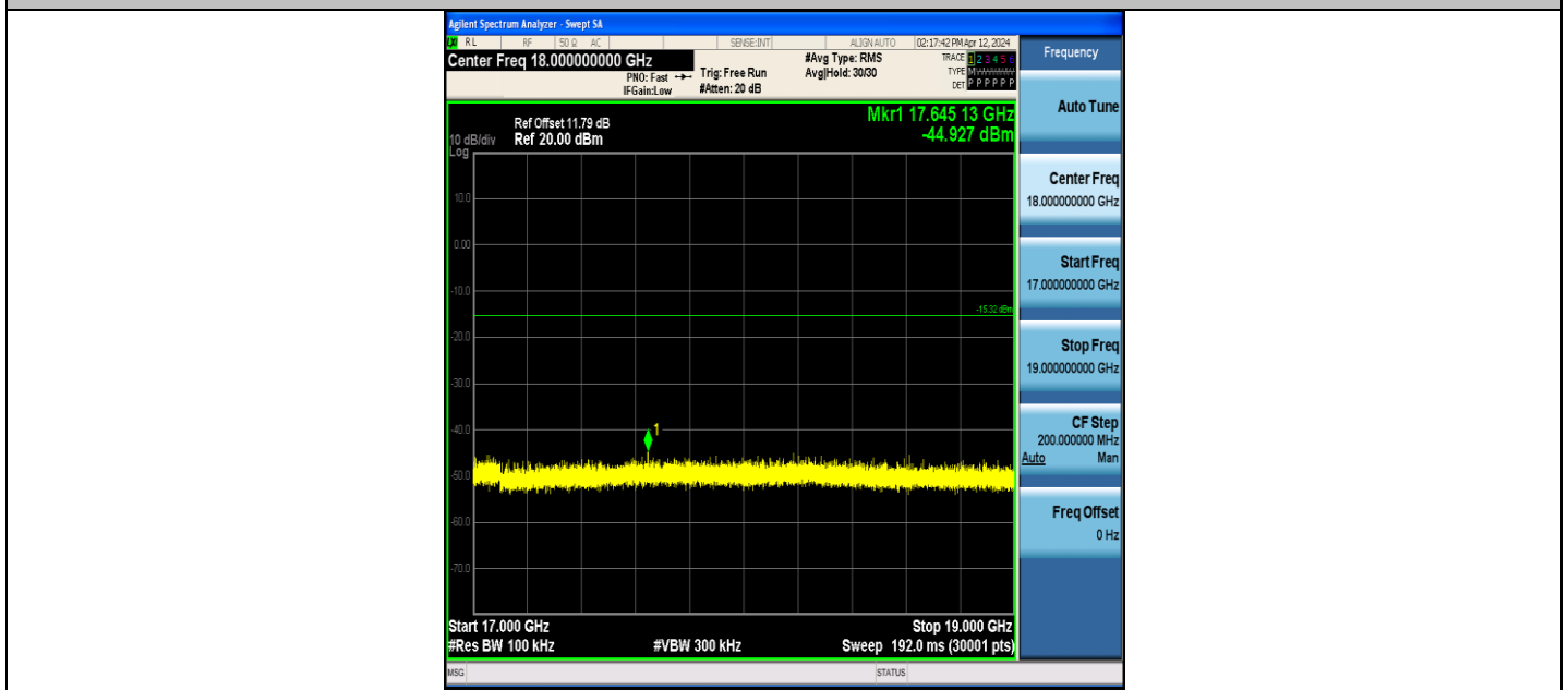
BLE_125K-Ant1-2402-17000~19000-PASS
