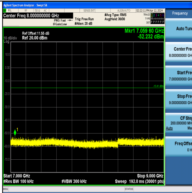
BLE_125K-Ant1-2440-7000~9000-PASS
