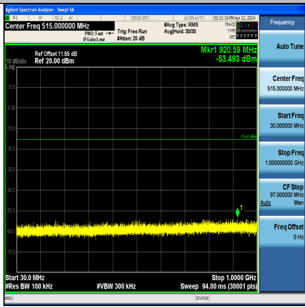
BLE_125K-Ant1-2440-30~1000-PASS
