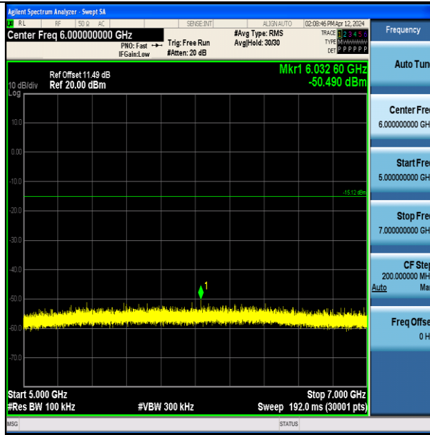
BLE_2M-Ant1-2480-5000~7000-PASS
