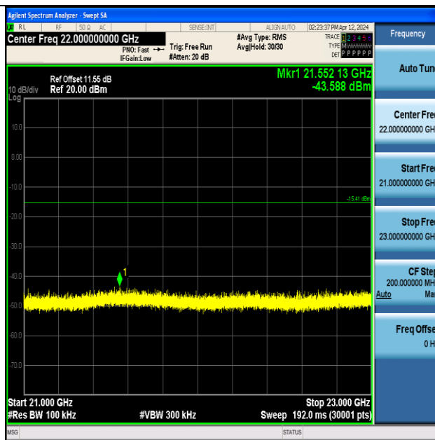
BLE_125K-Ant1-2440-21000~23000-PASS
