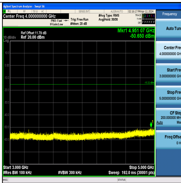
BLE_125K-Ant1-2402-3000~5000-PASS
