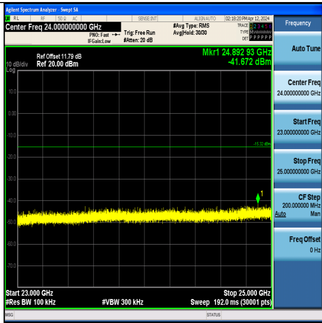
BLE_125K-Ant1-2402-23000~25000-PASS
