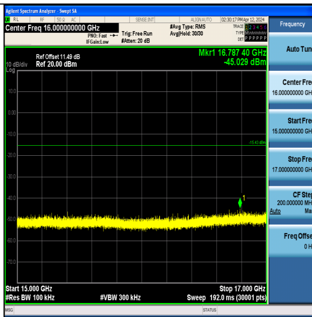
BLE_125K-Ant1-2480-15000~17000-PASS
