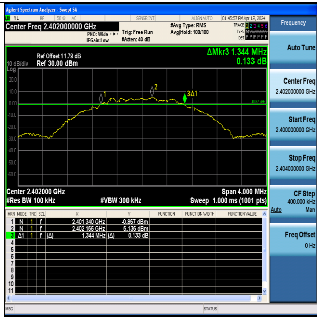
BLE_2M-Ant1-2402-PASS
