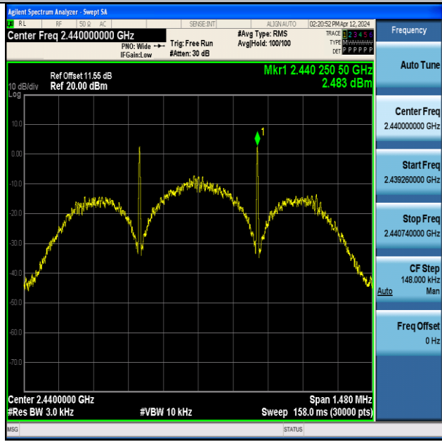
BLE_125K-Ant1-2440-PASS
