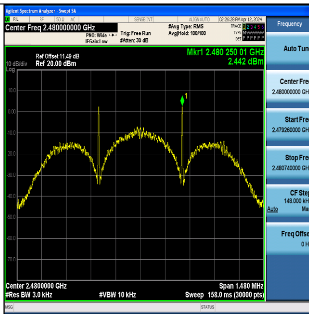
BLE_125K-Ant1-2480-PASS
