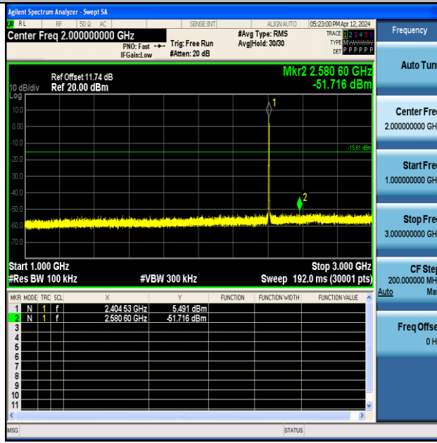
ZIGB-Ant1-2405-1000~3000-PASS
