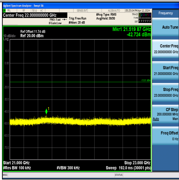
ZIGB-Ant1-2405-21000~23000-PASS
