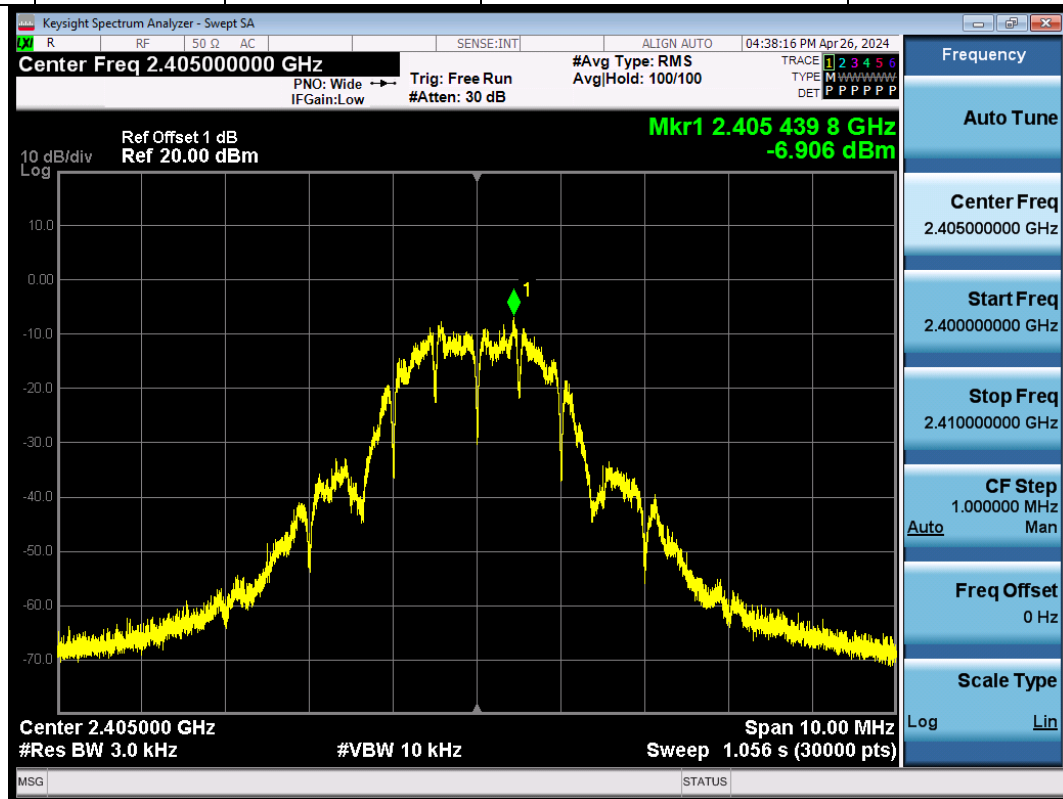
ZIGB-Ant1-2405-PASS
