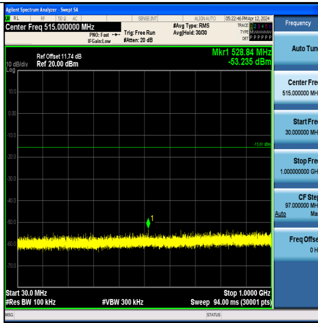
ZIGB-Ant1-2405-30~1000-PASS
