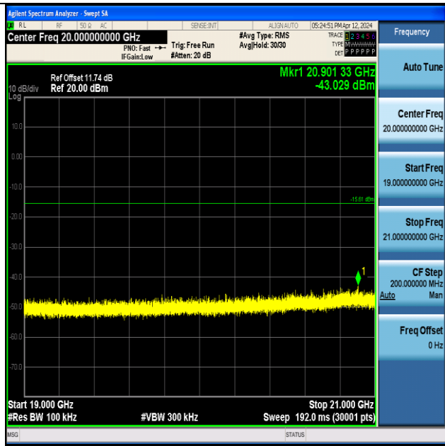
ZIGB-Ant1-2405-19000~21000-PASS
