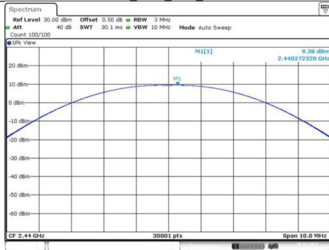
BLE_125K_Ant1_2440
