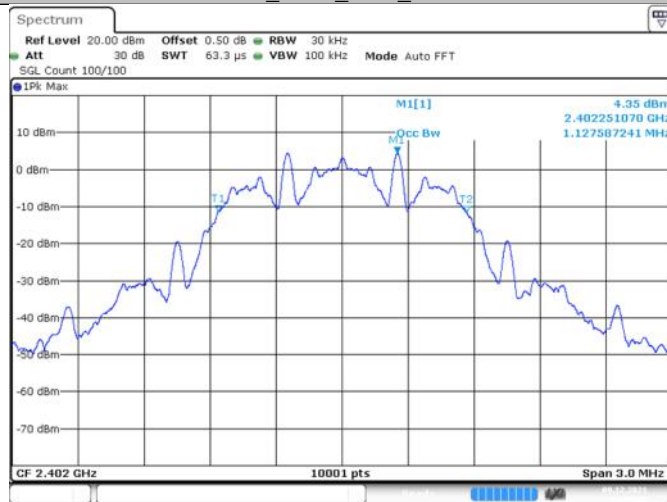
BLE_125K_Ant1_2402
