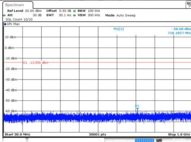
BLE_125K_Ant1_2402_30~1000
