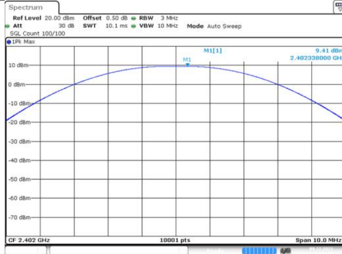
BLE_125K_Ant1_2402
