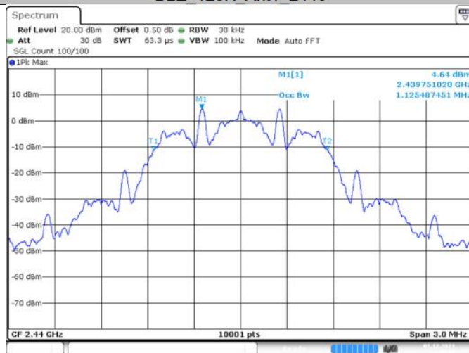
BLE_125K_Ant1_2440
