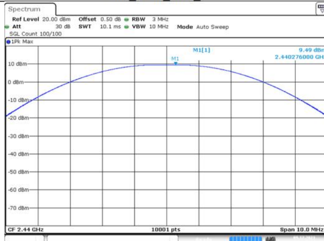
BLE_125K_Ant1_2440
