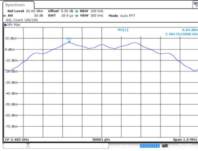
BLE_125K_Ant1_2402_0~Reference
