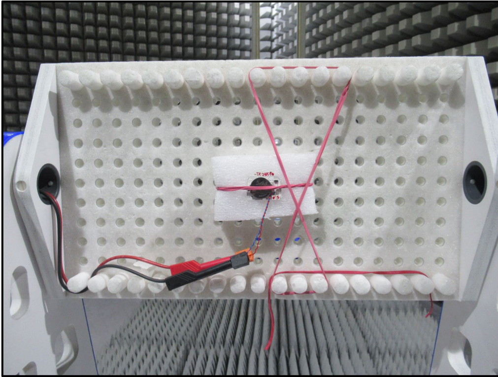
Photo 7: Radiated Test Setup - 1 GHz to 18 GHz – Close view
