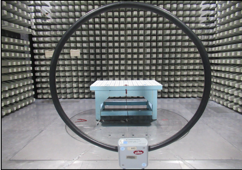
Picture 1: Radiated Test Setup - 9 kHz to 30 MHz
