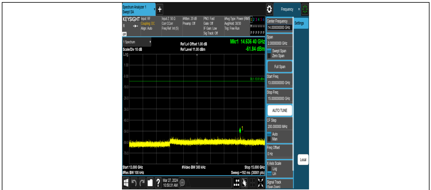
ZIGB-Ant1-2440-13000~15000-PASS
