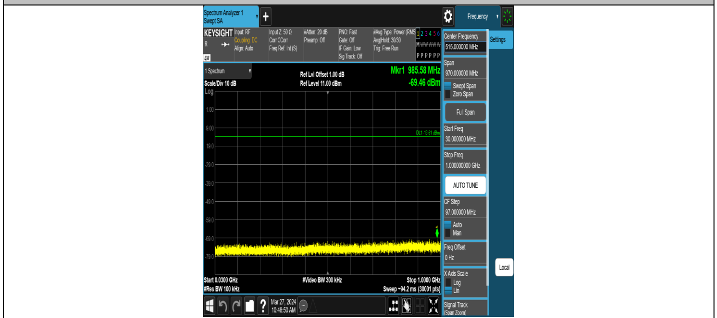
ZIGB-Ant1-2440-30~1000-PASS
