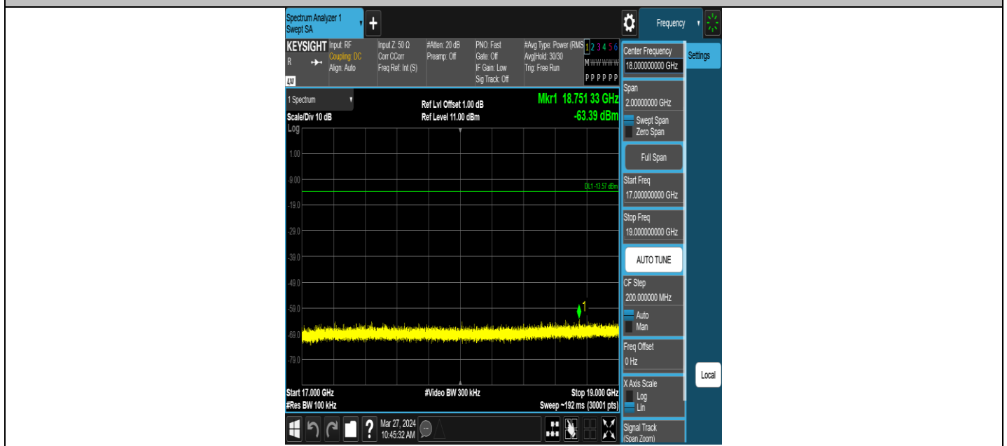
ZIGB-Ant1-2405-17000~19000-PASS
