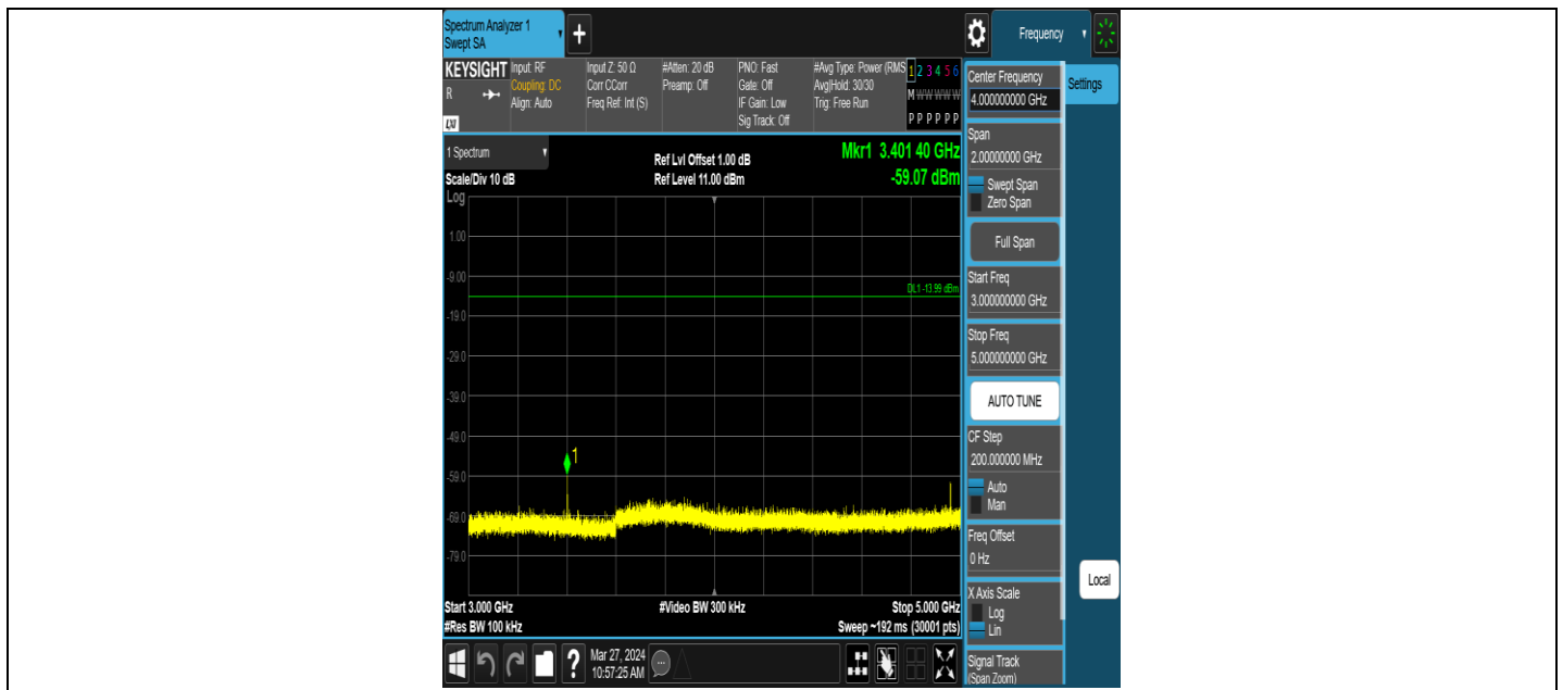
ZIGB-Ant1-2480-3000~5000-PASS
