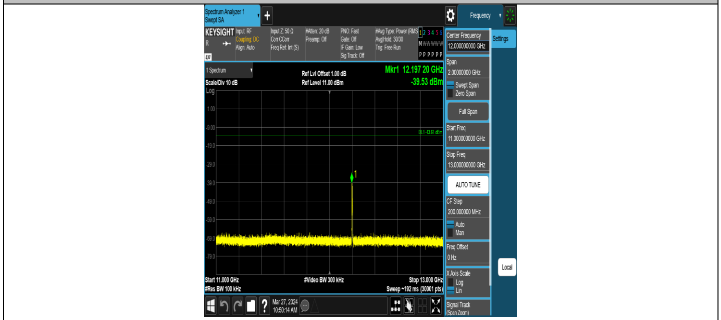
ZIGB-Ant1-2440-11000~13000-PASS
