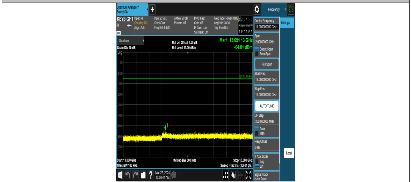
ZIGB-Ant1-2480-13000~15000-PASS
