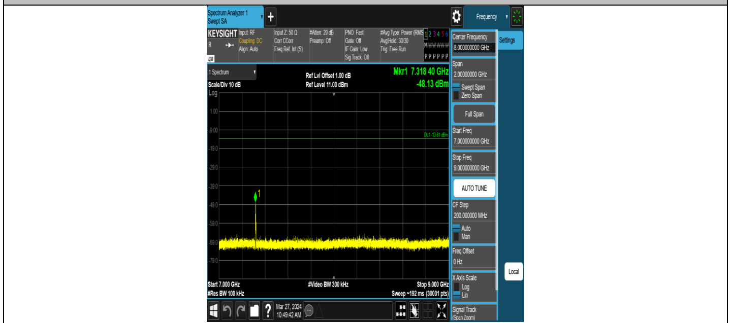
ZIGB-Ant1-2440-7000~9000-PASS
