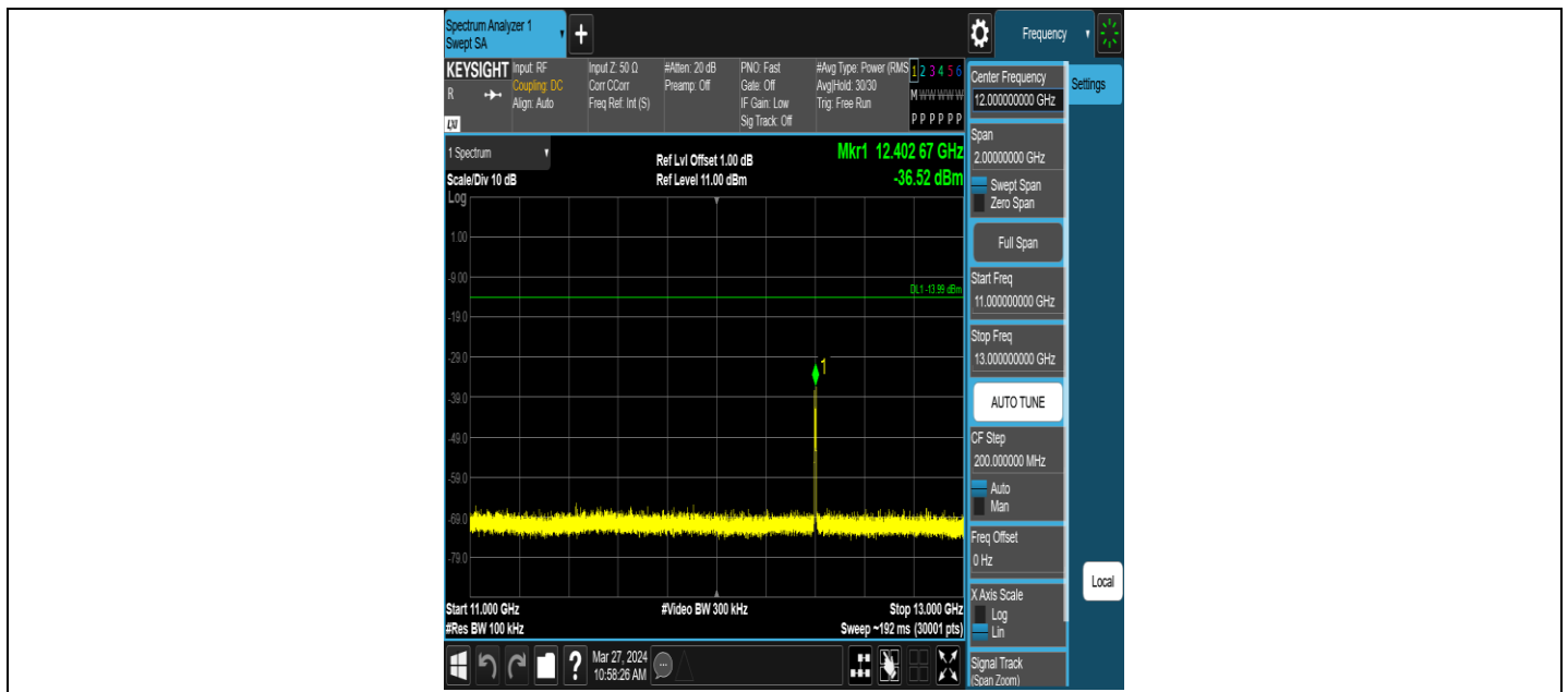
ZIGB-Ant1-2480-11000~13000-PASS
