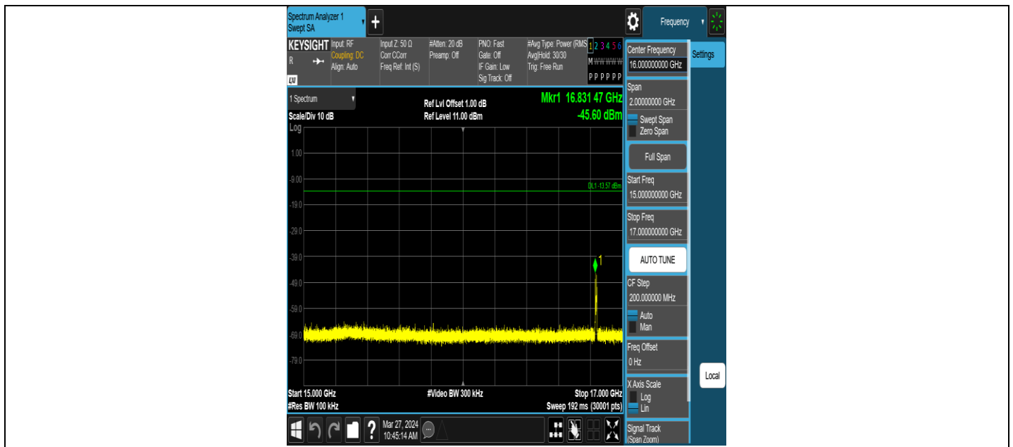
ZIGB-Ant1-2405-15000~17000-PASS
