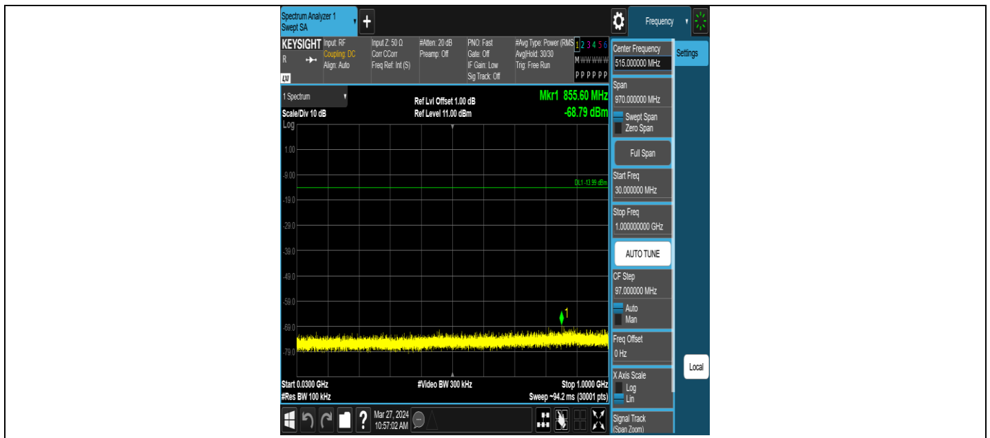
ZIGB-Ant1-2480-30~1000-PASS
