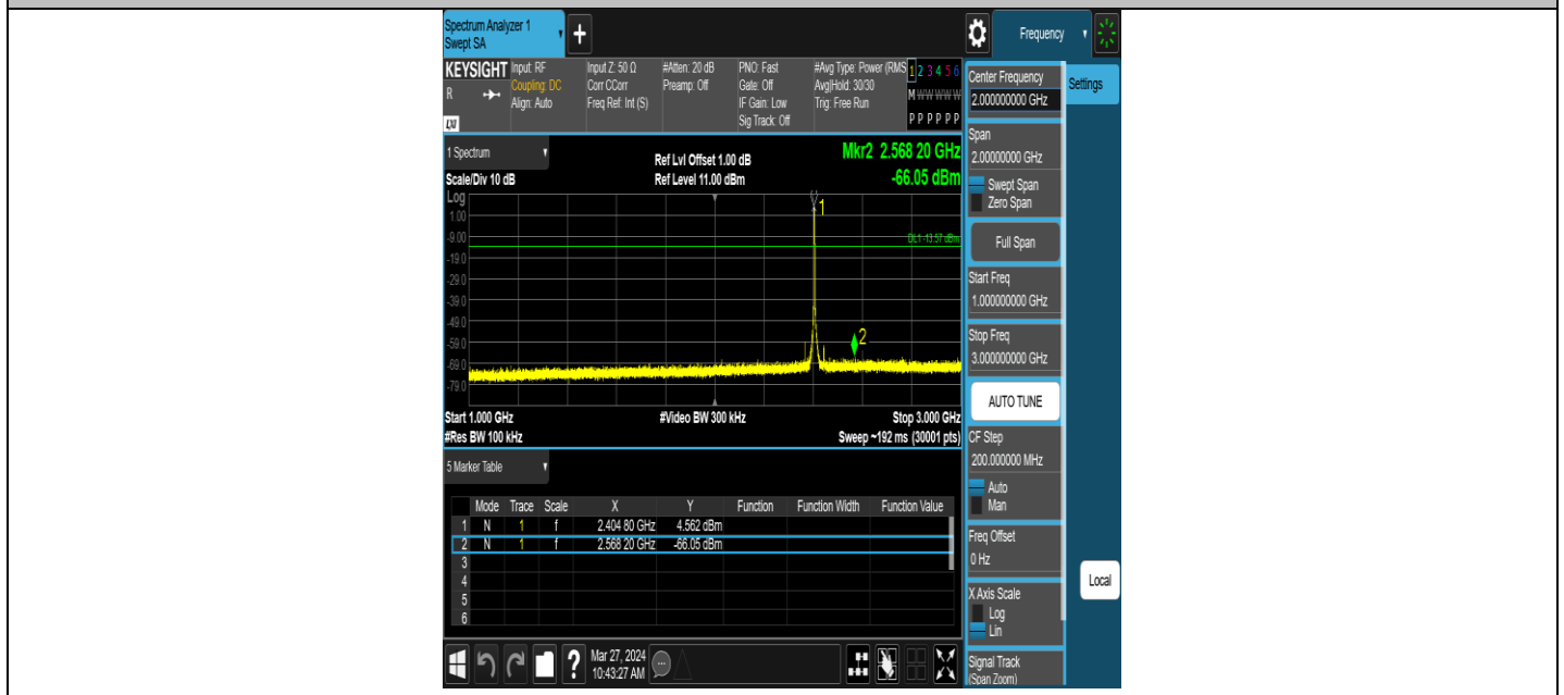
ZIGB-Ant1-2405-1000~3000-PASS
