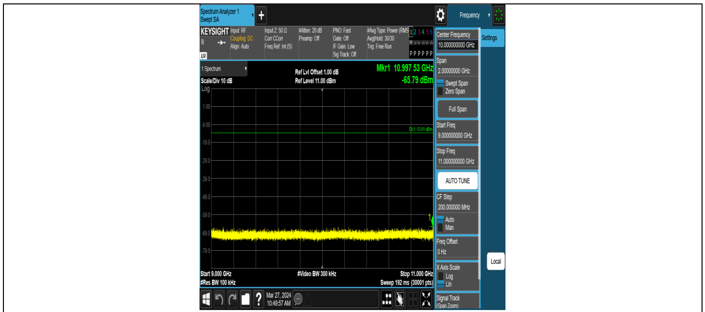
ZIGB-Ant1-2440-9000~11000-PASS
