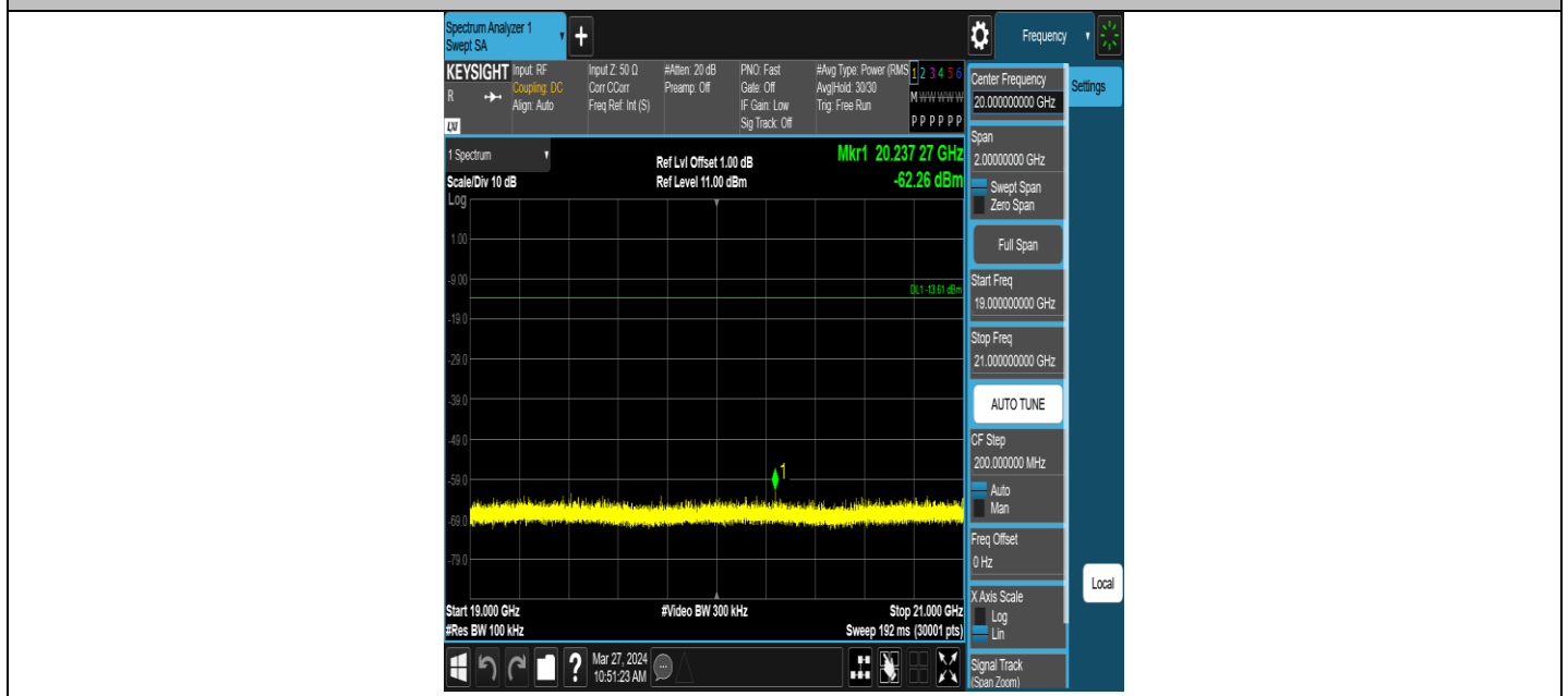
ZIGB-Ant1-2440-19000~21000-PASS
