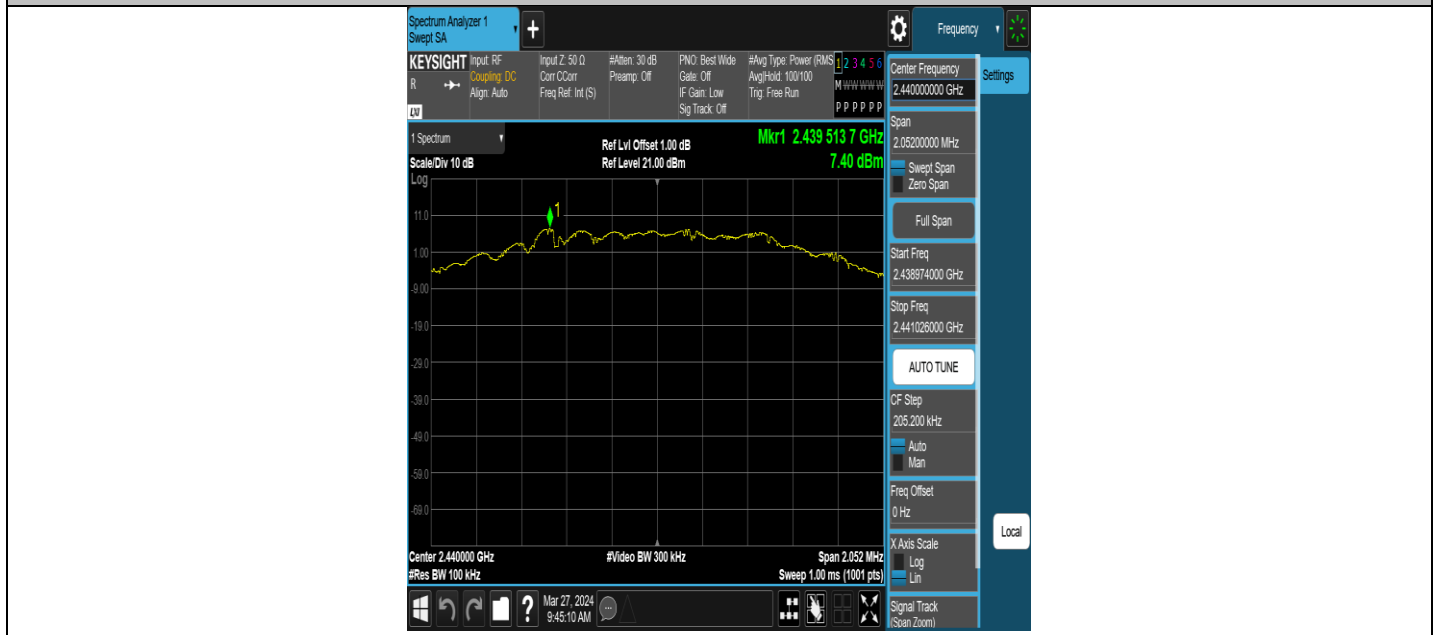
BLE_2M-Ant1-2440-PASS
