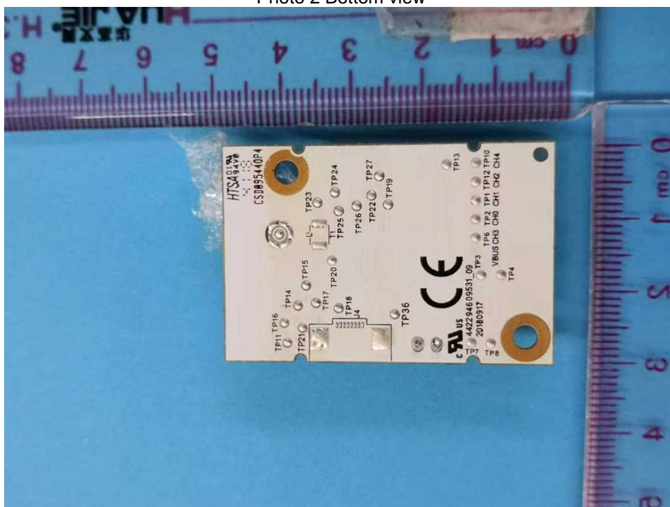
Photo 2 Bottom view
