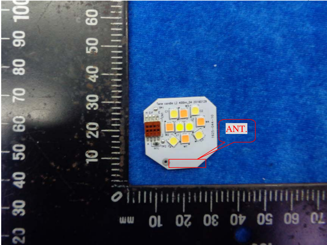
Figure 7 LED Board (Front View)
