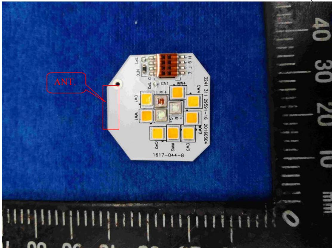
Figure 16 LED Board (Front View)
