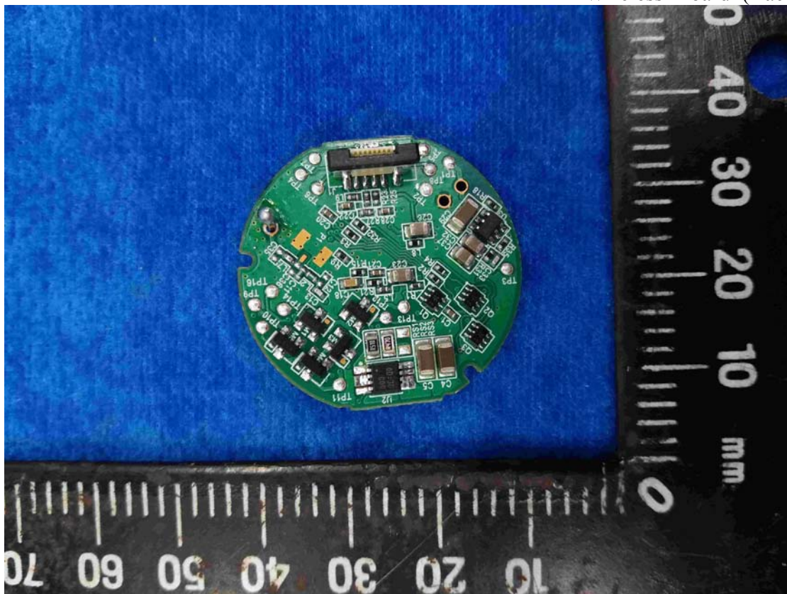
Figure 14 Wireless Board (Back View)
