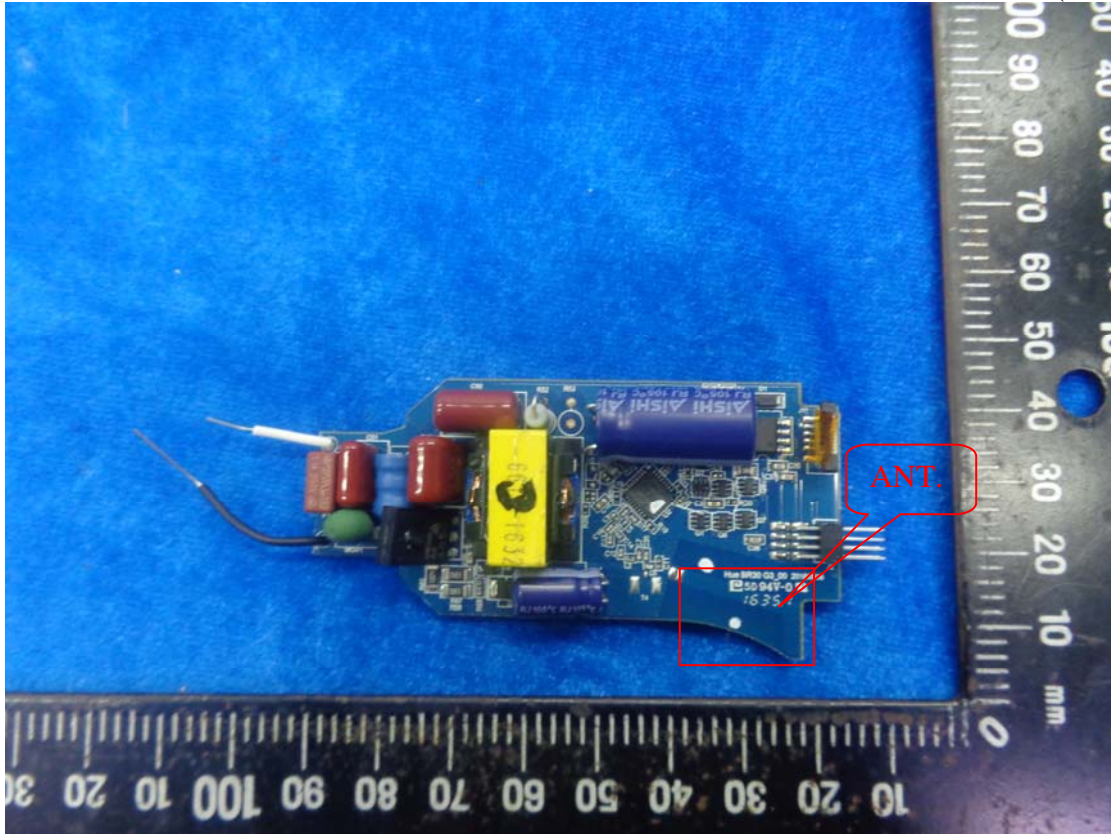
Figure 9 Power Board (Front View)
