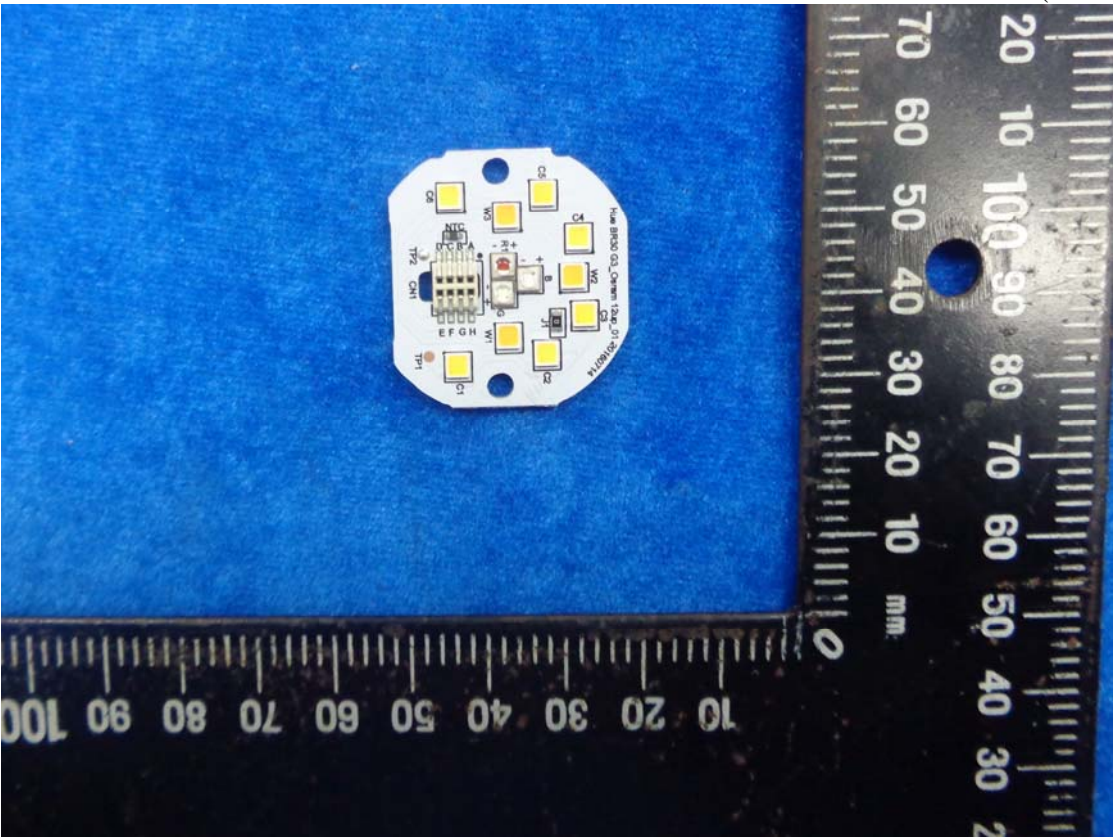
Figure 4 LED Board (Front View)
