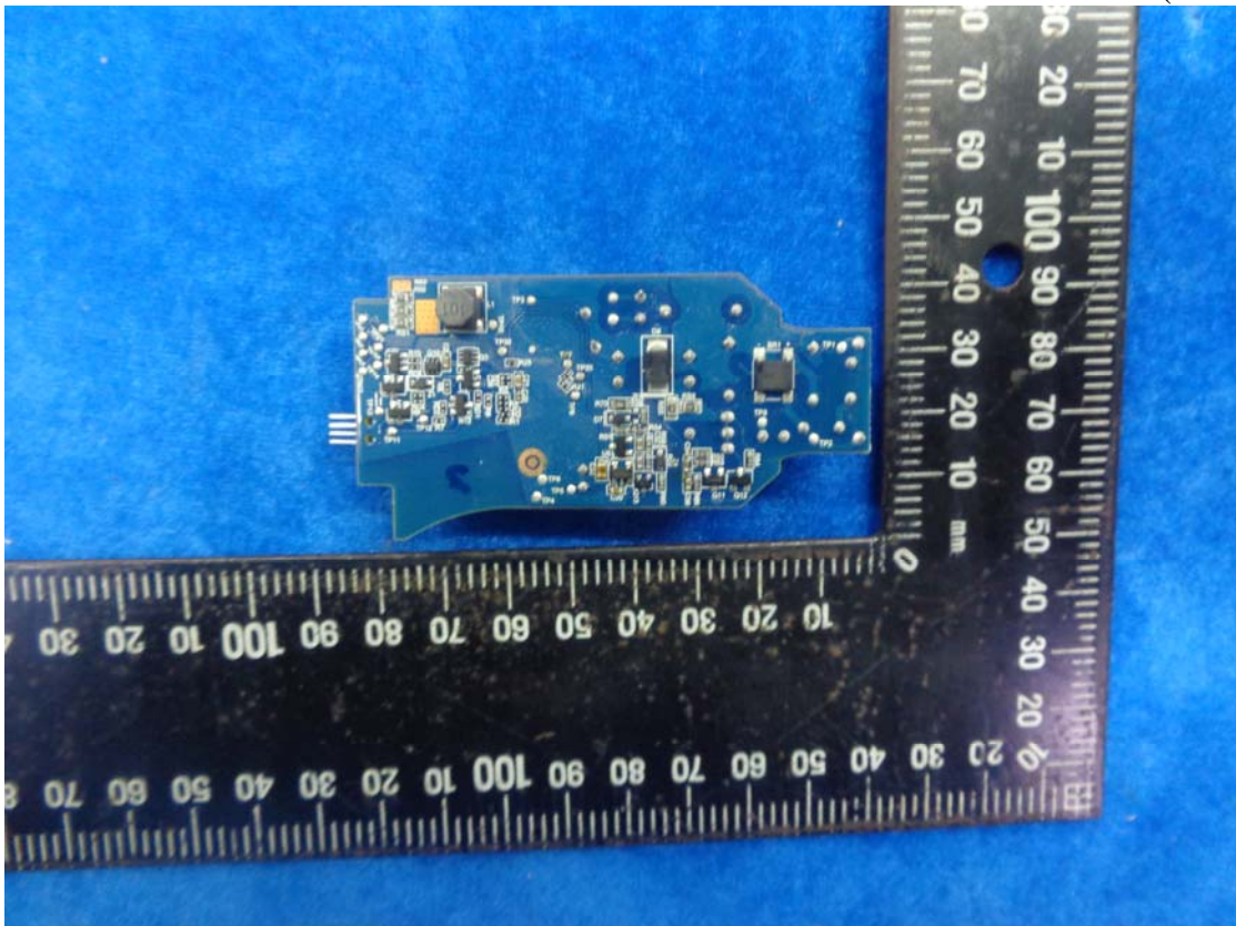
Figure 10 Power Board (Back View)
