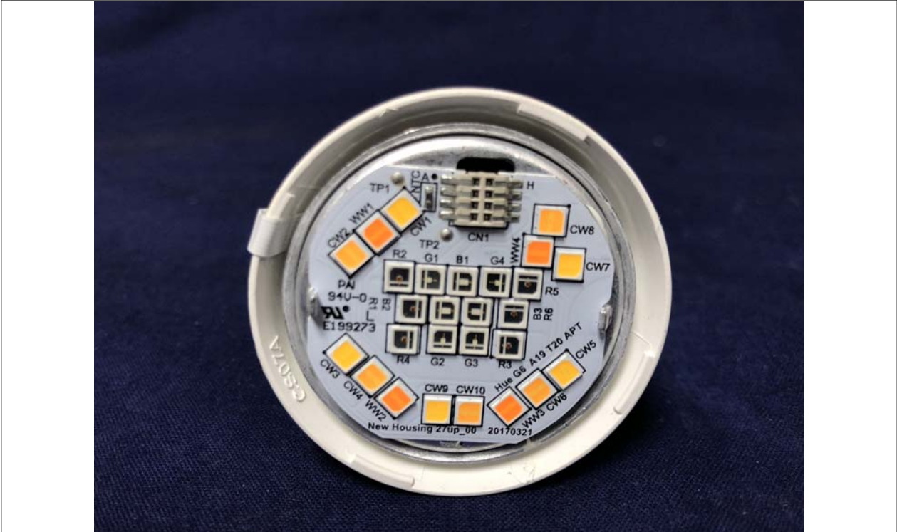
(15) EUT Photo(APT+Alvis+Murata)
