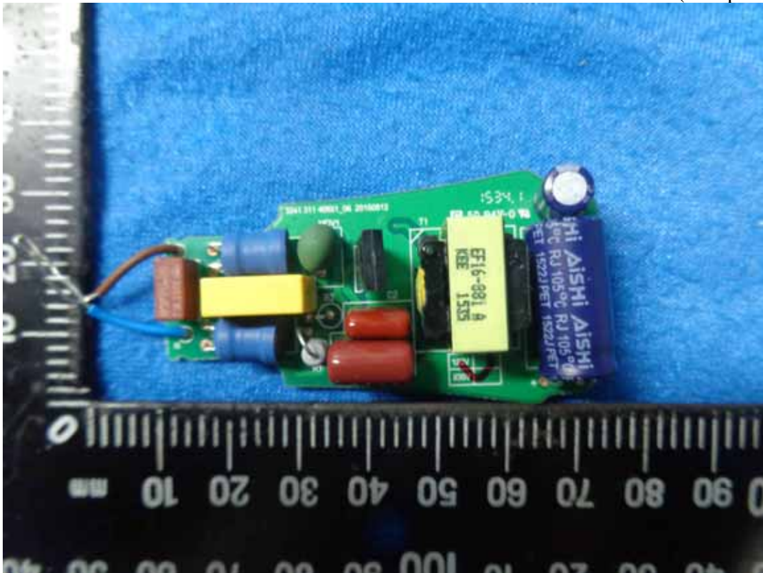
Figure 8 Power Board (Component Side)
