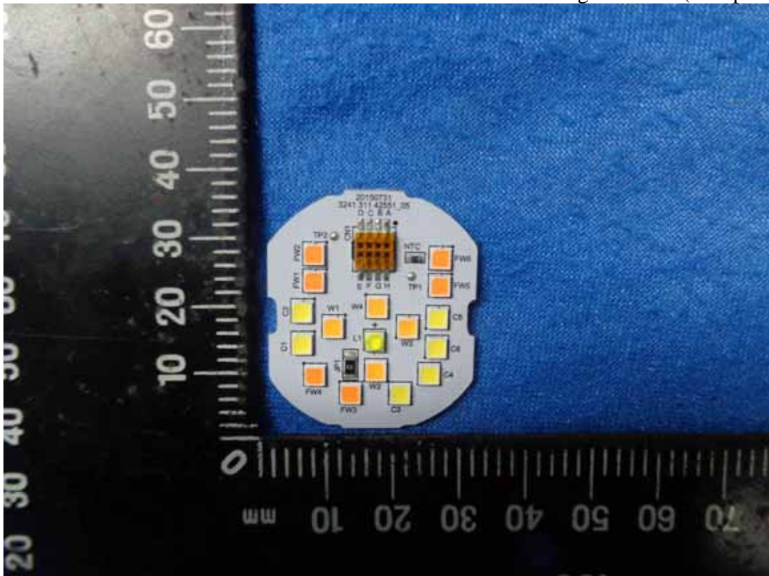
Figure 6 LED Light Board (Component Side)
