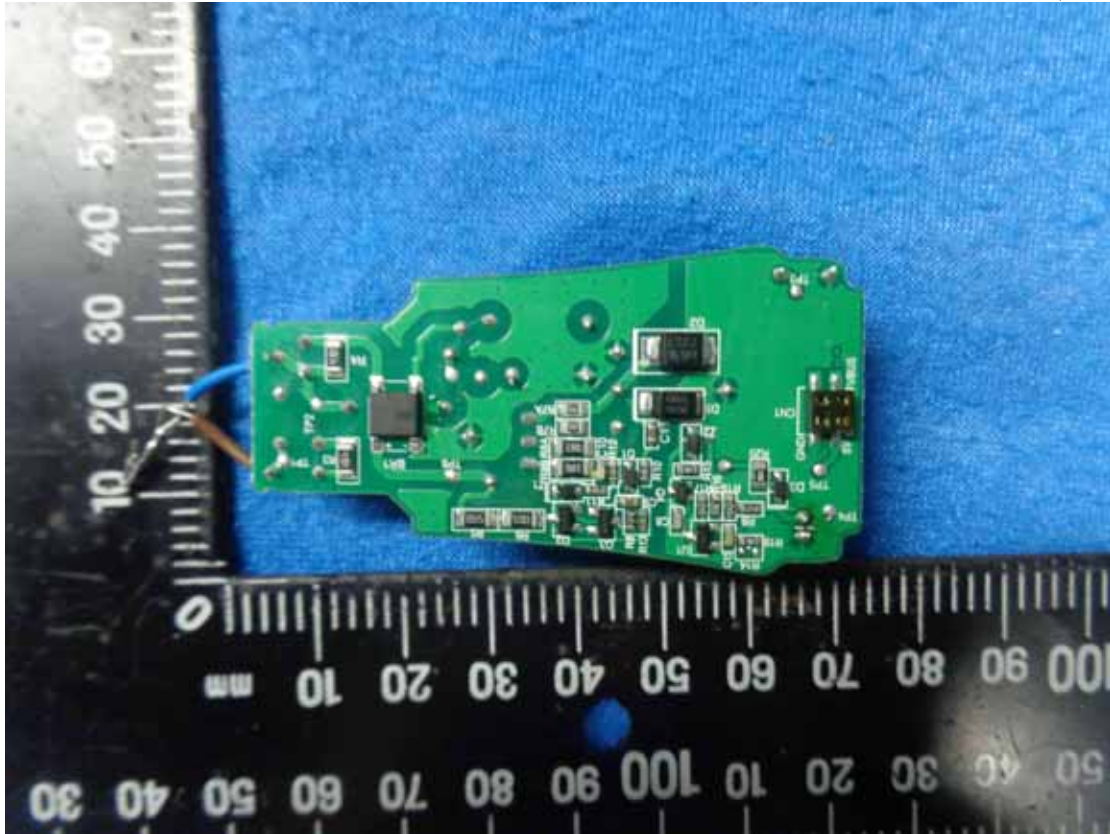
Figure 9 Power Board (Solder Side)
