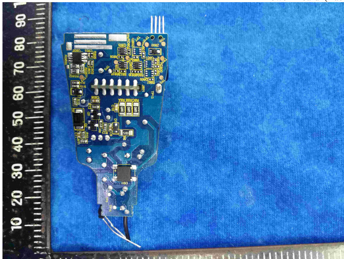
Figure 6 Power Board (Back View)
