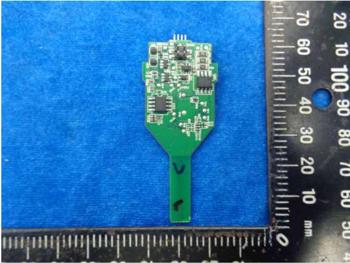
Figure 9 Wireless Board (Back View)
