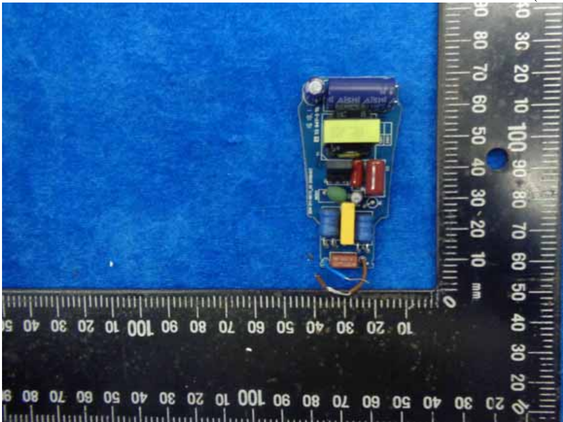
Figure 6 Power Board (Front View)
