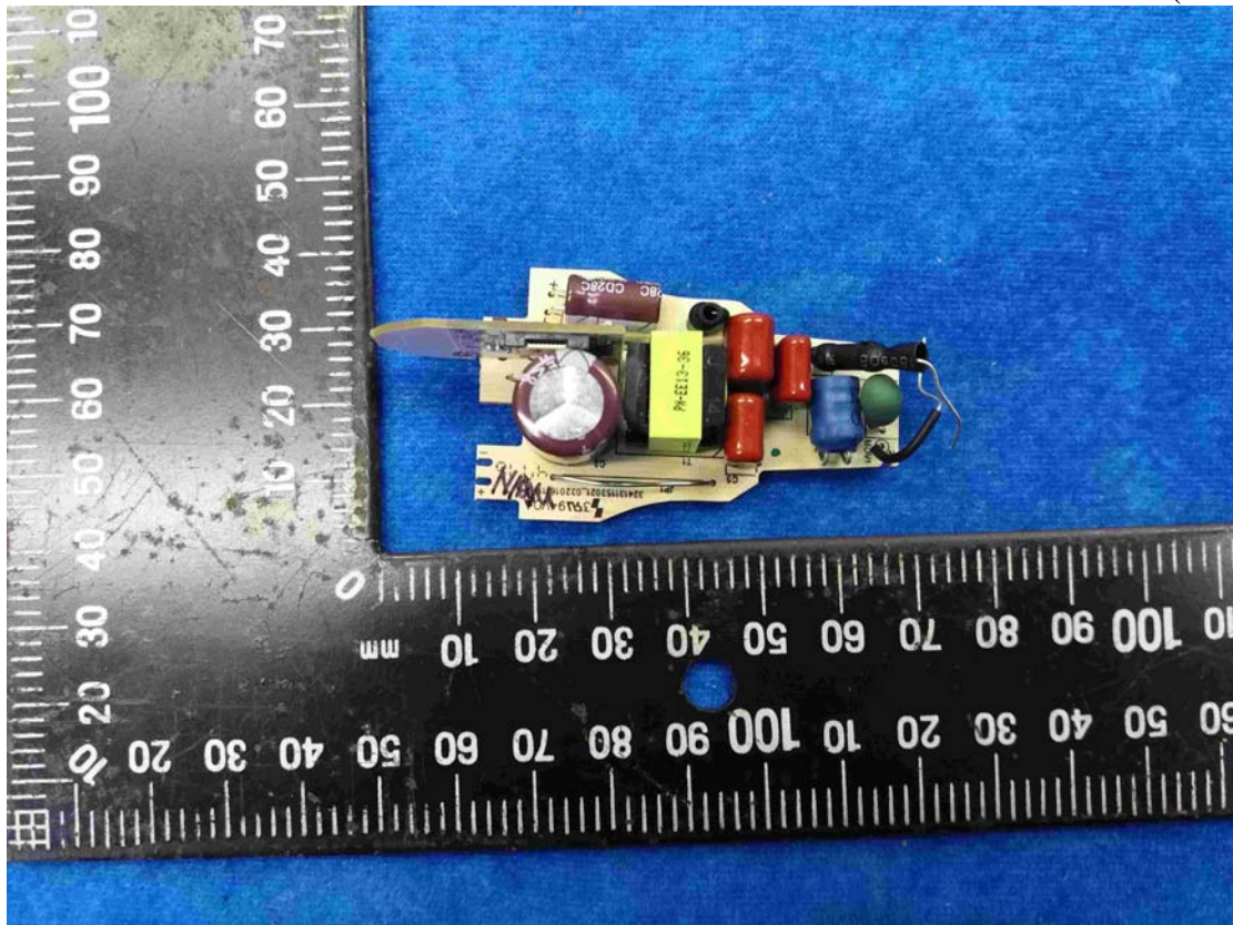
Figure 8 Power Board (Front View)
