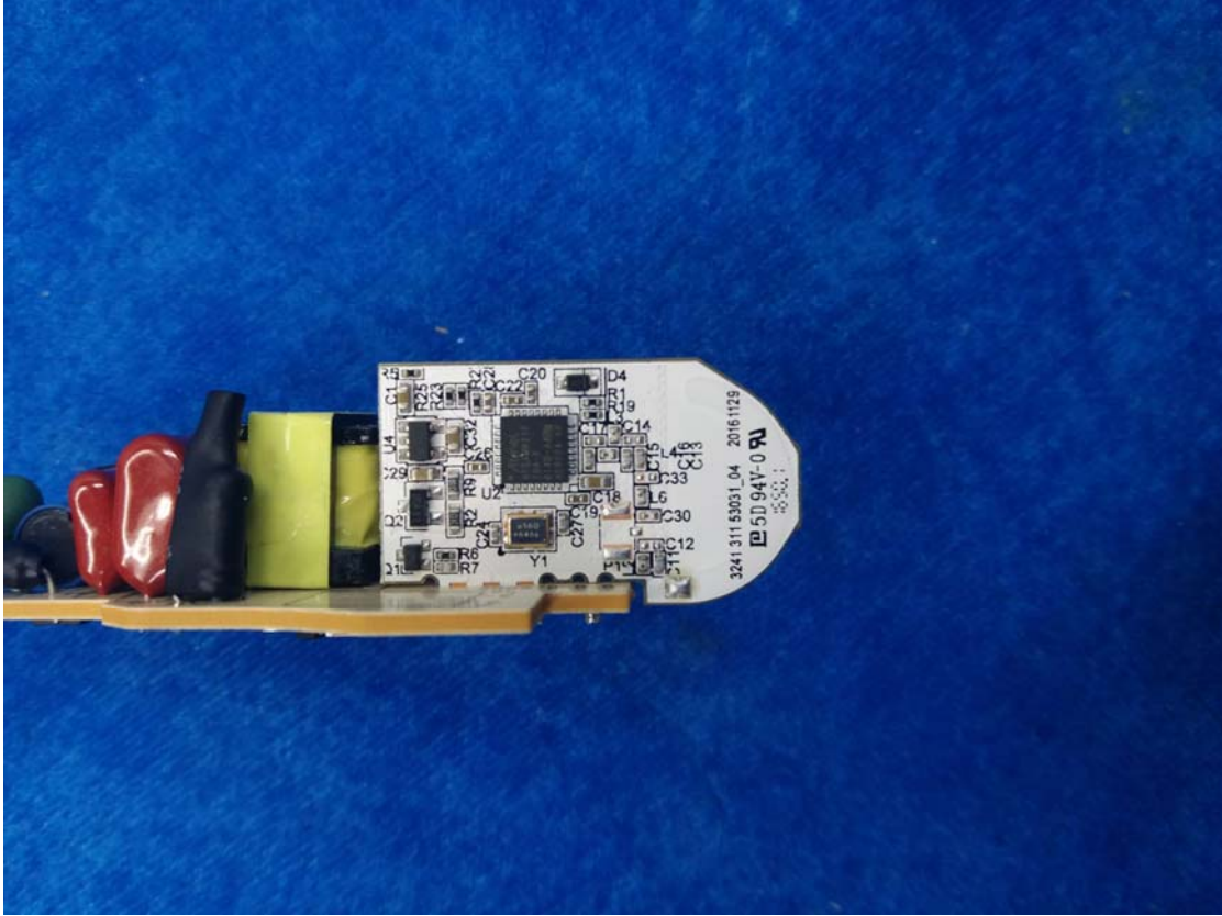
Figure 11 Wireless Board (Front View)
