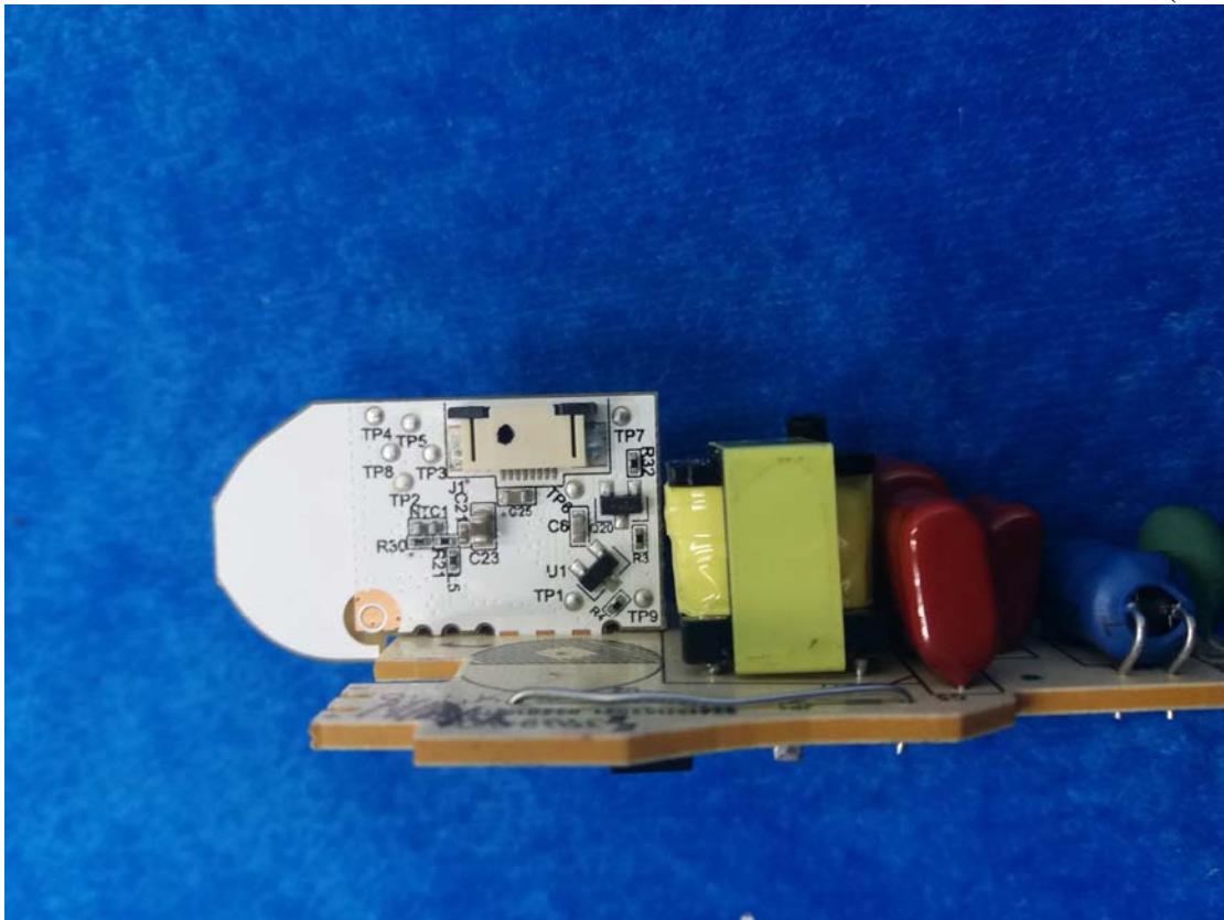
Figure 12 Wireless Board (Back View)
