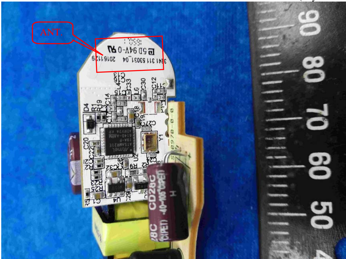
Figure 10 Wireless Board (Crystal Oscillator)
