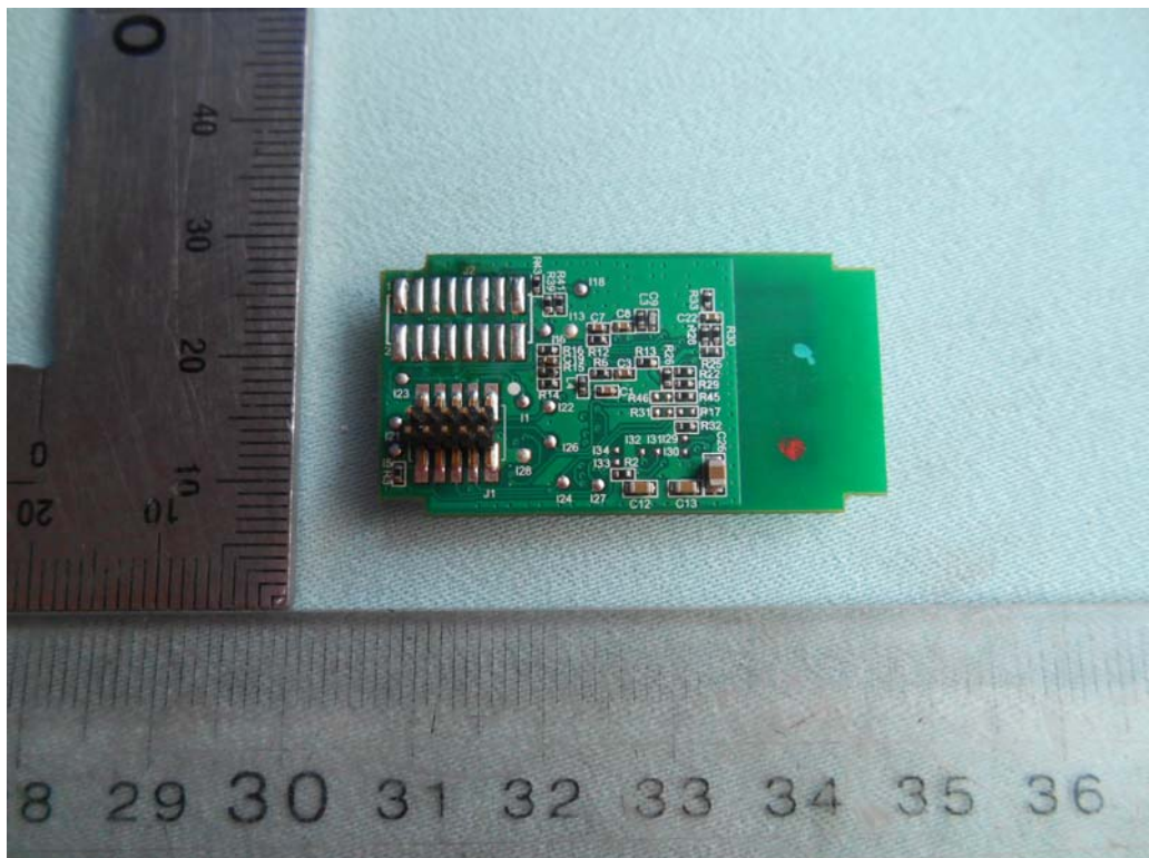
FIGURE 2 WIRELESS CONTROL BOARD (M/N: 324131296121) GENERAL APPEARANCE (BACK VIEW)
