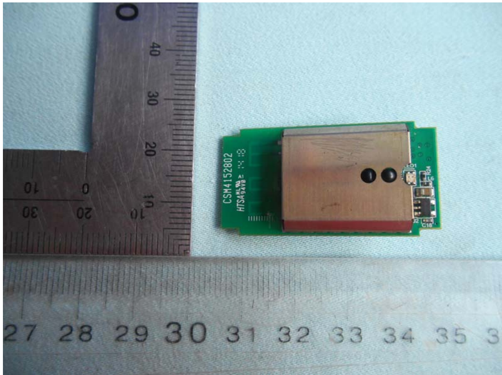
FIGURE 1 WIRELESS CONTROL BOARD (M/N: 324131296121) GENERAL APPEARANCE (FRONT VIEW)
