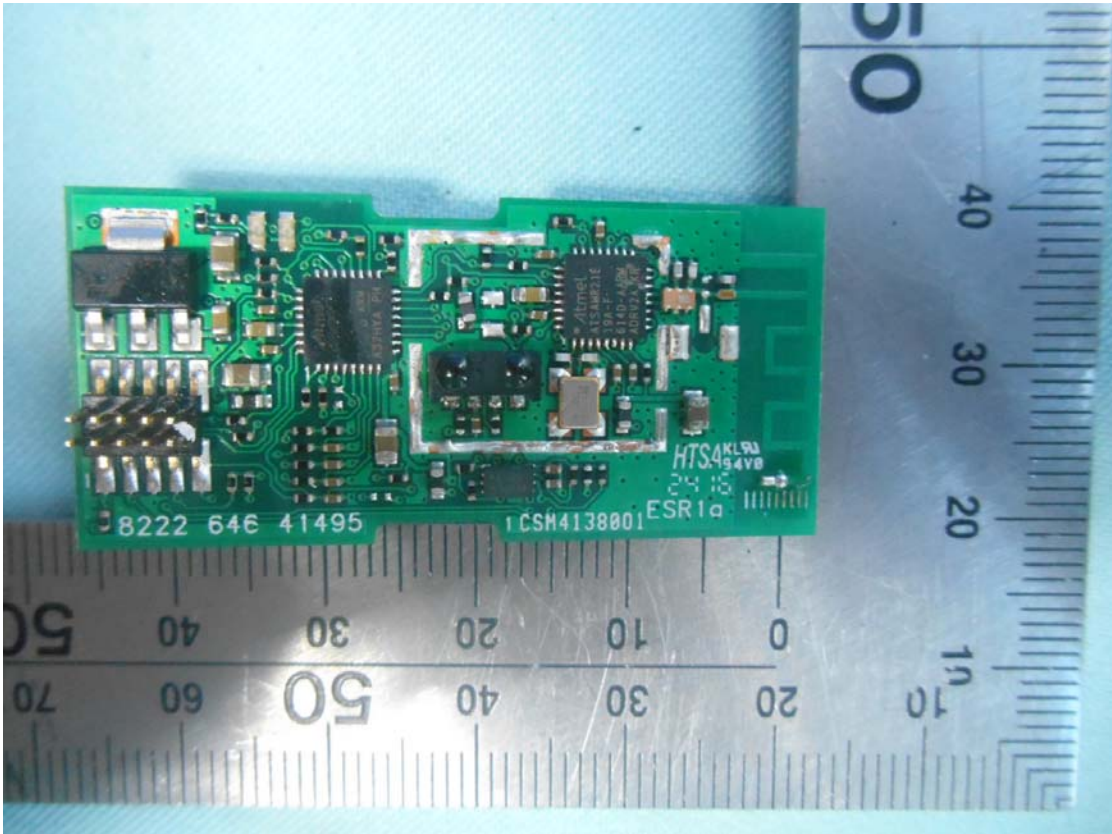
FIGURE 3 LED MODULE (M/N: HUE ENGINE V1.0) SHIELD REMOVED
