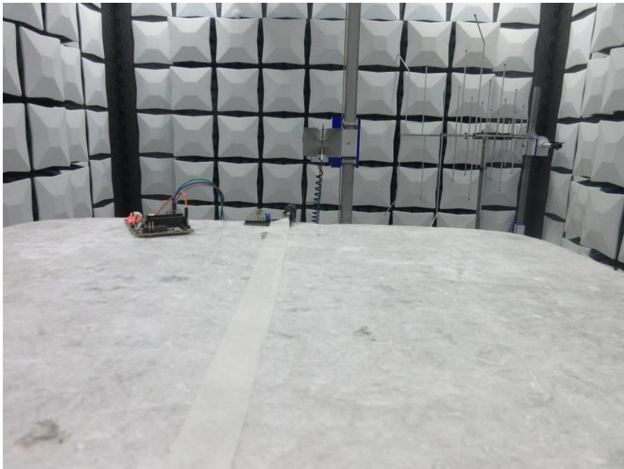
RADIATED RF MEASUREMENT SETUP (CLOSE SHOT)
