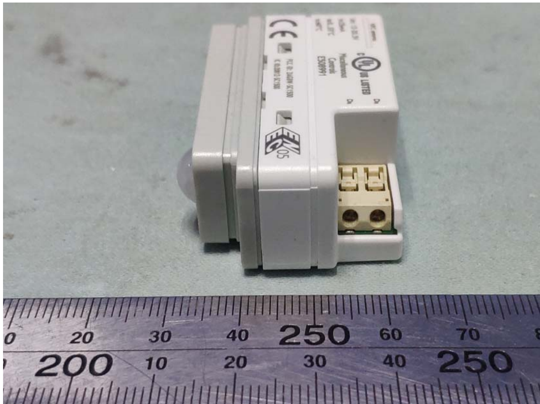
FIGURE 11 MISCELLANEOUS CONTROLS (M/N: SC1500/10) GENERAL APPEARANCE (RIGHT VIEW)
