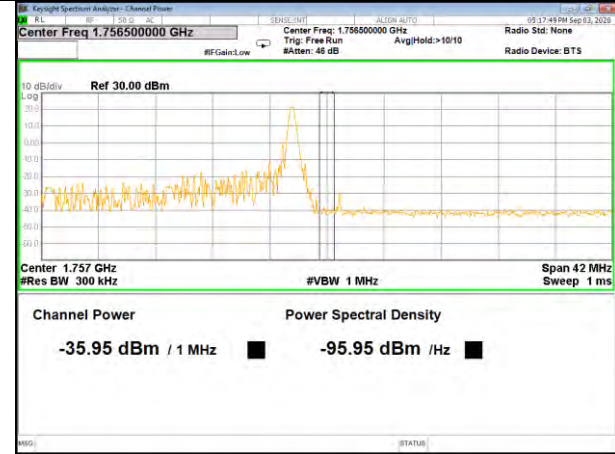
Band4_20M_QPSK_High_Full-RB
