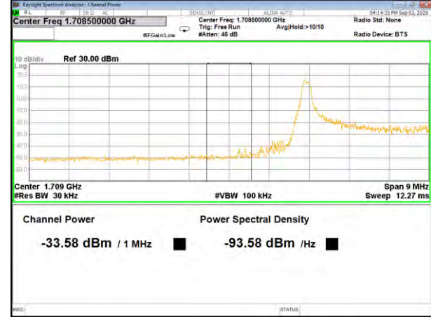
Band4_3M_16QAM_Low_Full-RB
