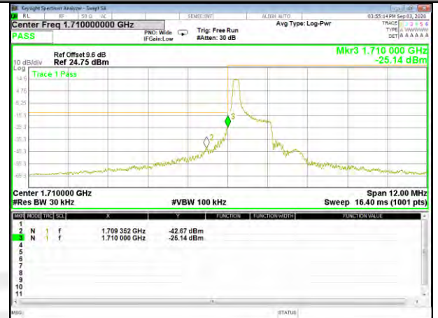
Band4_1.4M_QPSK_Low_Full-RB
