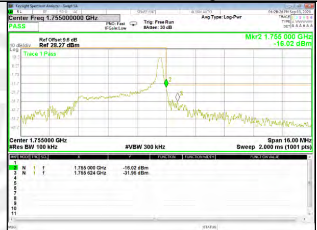
Band4_5M_16QAM_High_Full-RB
