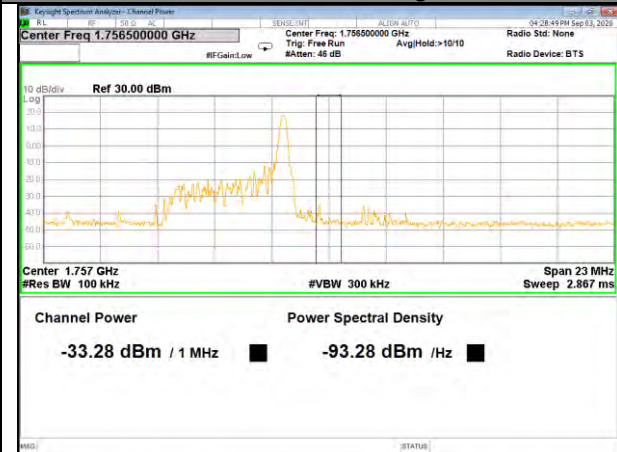
Band4_5M_16QAM_High_Full-RB
