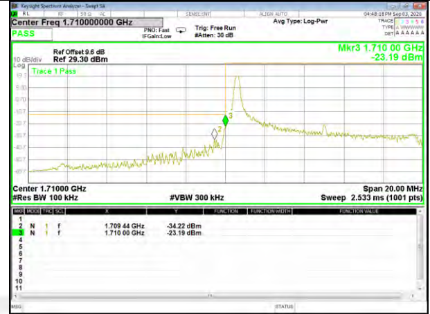
Band4_10M_QPSK_Low_Full-RB
