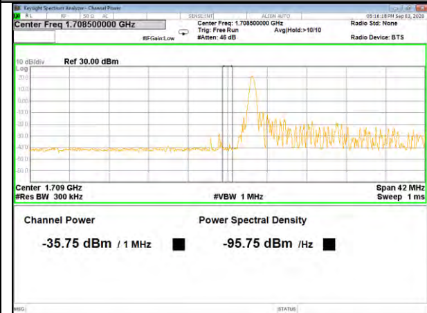
Band4_20M_QPSK_Low_Full-RB
