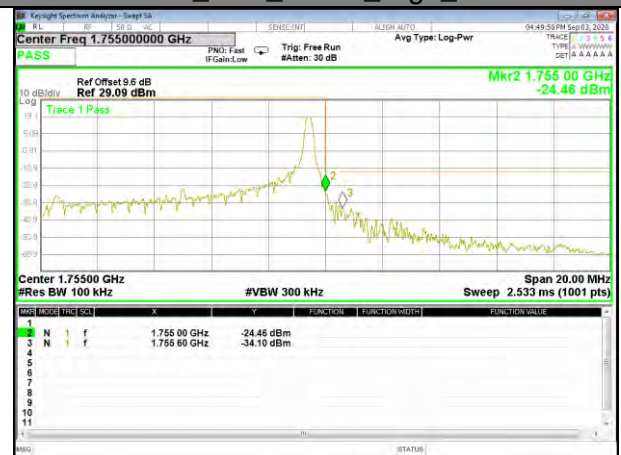
Band4_10M_QPSK_High_1-RB
