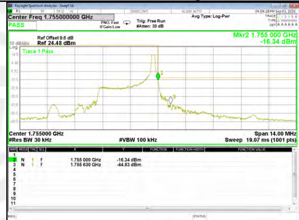
Band4_3M_QPSK_High_Full-RB
