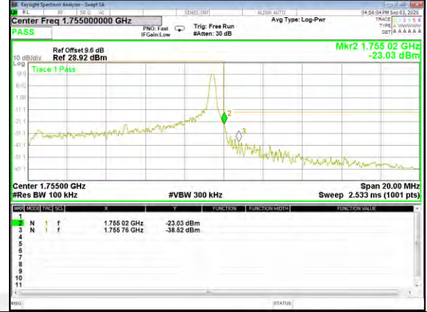
Band4_10M_16QAM_High_Full-RB
