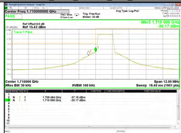
Band4_1.4M_16QAM_Low_Full-RB
