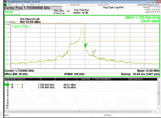
Band4_1.4M_16QAM_High_Full-RB
