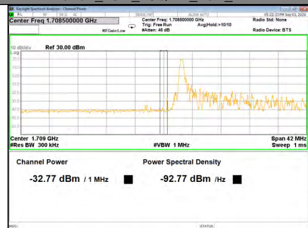
Band4_20M_16QAM_Low_1-RB
