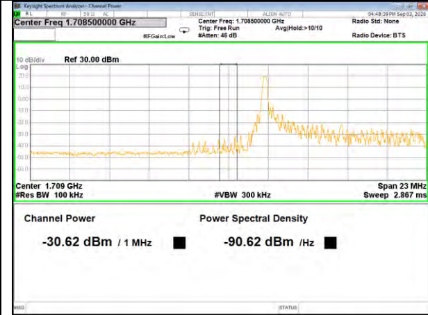
Band4_10M_QPSK_Low_Full-RB
