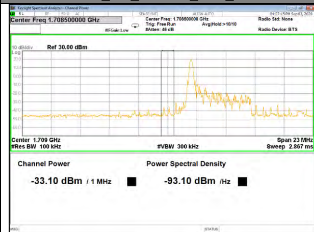
Band4_5M_16QAM_Low_1-RB
