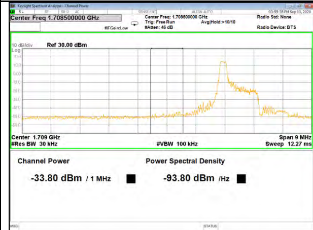
Band4_1.4M_QPSK_Low_Full-RB
