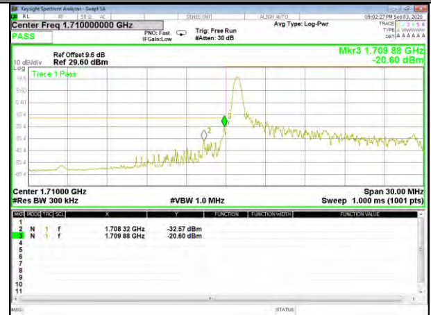
Band4_15M_QPSK_Low_1-RB
