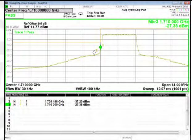
Band4_3M_16QAM_High_1-RB
