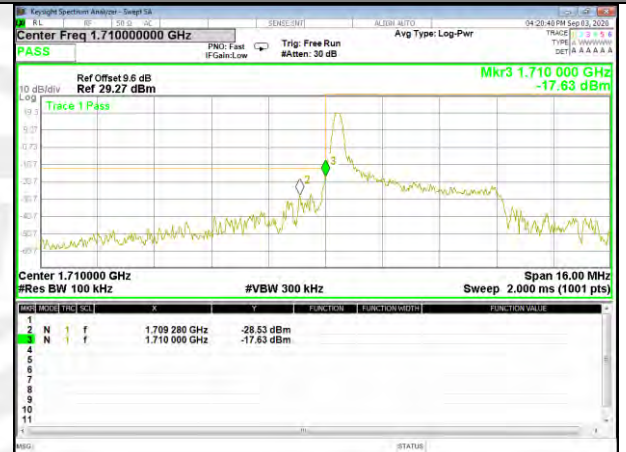
Band4_5M_QPSK_Low_Full-RB
