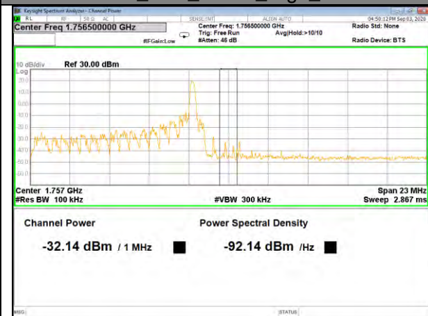
Band4_10M_QPSK_High_1-RB
