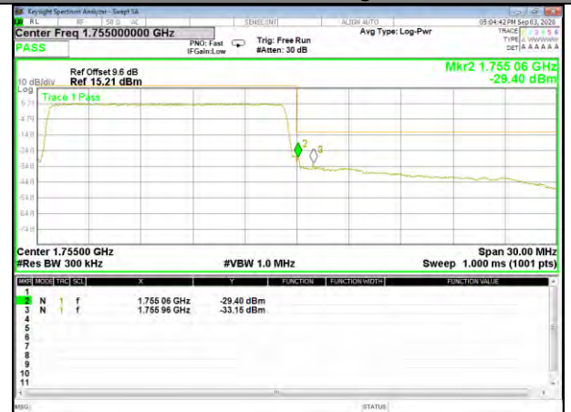
Band4_15M_QPSK_High_Full-RB
