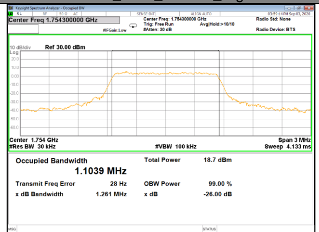
Band4_1.4M_16QAM_High
