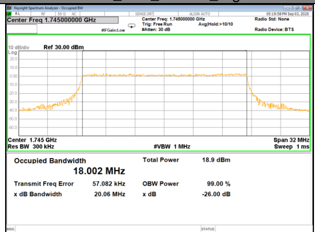
Band4_20M_16QAM_High
