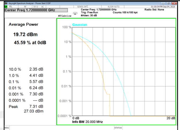
Band4_100_Q16_Low
