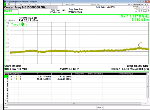
Band4_15M_16QAM_Middle
