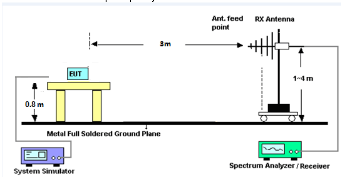
(A) Radiated Emission Test-Up Frequency 30MHz~1GHz
