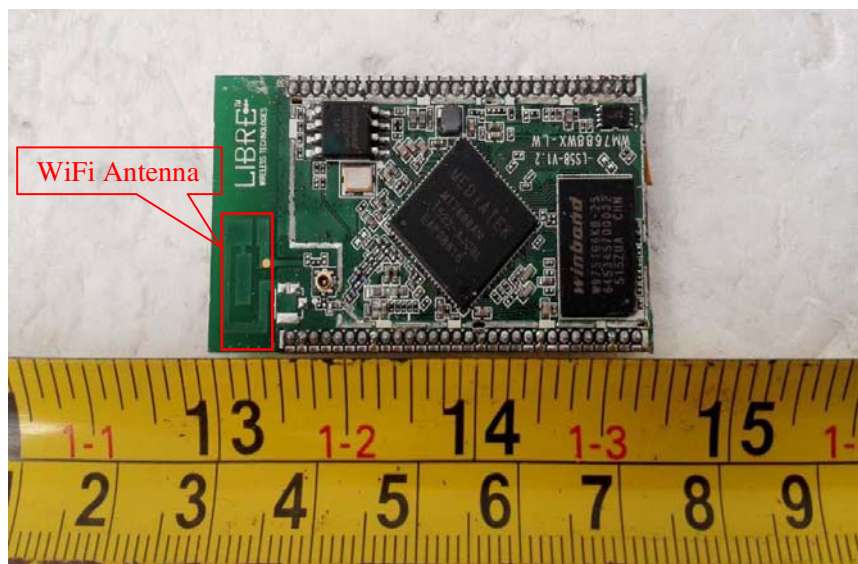
EUT – Main Board-1 Rear View
