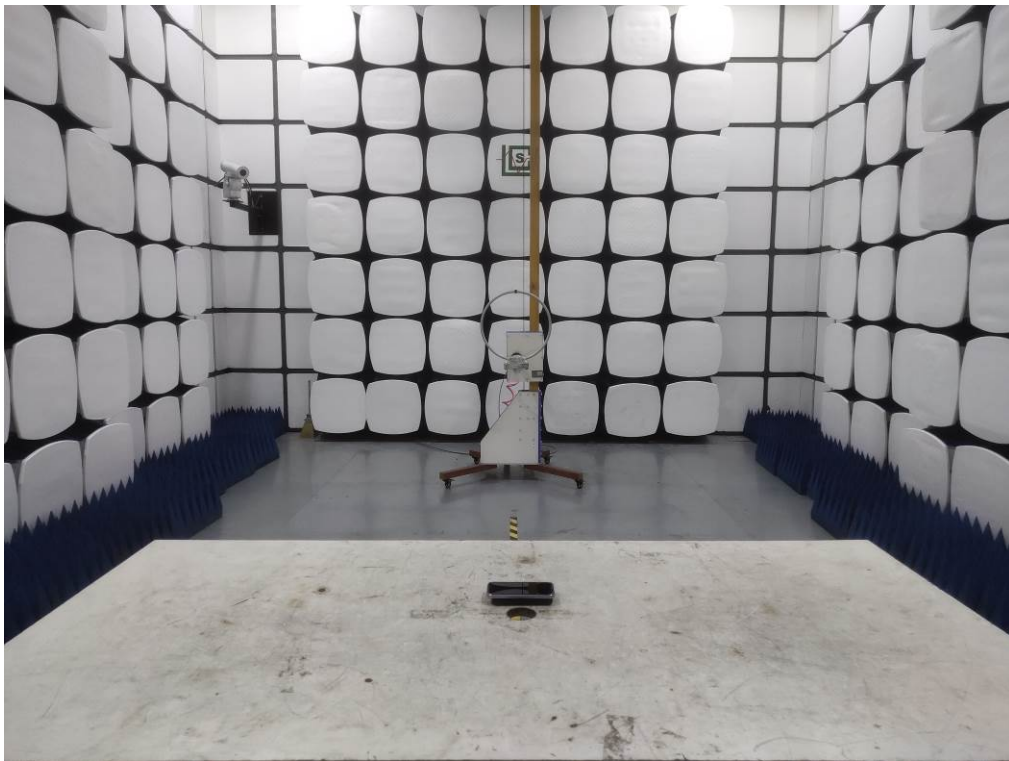
Radiated Emission below 30MHz-DC adapter charge mode
