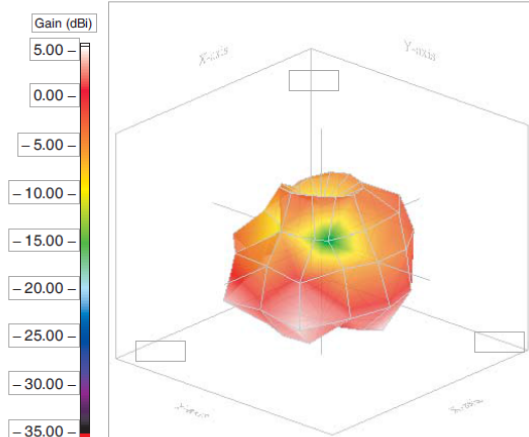
Max gain = -2 dBi, at (150,150) MEG
