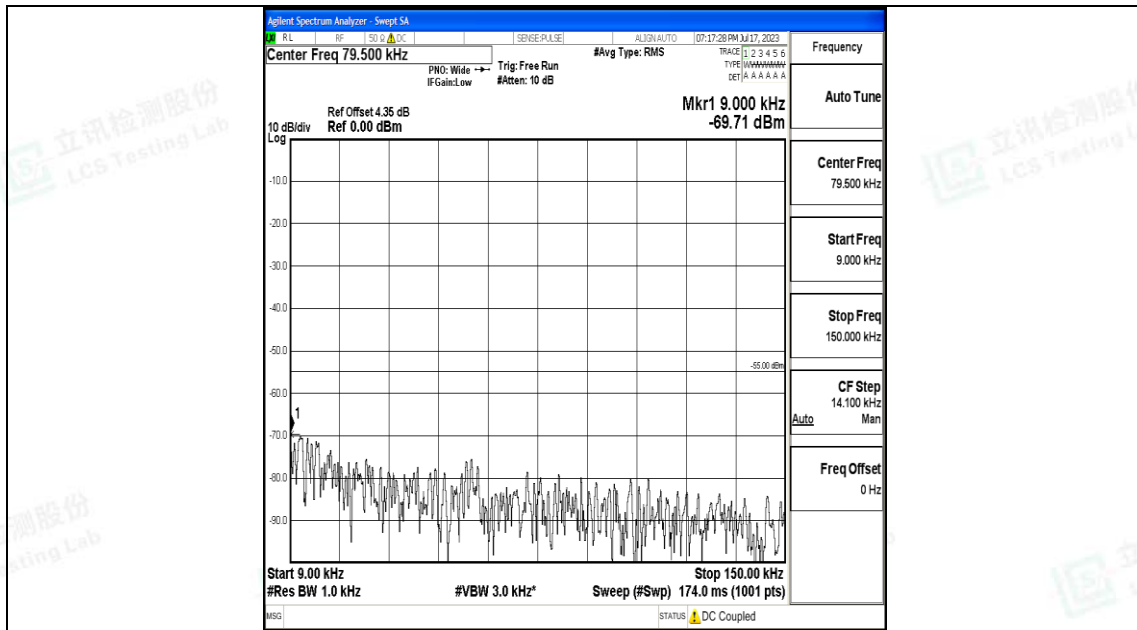
Band7_5MHz_16QAM_20775_1RB#0_0.009~0.15_0.009~0.15
