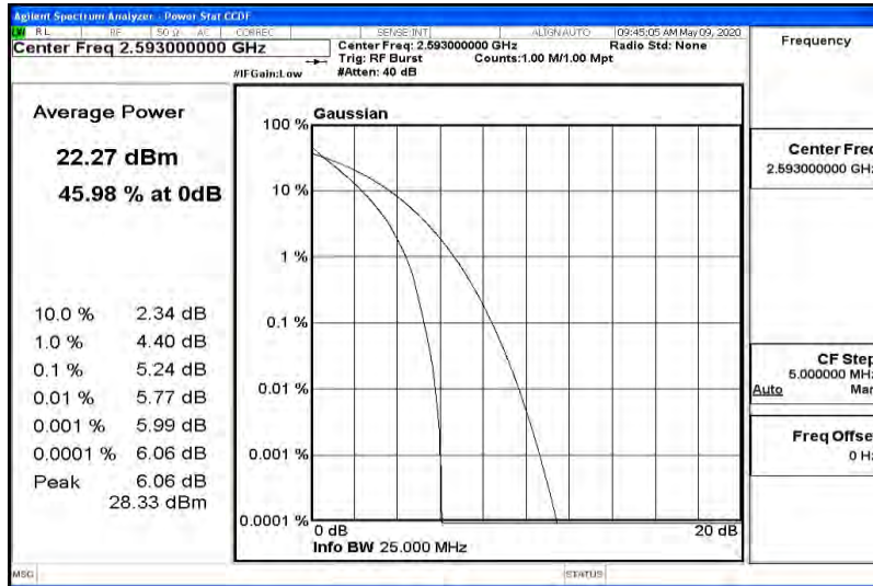
Band41-10MHz-QPSK-41540-1RB#0
