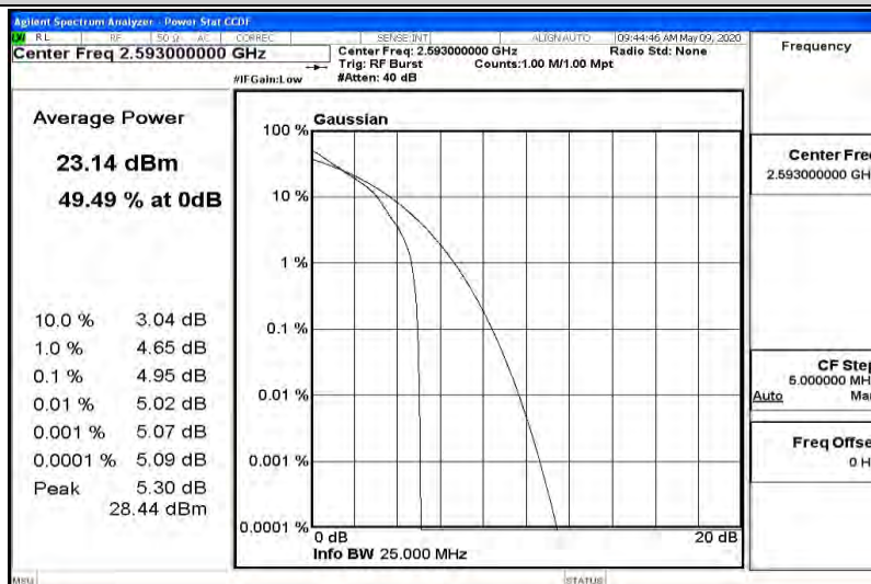
Band41-10MHz-QPSK-40620-50RB#0
