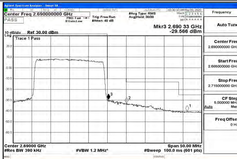
Band41-20MHz-16QAM-39750-100RB#0
