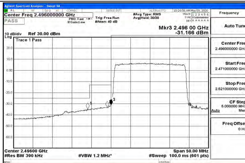
Band41-20MHz-16QAM-41490-100RB#0
