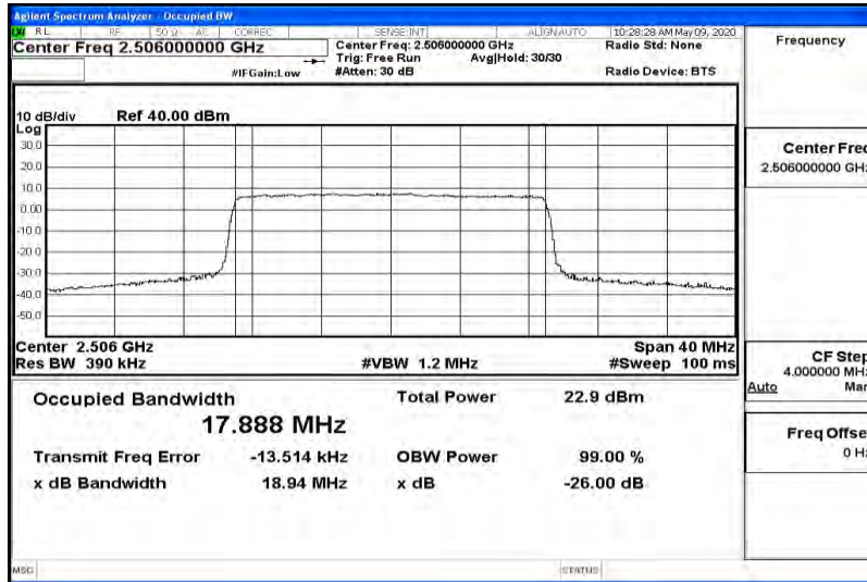
Band41-20MHz-QPSK-40620-100RB#0-17.888
