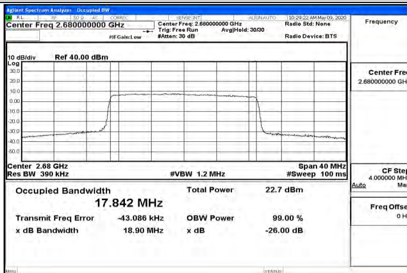
Band41-20MHz-16QAM-41490-100RB#0-17.842
