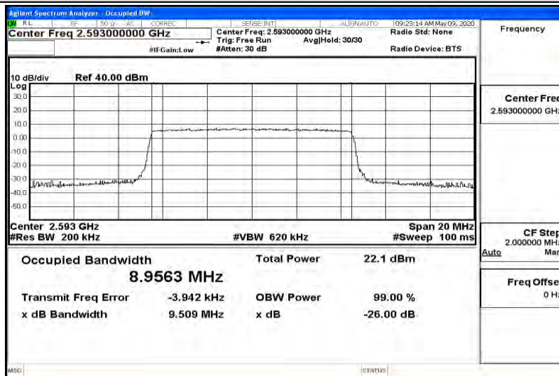
Band41-10MHz-16QAM-41540-50RB#0-8.9565
