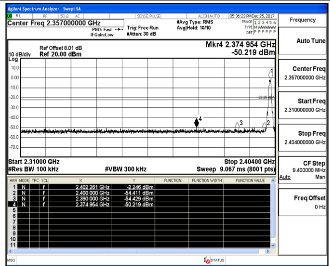
Channel 0 / 2402 MHz
