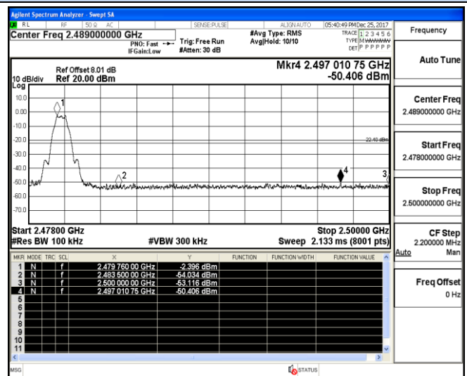
Channel 39 / 2480 MHz
