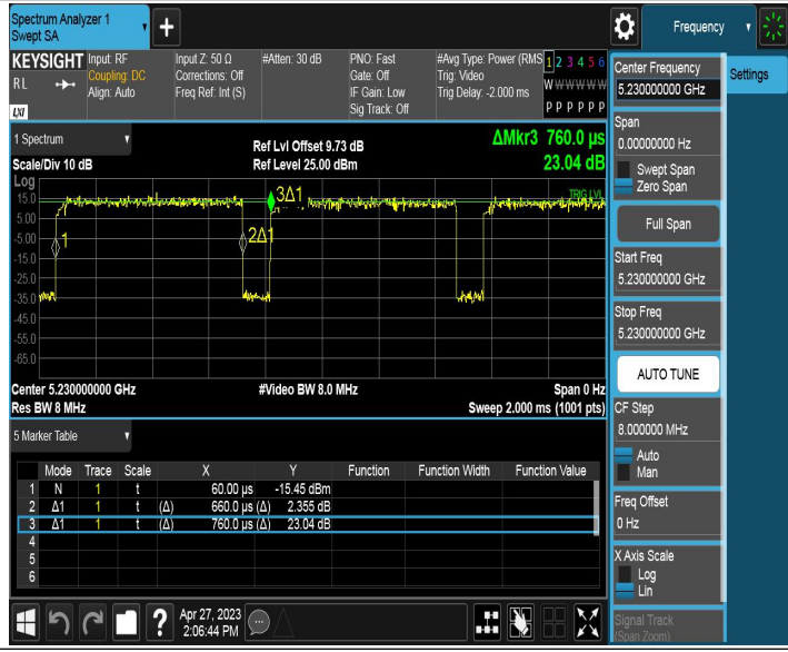
11AC40SISO_Ant2_5230
