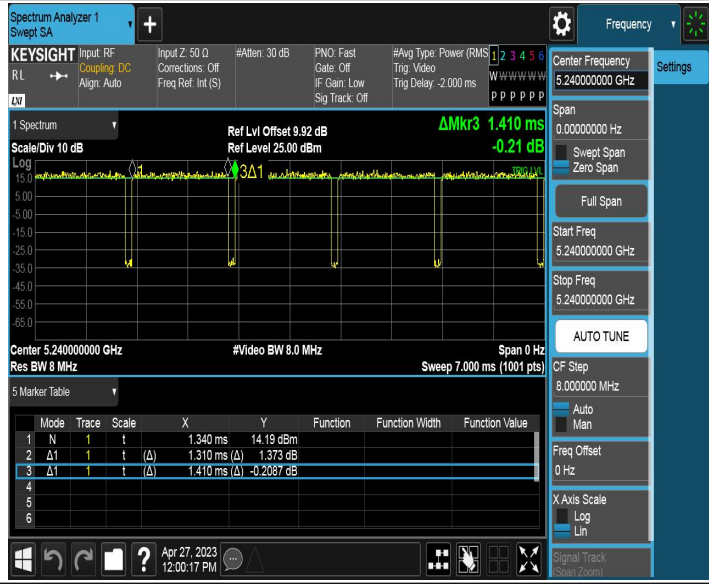
11AC20SISO_Ant2_5240
